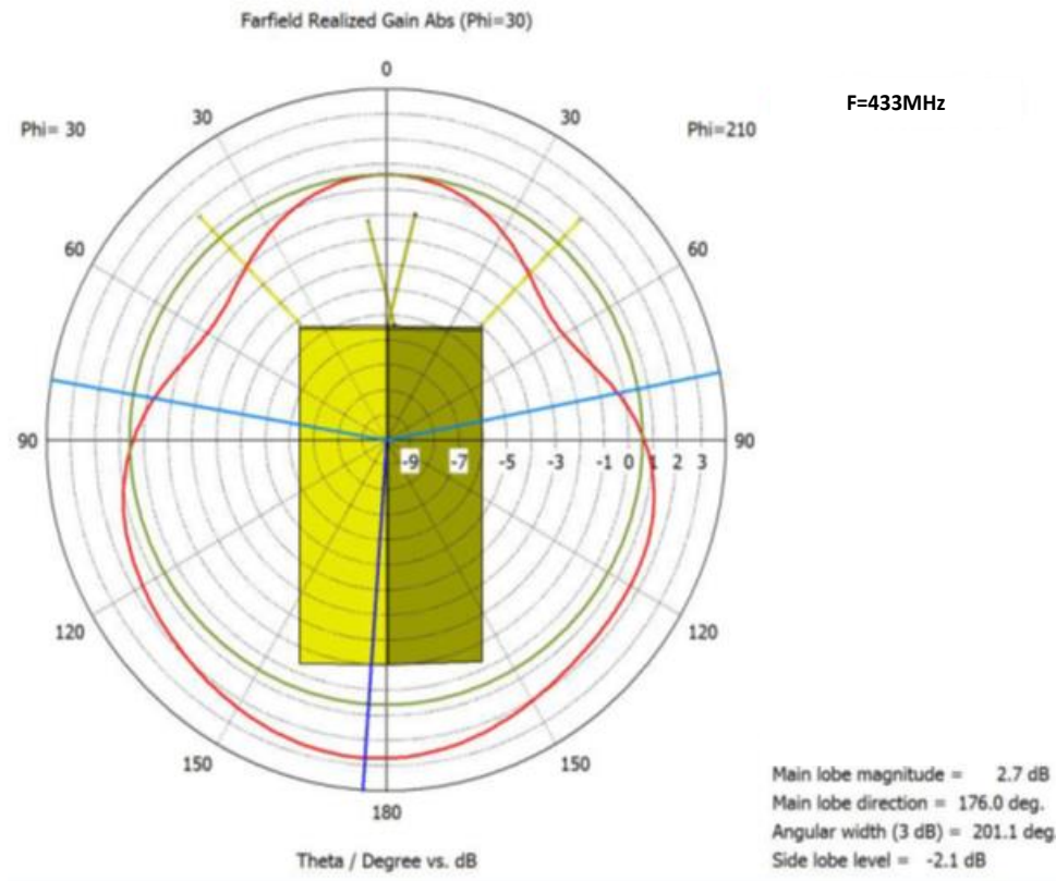
Figure 2 UHF Monopole TX Antenna Pattern
