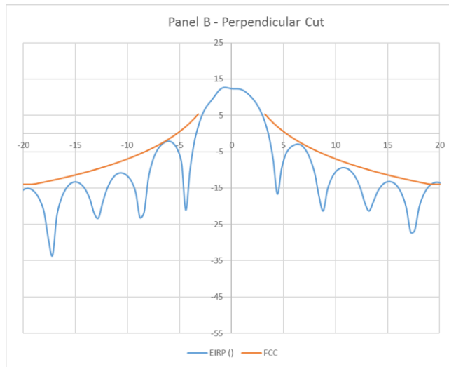
Panel B EIRP Mask vs FCC EIRP Mask - Elevation
