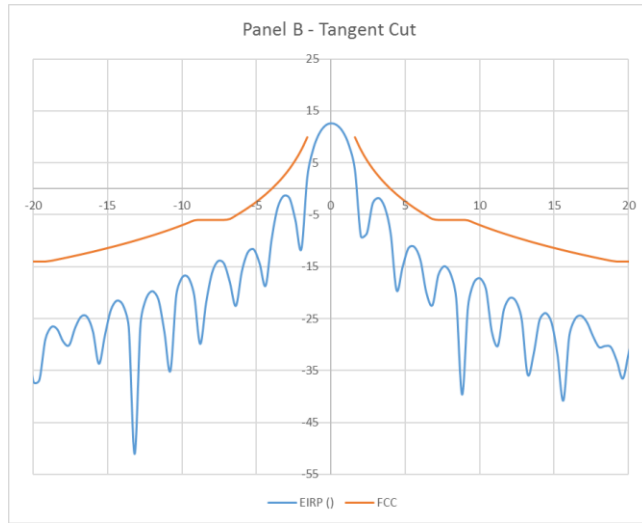
Panel B EIRP Mask vs FCC EIRP Mask - Azimuth
