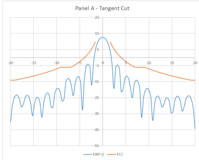
Panel A EIRP Mask vs FCC EIRP Mask - Azimuth
