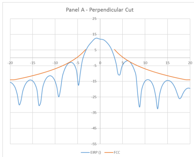
Panel A EIRP Mask vs FCC EIRP Mask - Elevation
