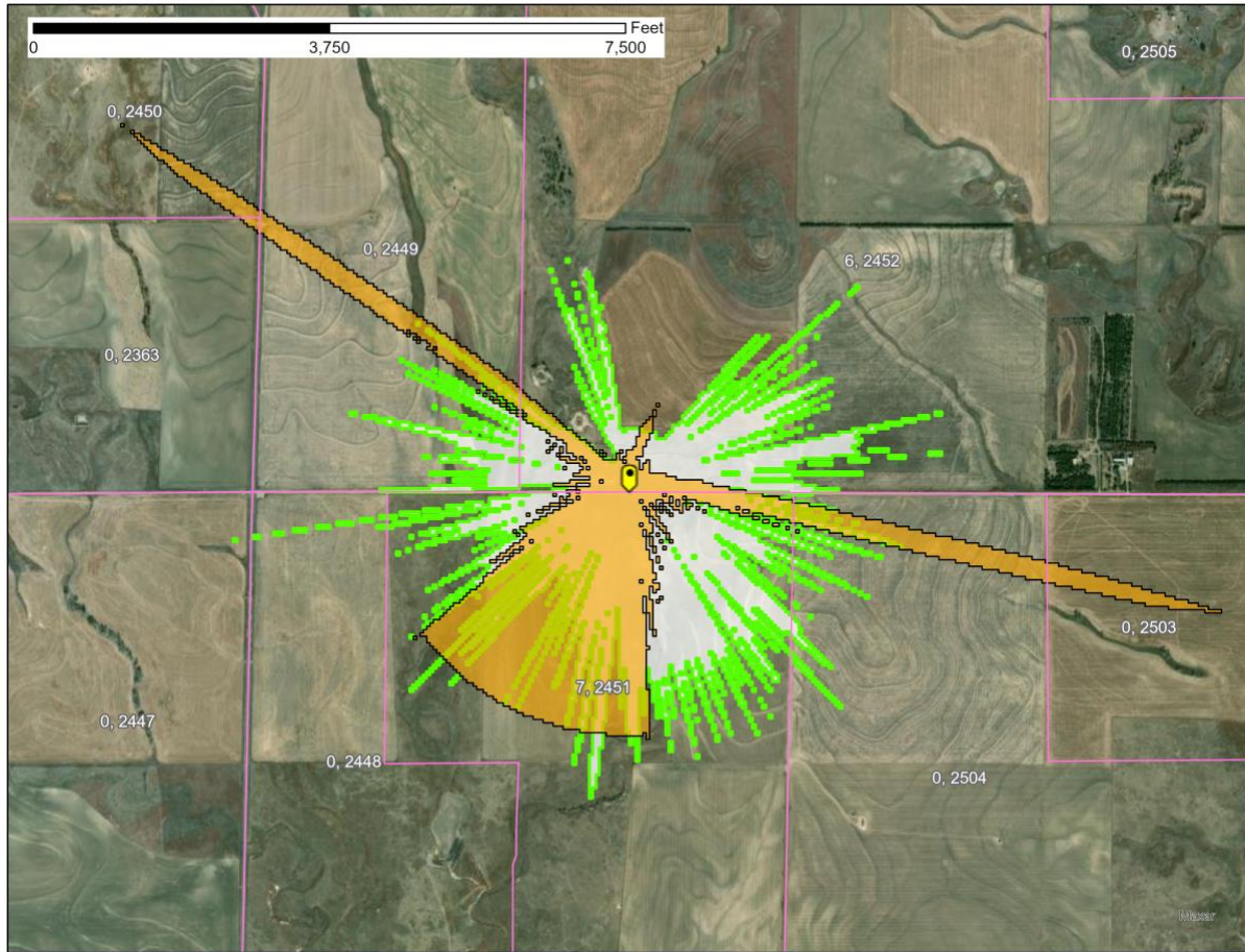
Figure 2 – Ellis, KS SAN and E110049 combined -77.6 dB(mW/(m² * MHz)) pfd contours
