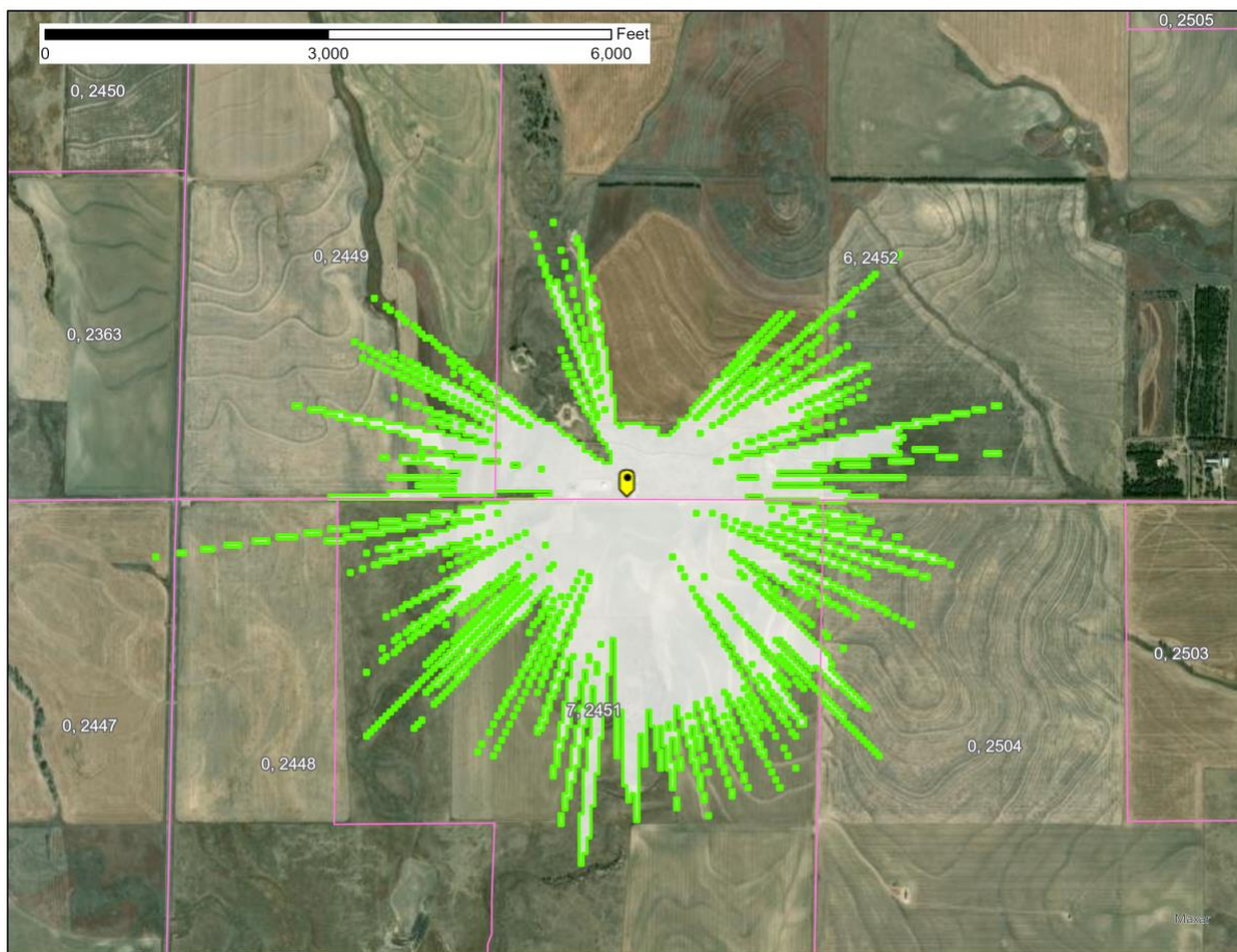
Figure 1 – Ellis, KS SAN -77.6 dB(mW/(m 2 * MHz)) pfd contour
