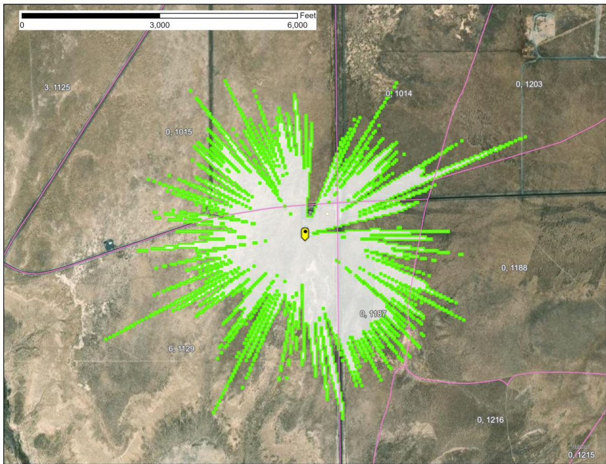
Figure 1 – Milford, UT SAN -77.6 dB(mW/(m² * MHz)) pfd contour
