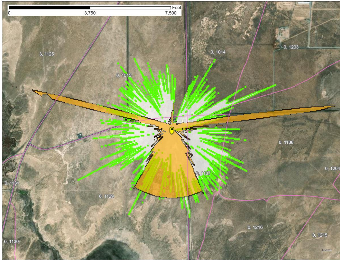
Figure 2 – Milford, UT SAN and E110026 earth station combined -77.6 dB(mW/(m 2 * MHz)) pfd contours
