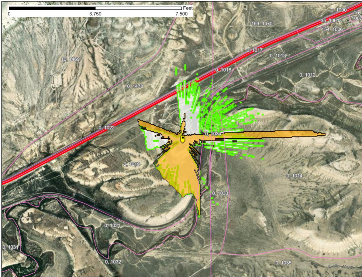
Figure 2 – Green River, WY SAN and E110047 earth station aggregate -77.6 \text{ dB(mW/(m}^2 * \text{ MHz)) pfd} contours
