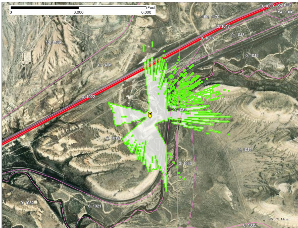
Figure 1 – Green River, WY SAN -77.6 dB(mW/(m 2 * MHz)) pfd contour
