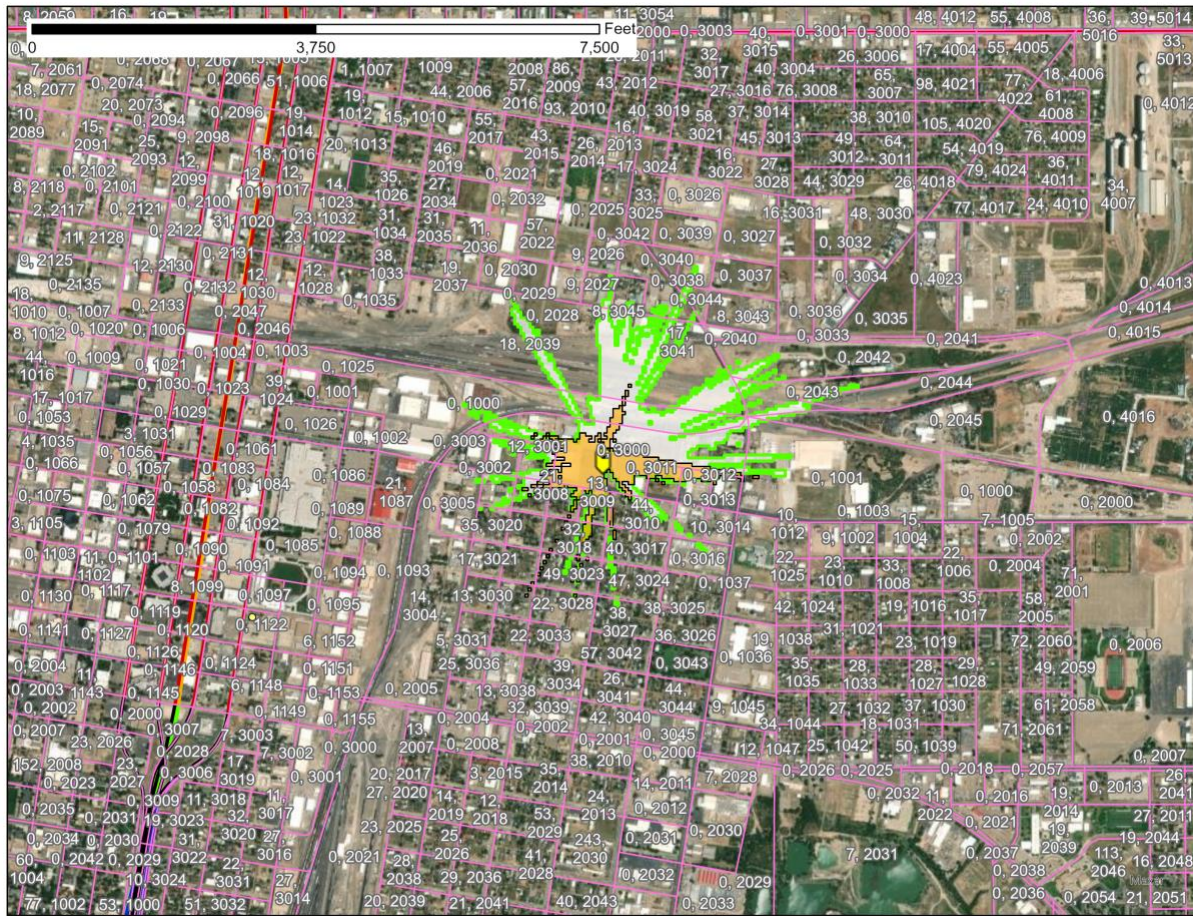
Figure 2 – Amarillo, TX Combined SAN and Viasat E110050 ES -77.6 dB(mW/(m 2 * MHz)) pfd contour
