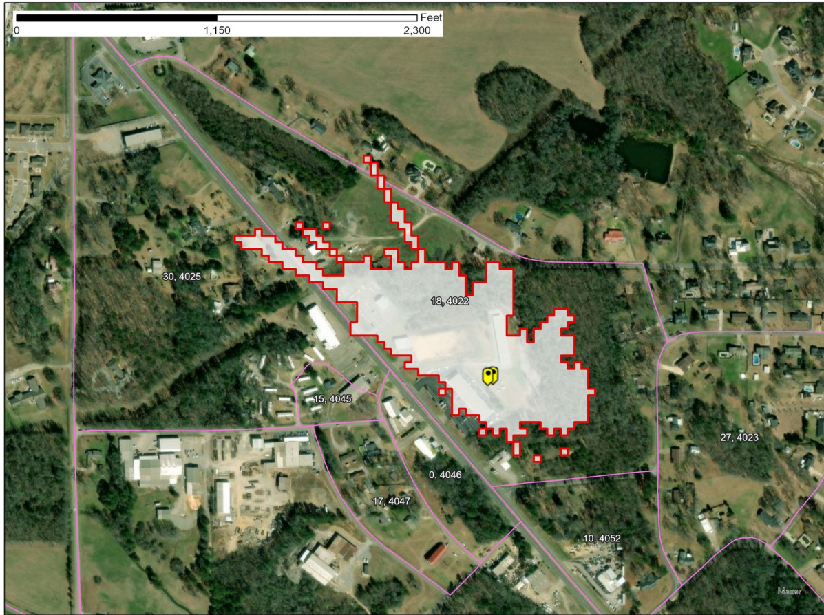
Figure 1 – Clanton, AL SAN -77.6 dB(mW/(m2 * MHz)) pfd contour
