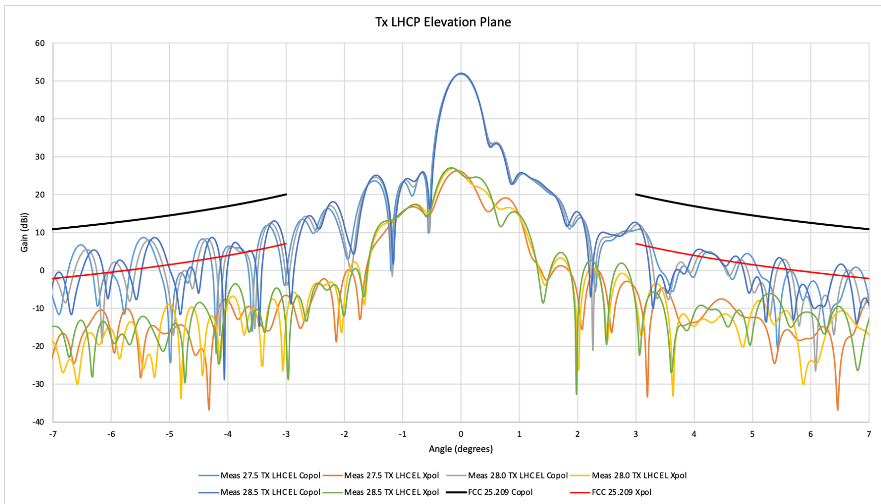
Figure 4 Tx LHCP Elevation Plane Narrow Cut
