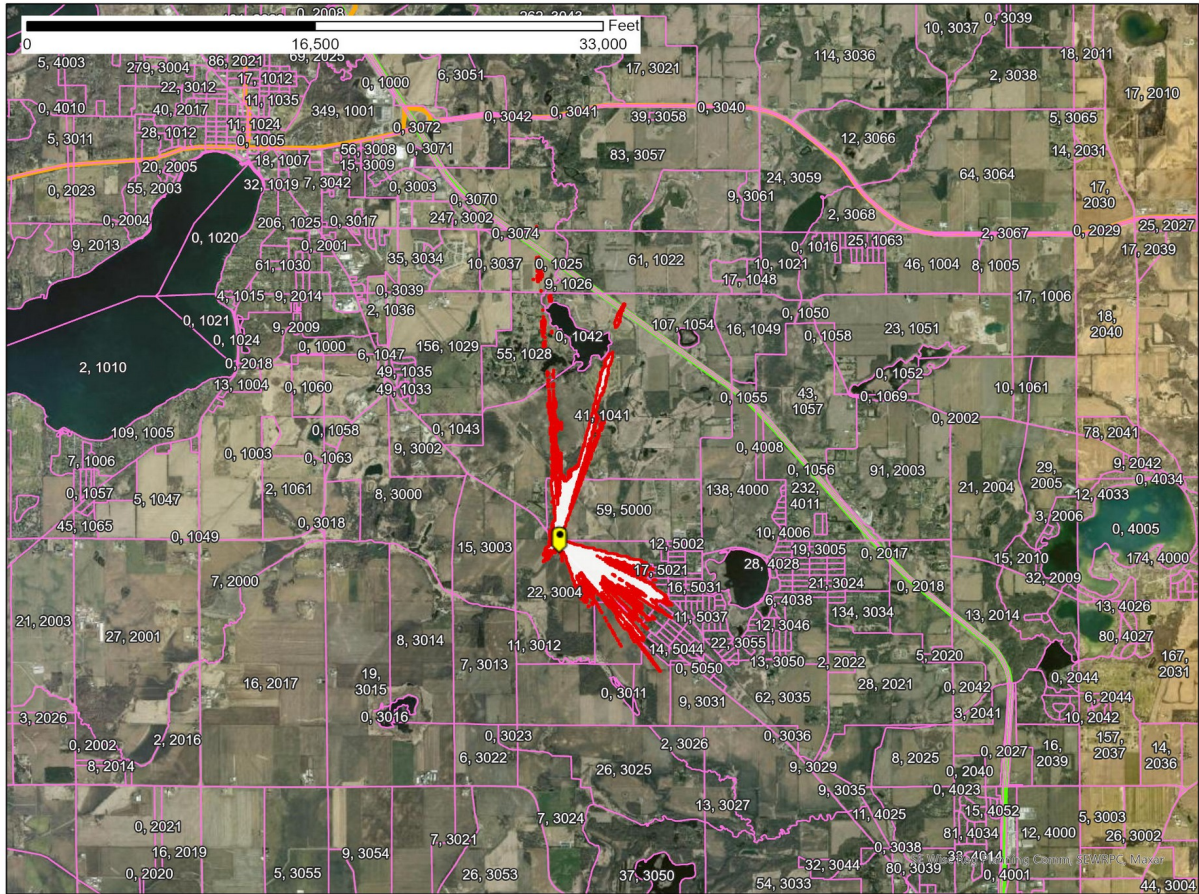
Figure 1 – Lake Geneva, WI SAN -77.6 dB(mW/(m2 * MHz)) pfd contour
