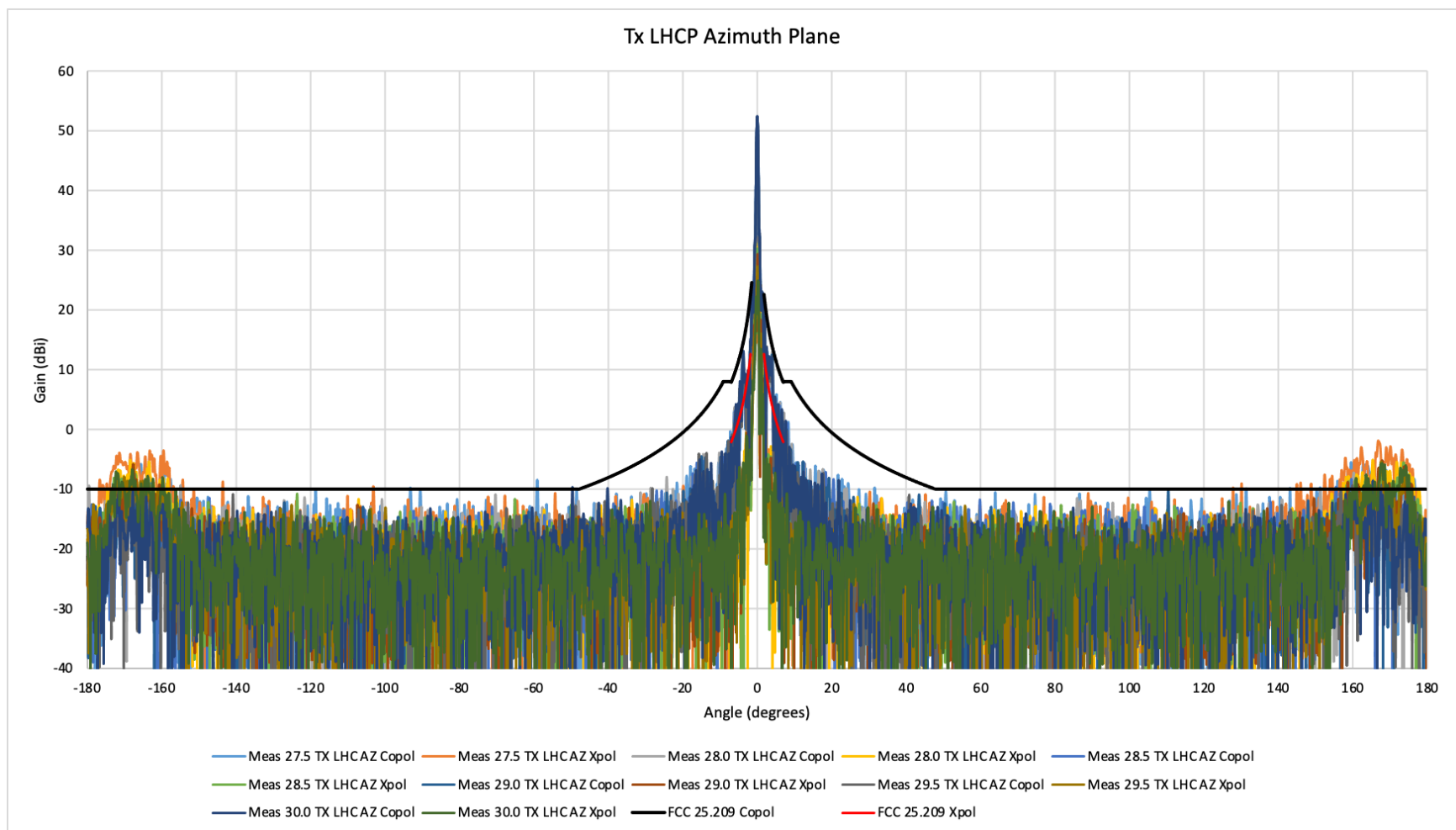
Figure 1 Tx LHCP Azimuth Plane Wide Cut
