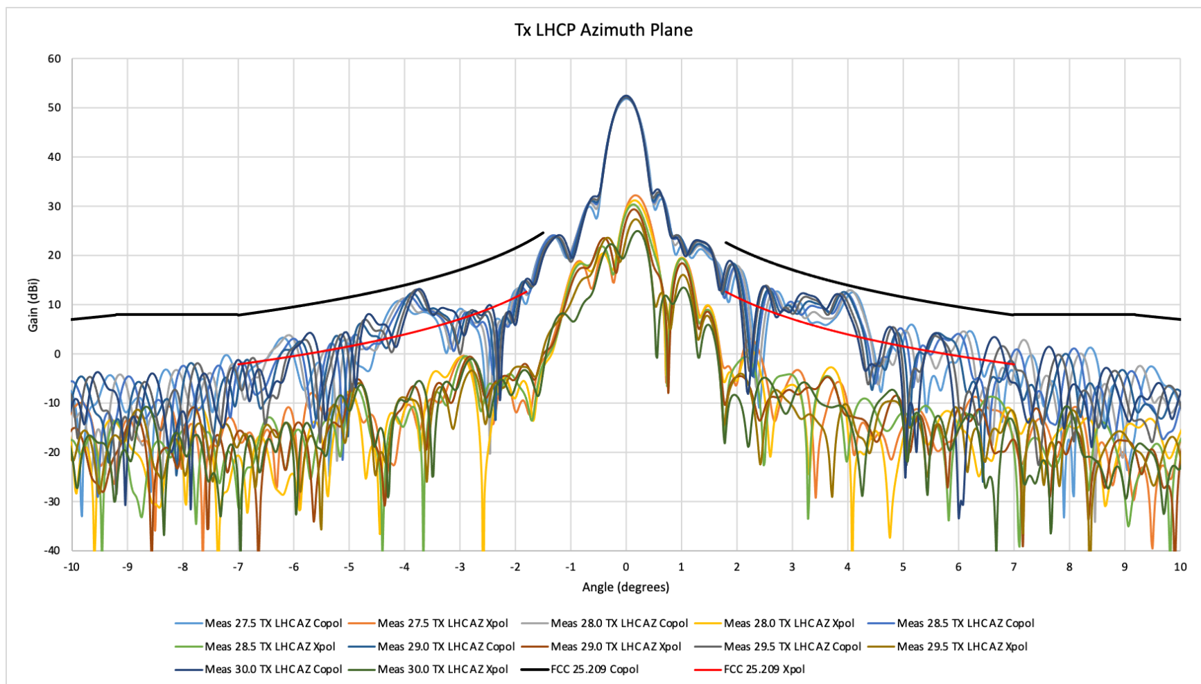
Figure 2 Tx LHCP Azimuth Plane Narrow Cut
