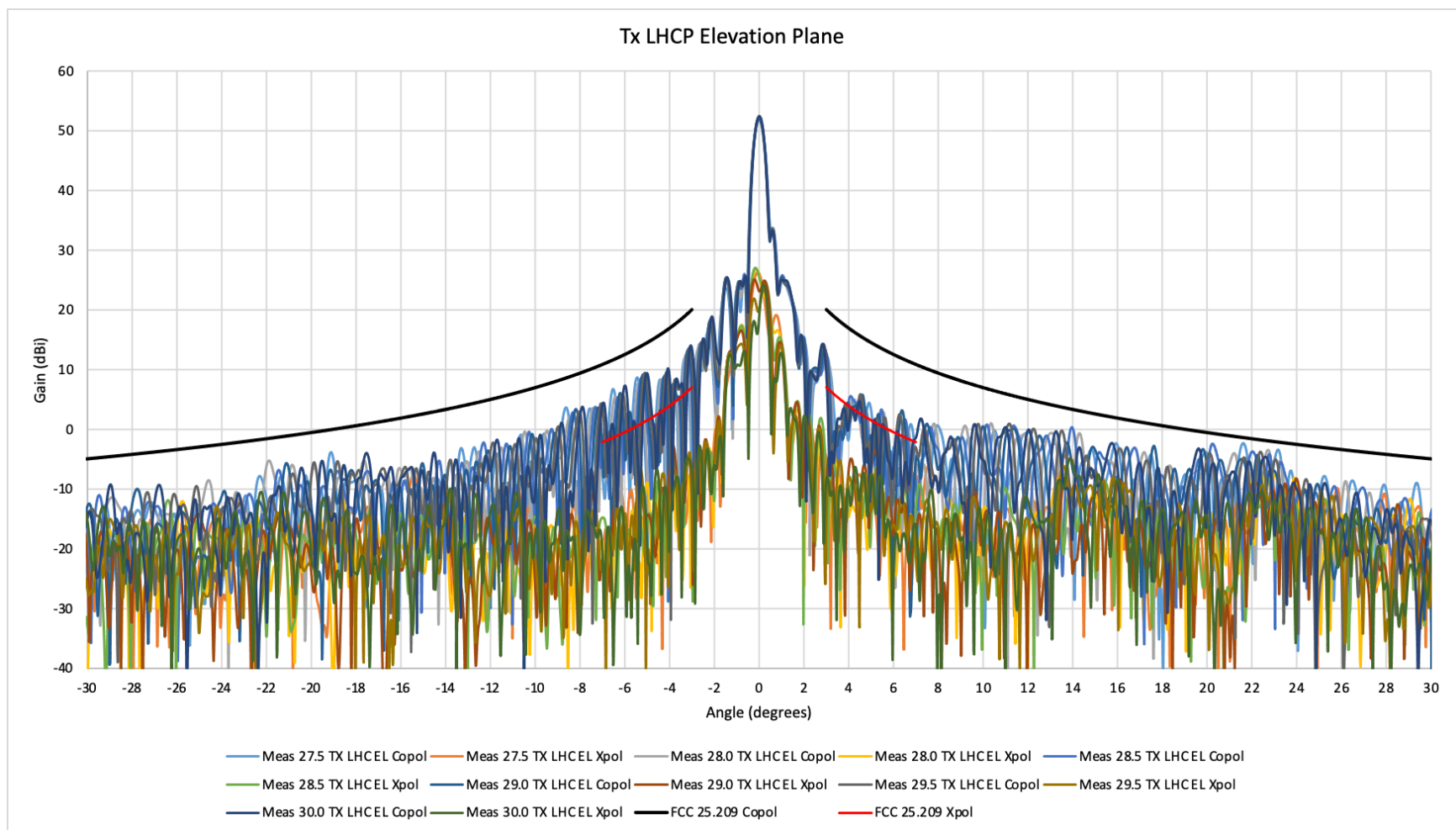
Figure 3 Tx LHCP Elevation Plane Wide Cut
