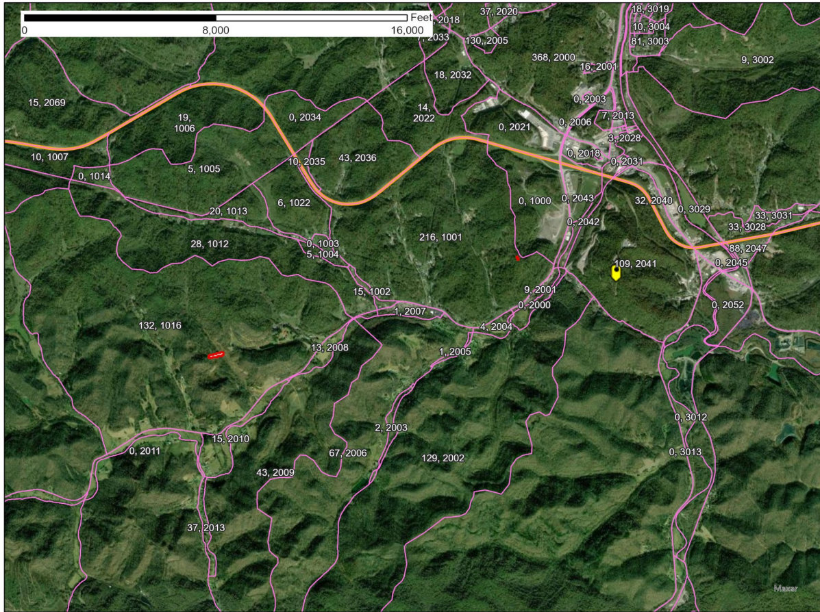
Figure 1 – Manchester, KY SAN -77.6 dB(mW/(m2 * MHz)) pfd contour
