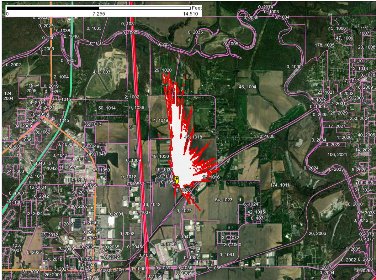
Figure 1 – Springfield, IL SAN -77.6 dB(mW/(m2 * MHz)) pfd contour
