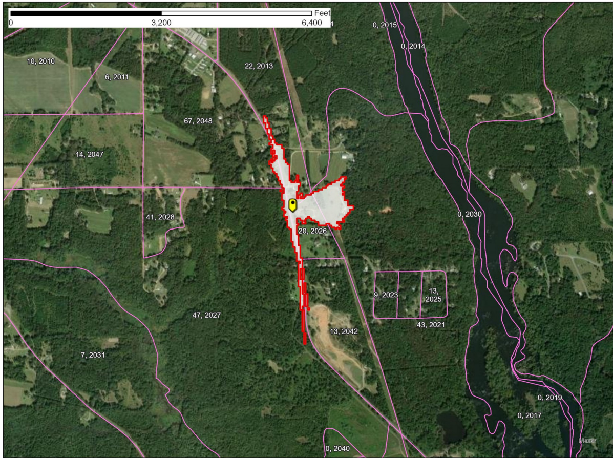
Figure 1 – Wetumpka, AL SAN -77.6 dB(mW/(m2 * MHz)) pfd contour
