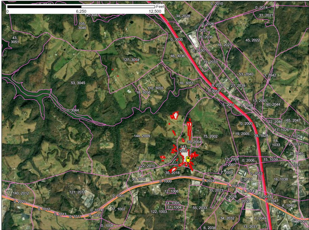
Figure 1 – London, KY SAN -77.6 dB(mW/(m2 * MHz)) pfd contour
