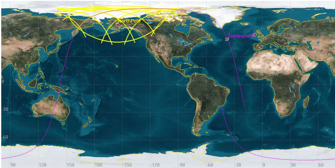
USN Alaska coverage of Sentinels-2A (typical coverage each day) Pre-LEOP June 2020
