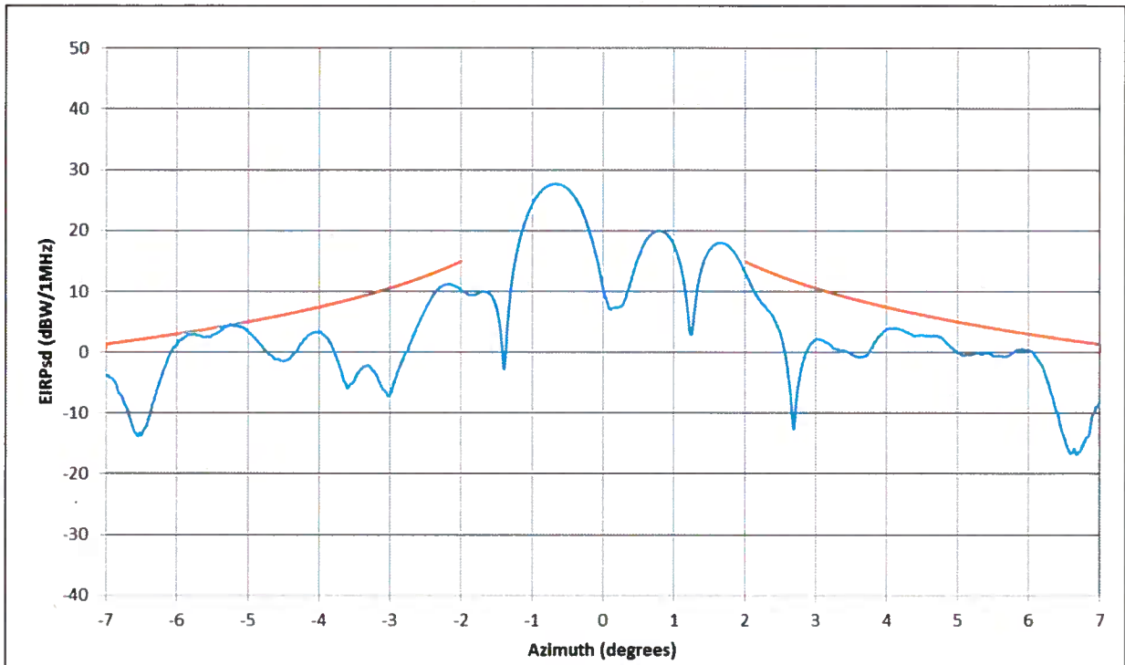
X-Pol EIRP density in the plane tangent to the GSO Arc 29.5 GHz (-7 to +7 degrees)
