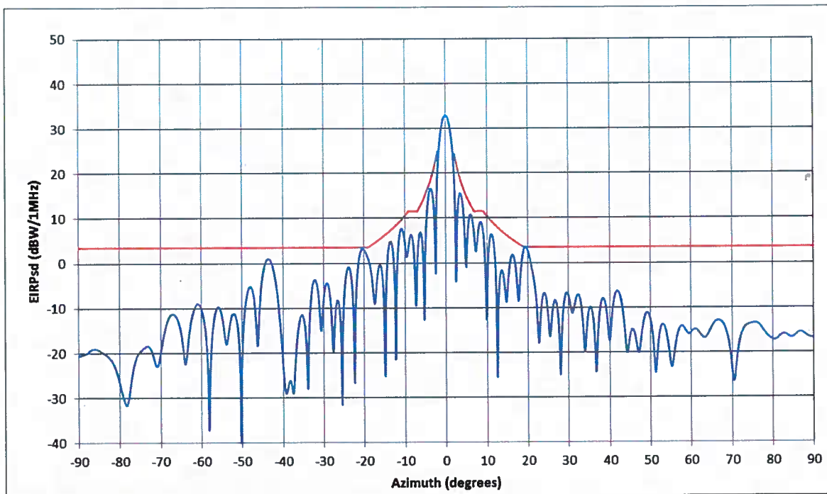
Co-Pol EIRP density in the Plane Tangent to the GSO Arc 30 GHZ
