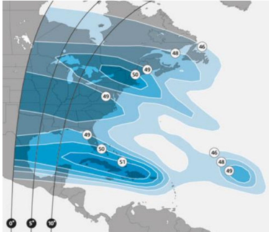
Figure 1. Ku-Band Coverage (NSS-7 at 20W) (Ku-band exclusion zone around radio astronomy sites, as indicated in Narrative)
