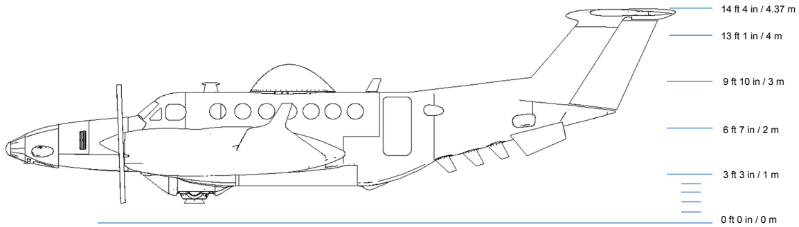
Figure 3-2. Aircraft Configuration
