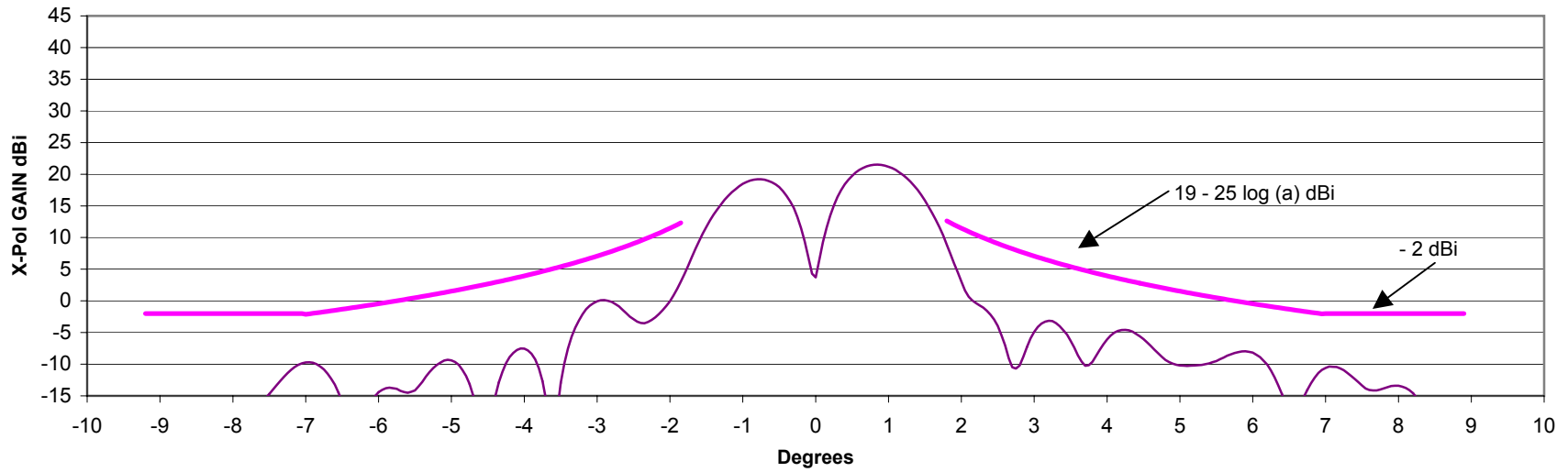
6.04 GHz Cross Pol Gain, Az E-Plane
