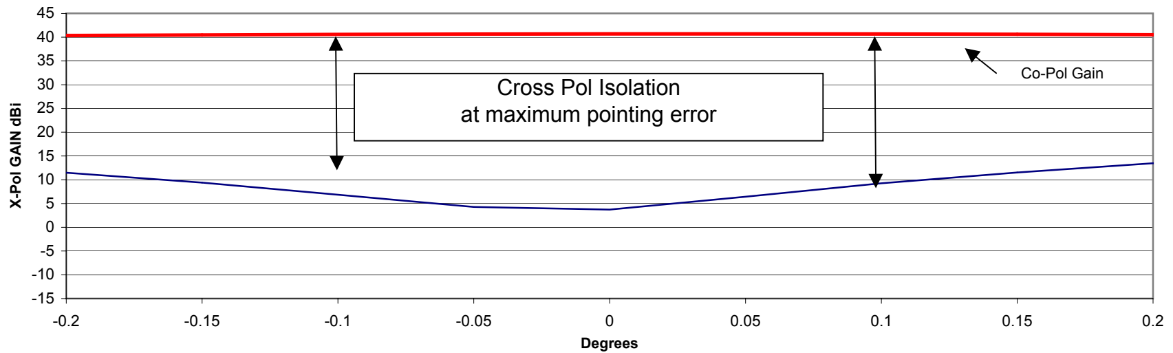
6.04 GHz Cross Pol Isolation, Az E-Plane
