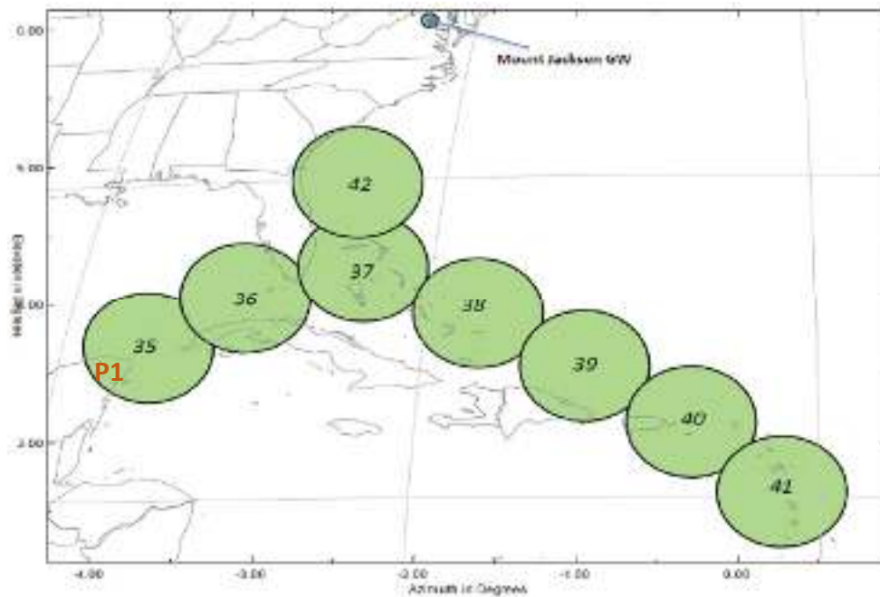
Figure 3: Telstar 19V Coverage Area and Skew Angles for Thales ESAA Operation (Worst-Case Skew Angle of ~45°, Elevation 15° at position P1 in red)
