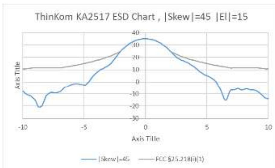
Figure 6 – AMC-15 Skew = 45 degrees and Elevation = 15 degrees ESD. The chart represents the highest allowed power level of 34.5 dBW/MHz (10.5 dBW/4kHz). Thales system will limit power to this level when at this position.
