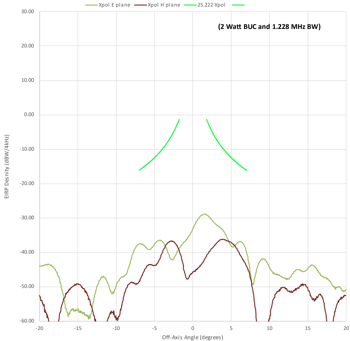
H60 Transmit Azimuth 14.25 GHz Xpol EIRP
