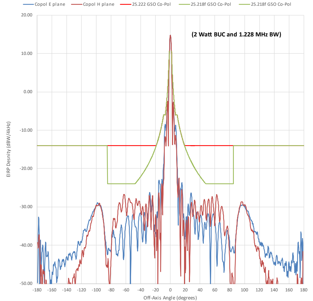
H60 Transmit Azimuth 14.25 GHz Copol EIRP
