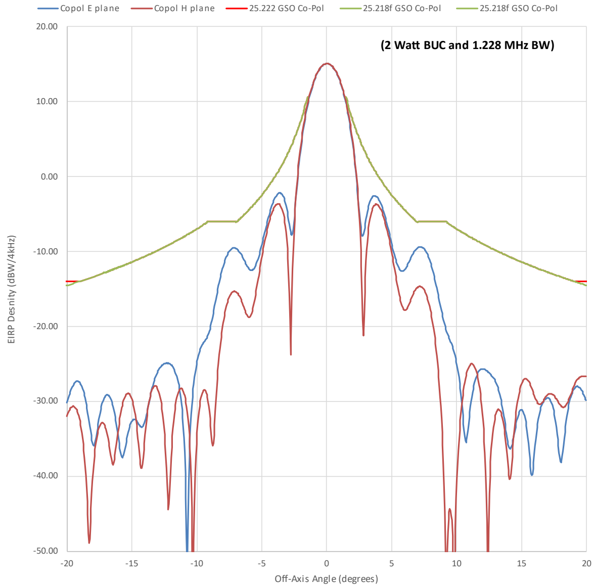
H60 Transmit Azimuth 14.50 GHz Copol EIRP
