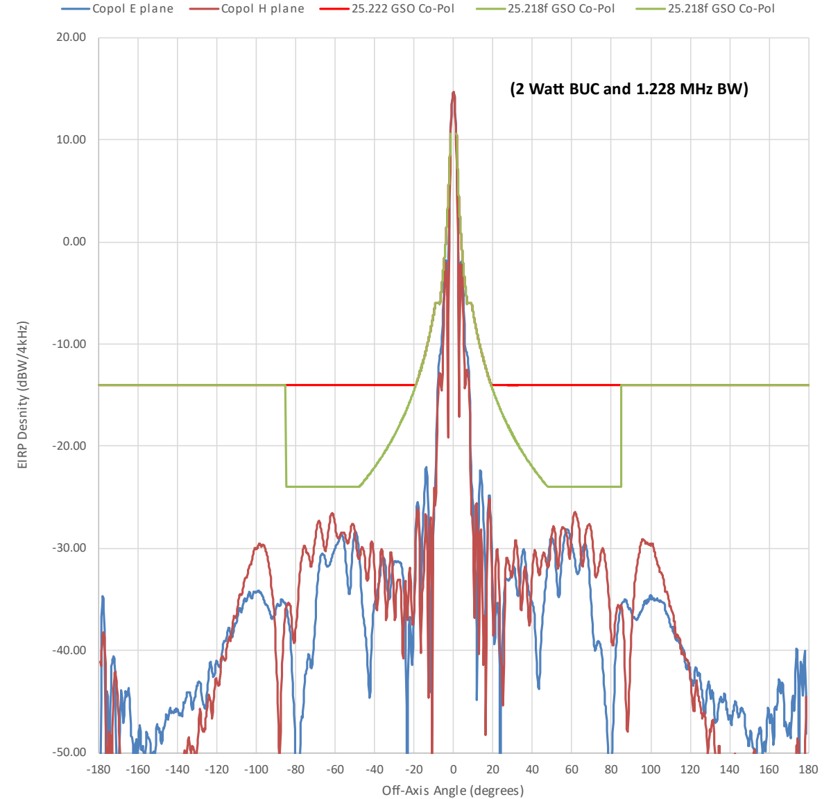
H60 Transmit Azimuth 14.00 GHz Copol EIRP
