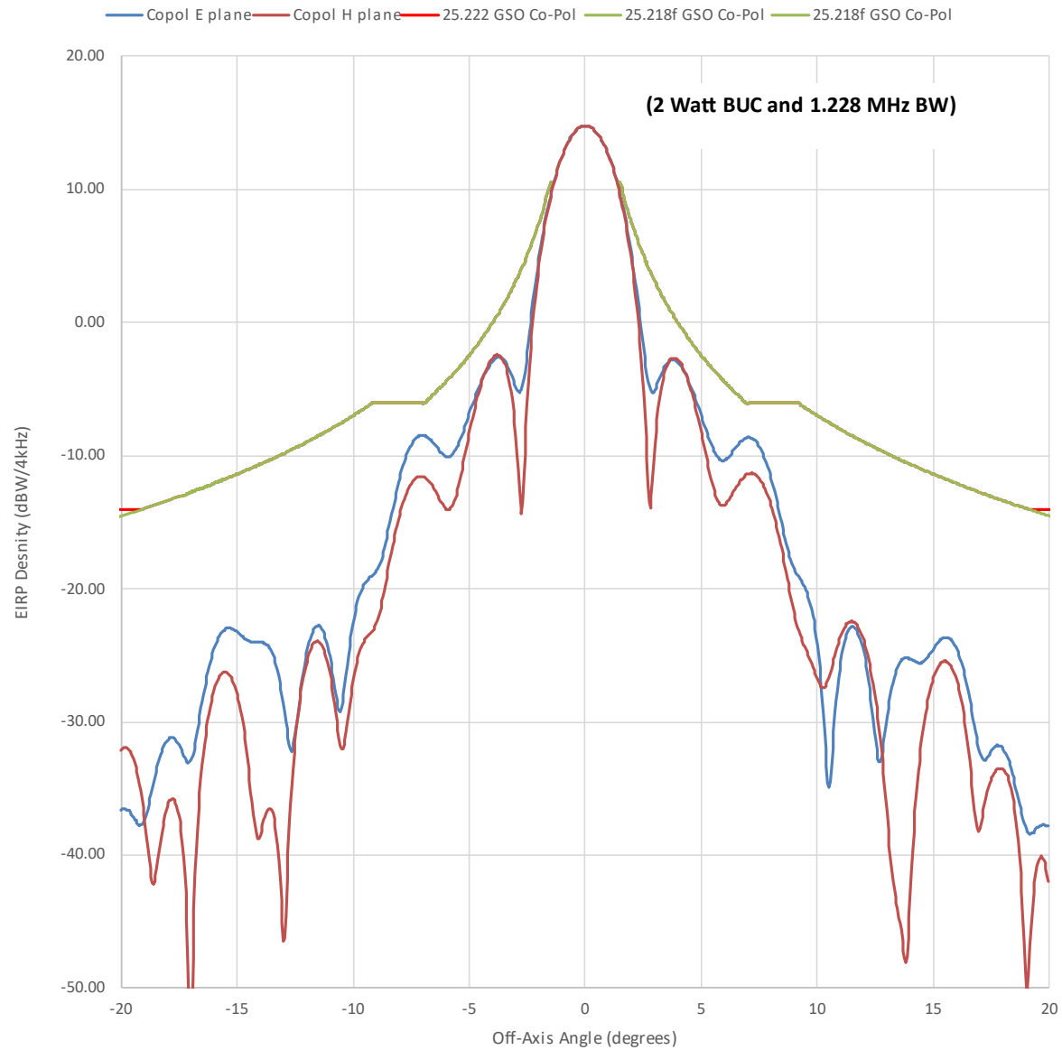
H60 Transmit Azimuth 14.25 GHz Copol EIRP
