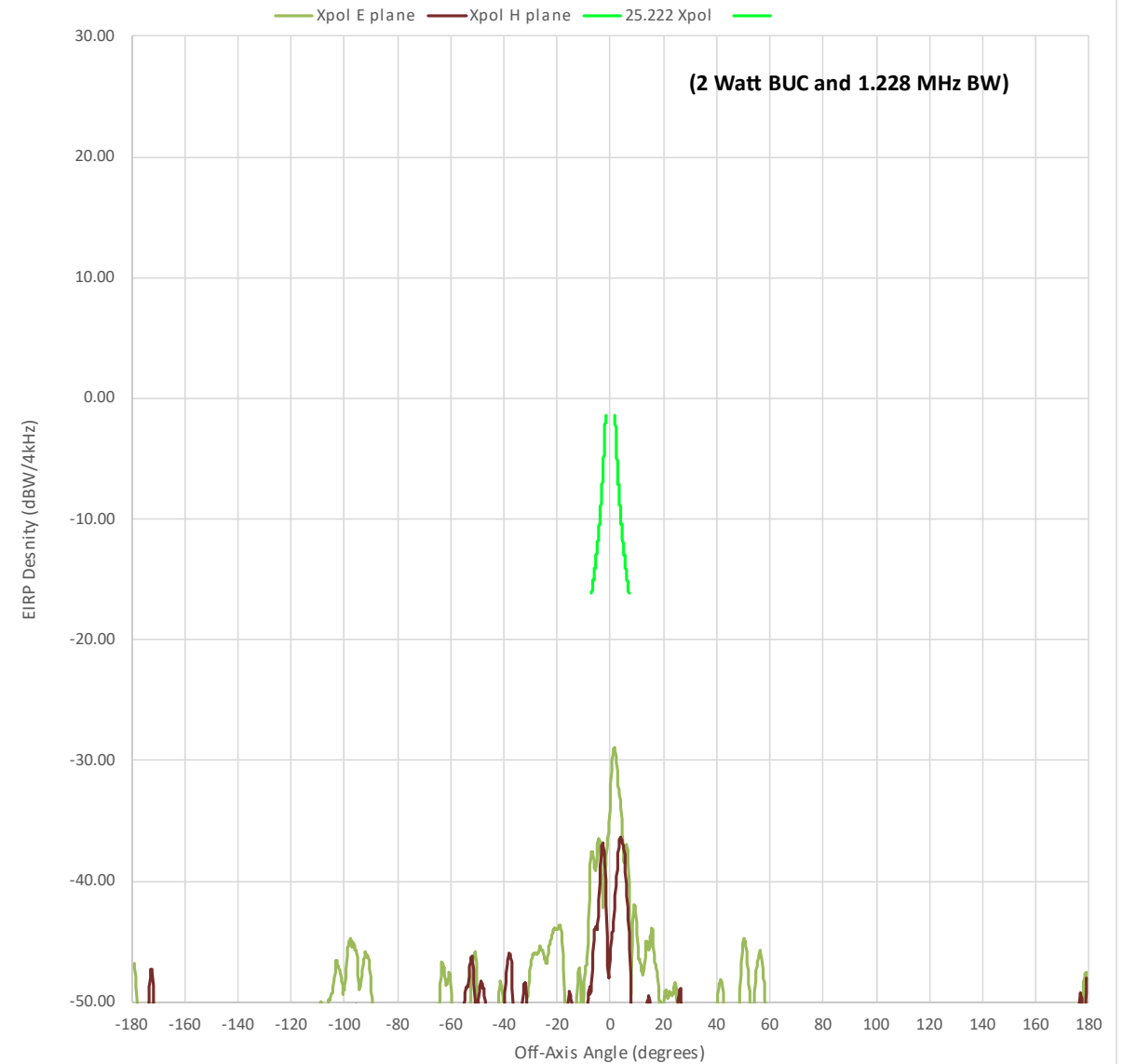
H60 Transmit Azimuth 14.25 GHz Xpol EIRP
