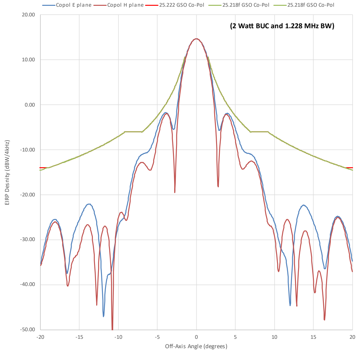
H60 Transmit Azimuth 14.00 GHz Copol EIRP
