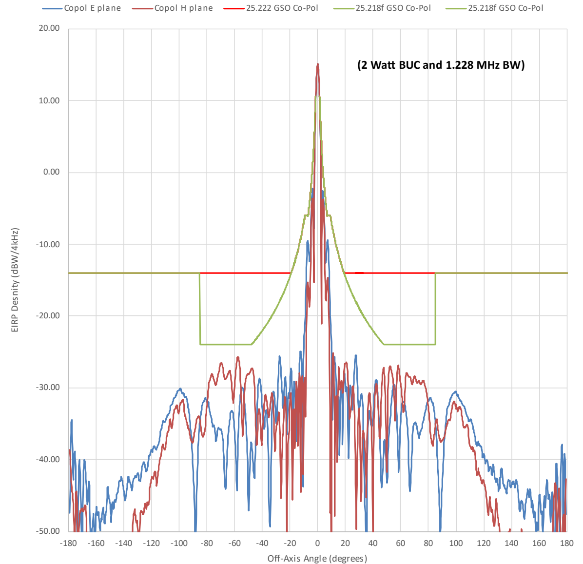
H60 Transmit Azimuth 14.50 GHz Copol EIRP
