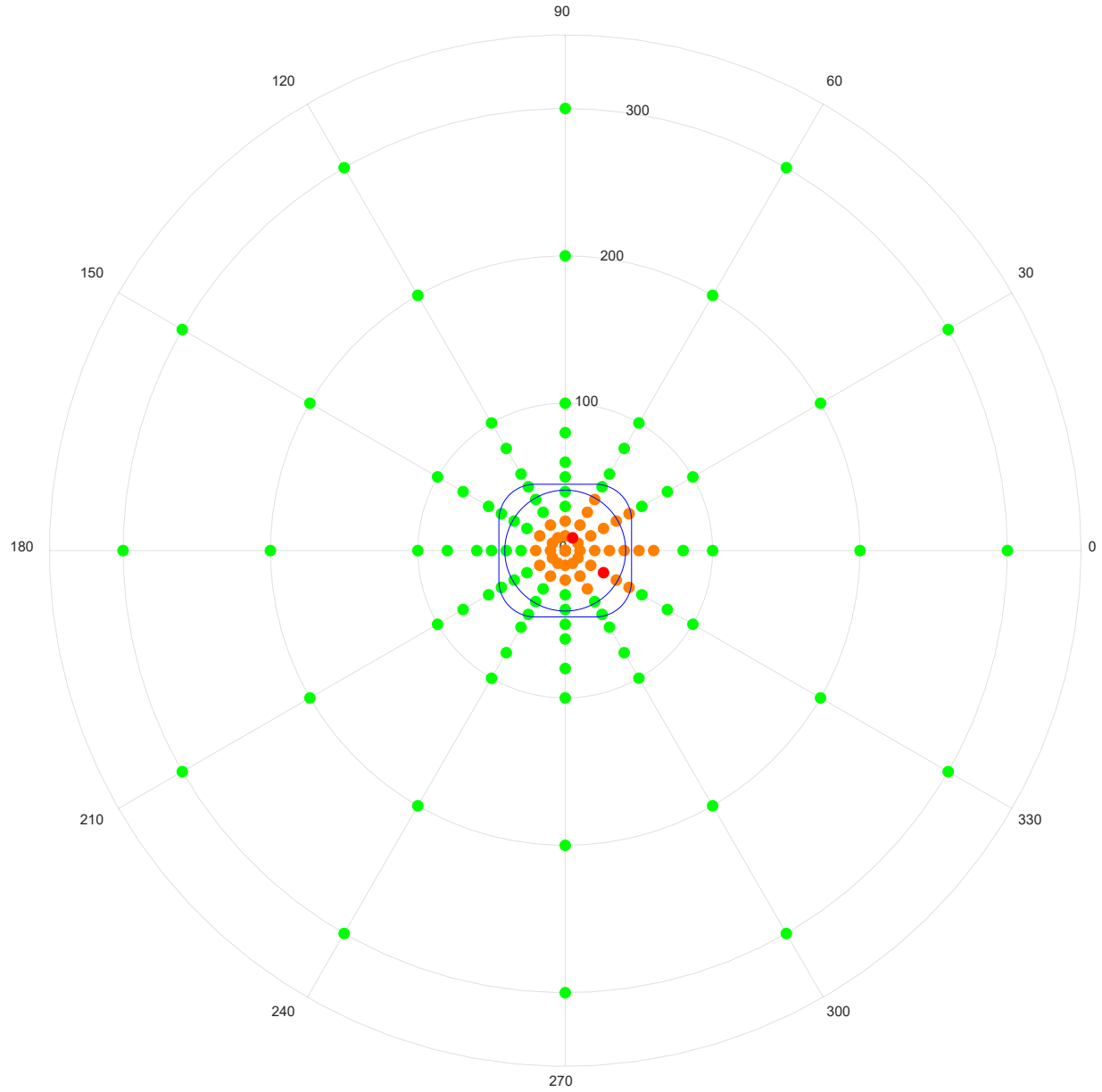
Figure 14: Height 0 cm, 40 W with 30% Duty Cycle, Scan 75 degrees
