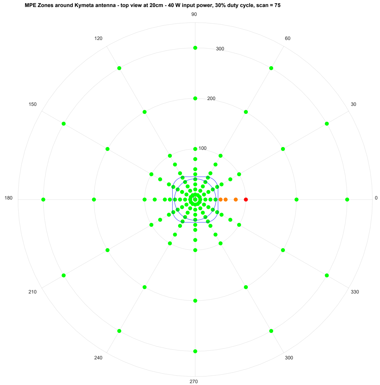
Figure 16: Height 20 cm, 40 W with 30% Duty Cycle, Scan 75 degrees
