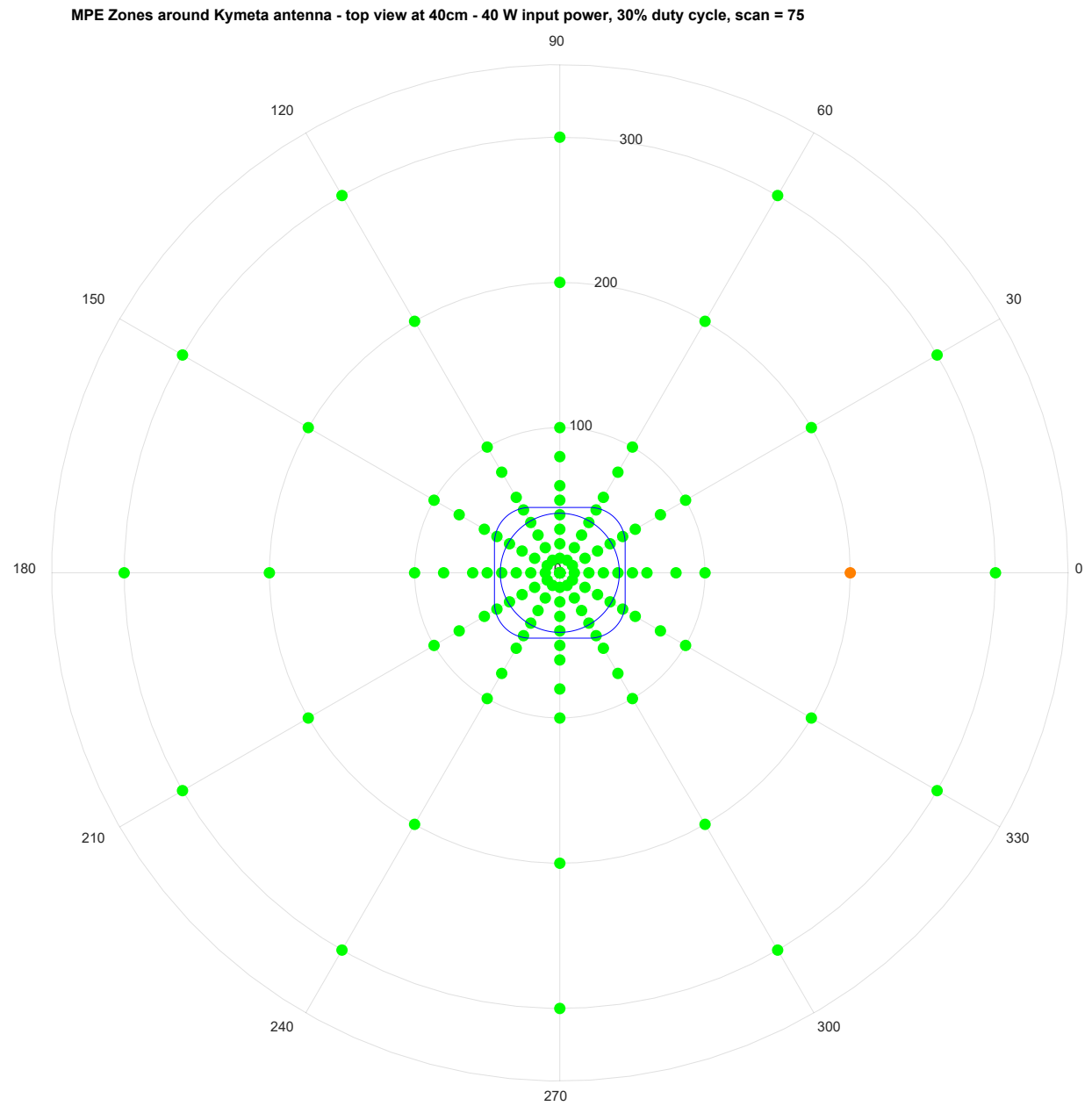
Figure 18: Height 40 cm, 40 W with 30% Duty Cycle, Scan 75 degrees
