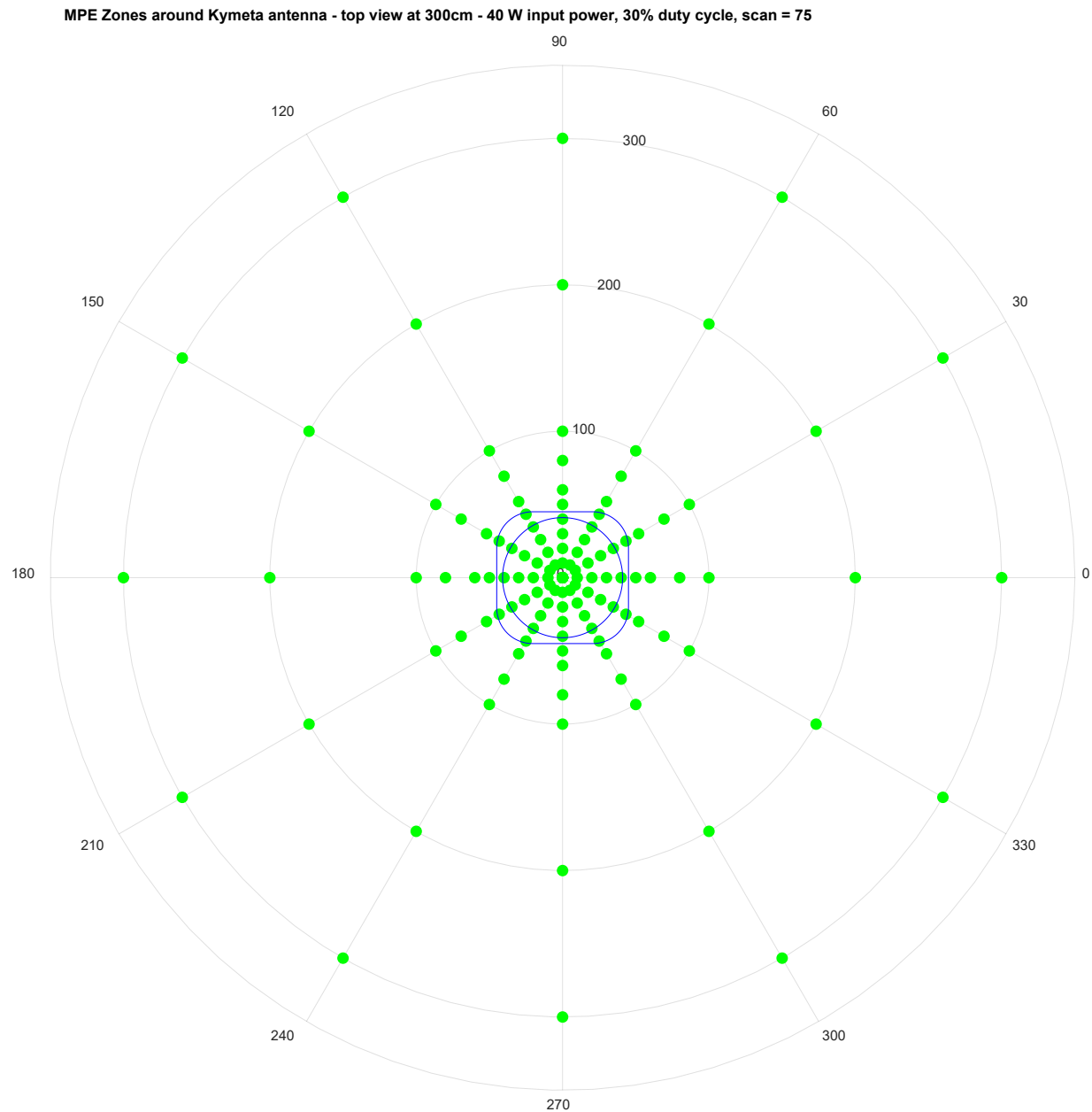
Figure 22: Height 300 cm, 40 W with 30% Duty Cycle, Scan 75 degrees
