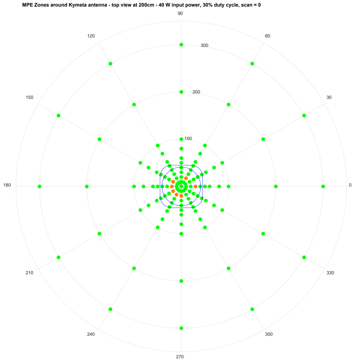
Figure 12: Height 200 cm, 40 W with 30% Duty Cycle, Scan 0 degrees
