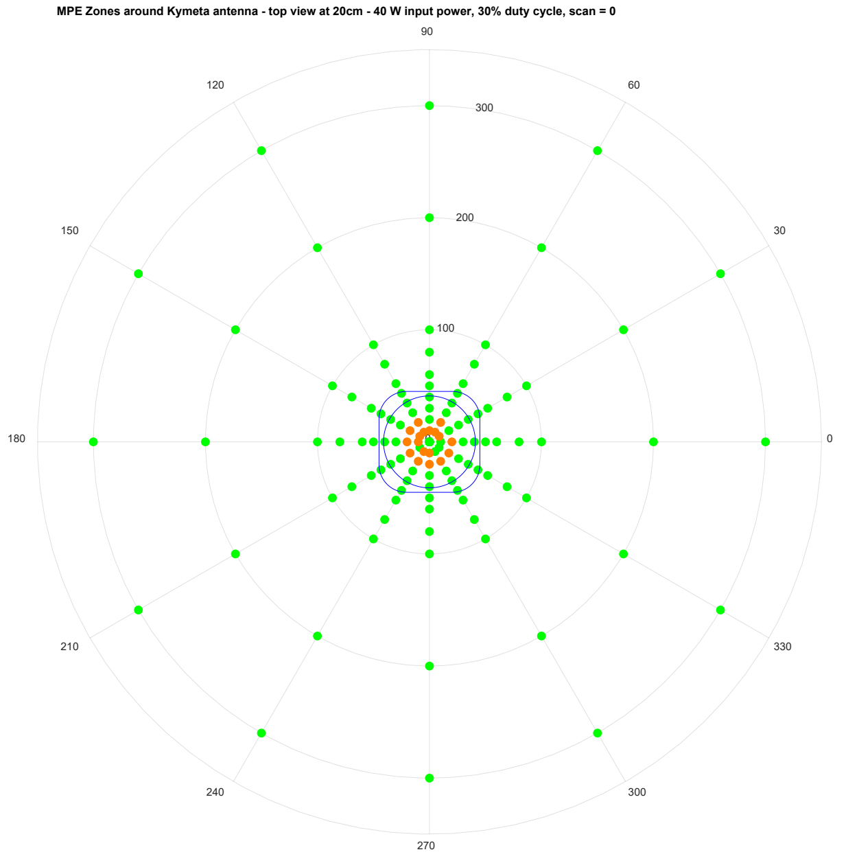
Figure 7: Height 20 cm, 40 W with 30% Duty Cycle, Scan 0 degrees
