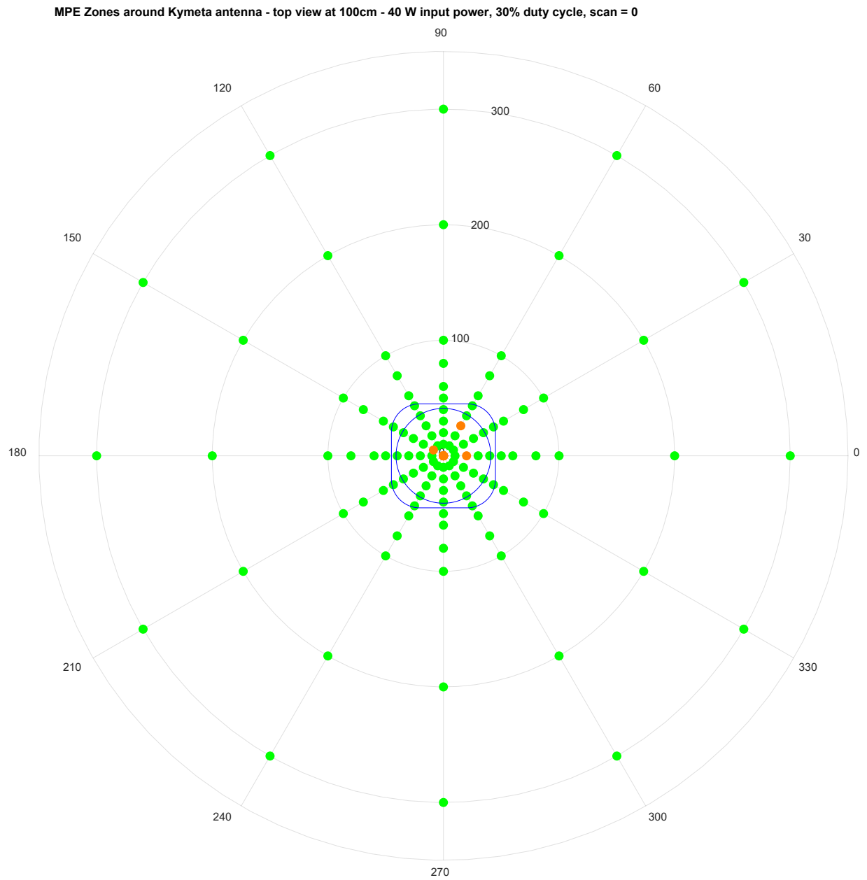
Figure 11: Height 100 cm, 40 W with 30% Duty Cycle, Scan 0 degrees
