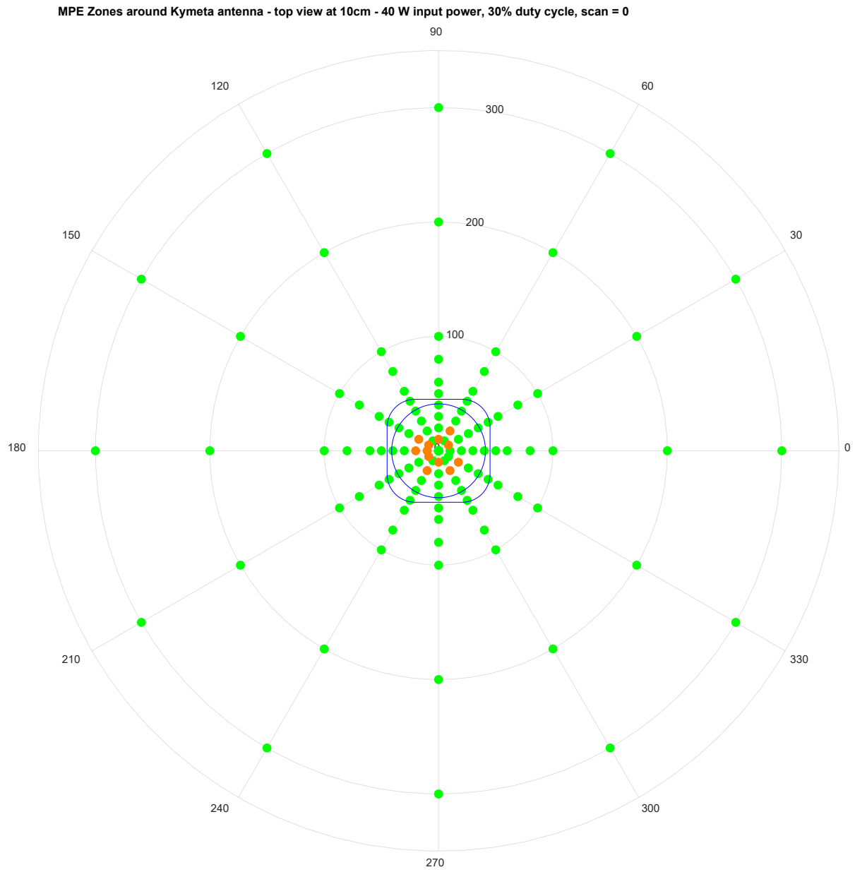
Figure 6: Height 10 cm, 40 W with 30% Duty Cycle, Scan 0 degrees
