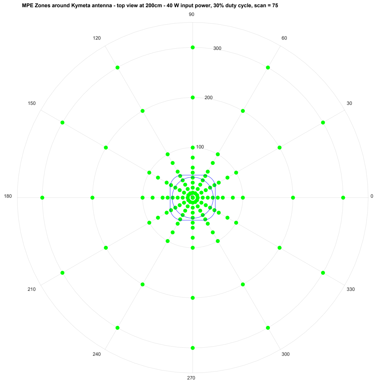
Figure 21: Height 200 cm, 40 W with 30% Duty Cycle, Scan 75 degrees
