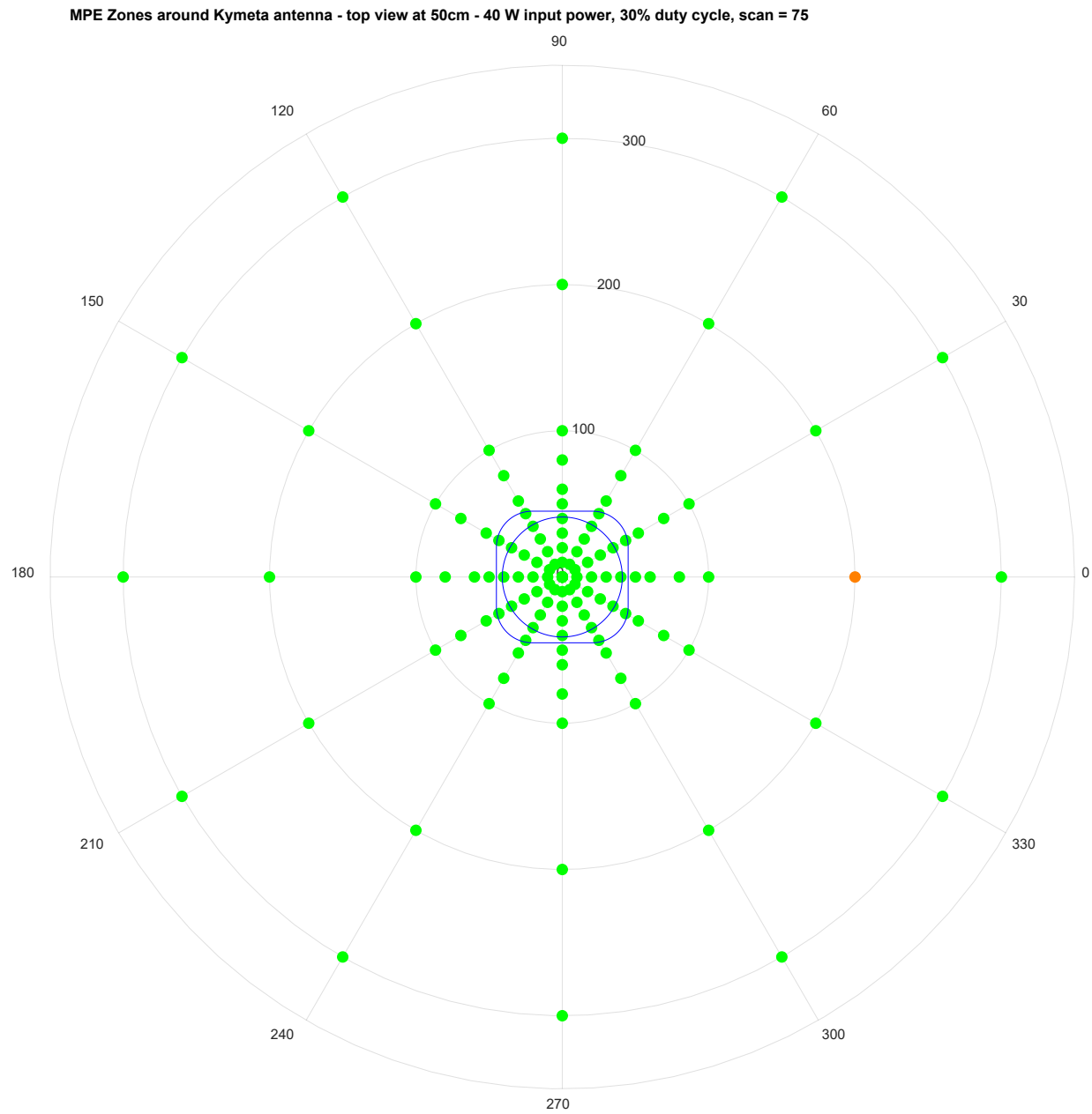
Figure 19: Height 50 cm, 40 W with 30% Duty Cycle, Scan 75 degrees
