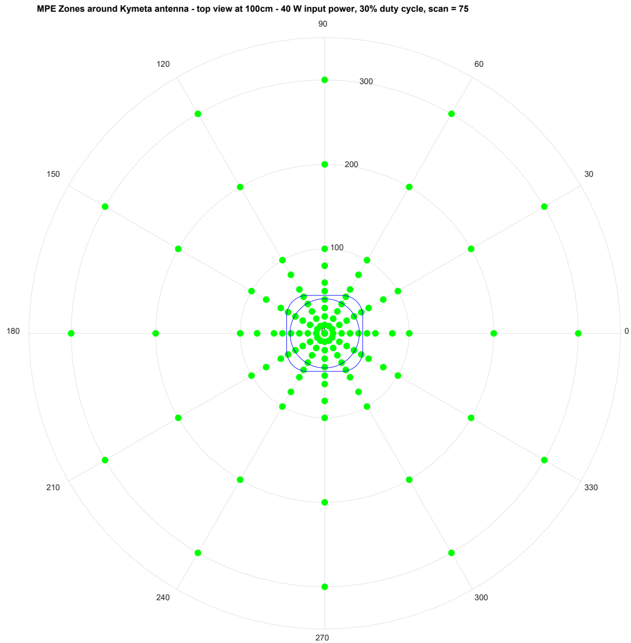
Figure 20: Height 100 cm, 40 W with 30% Duty Cycle, Scan 75 degrees
