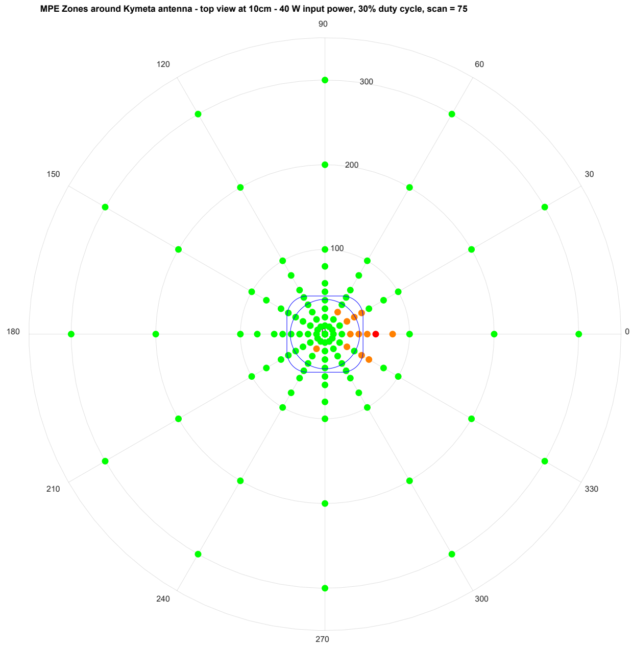
Figure 15: Height 10 cm, 40 W with 30% Duty Cycle, Scan 75 degrees
