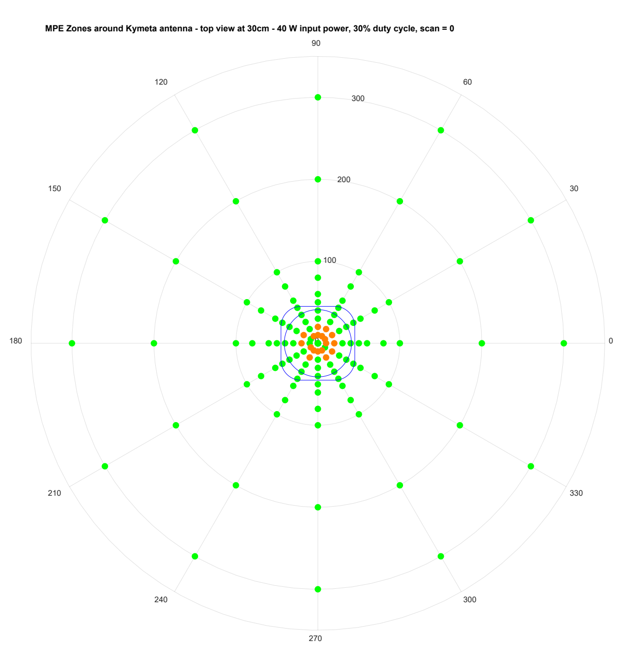
Figure 8: Height 30 cm, 40 W with 30% Duty Cycle, Scan 0 degrees
