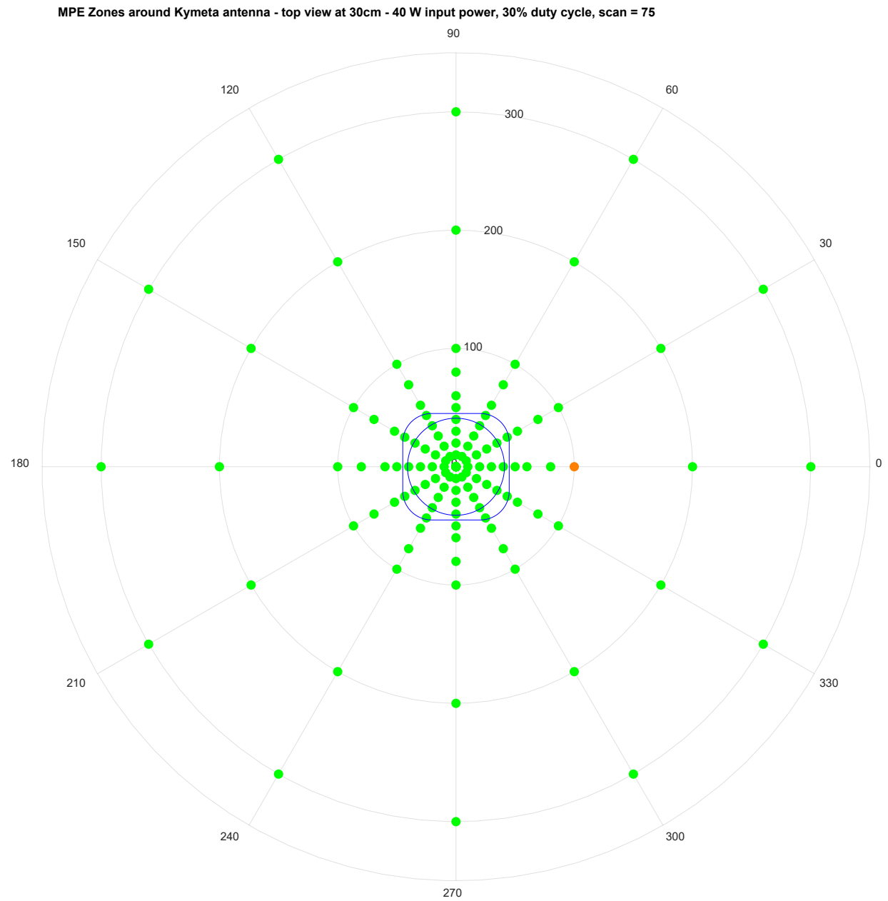
Figure 17: Height 30 cm, 40 W with 30% Duty Cycle, Scan 75 degrees
