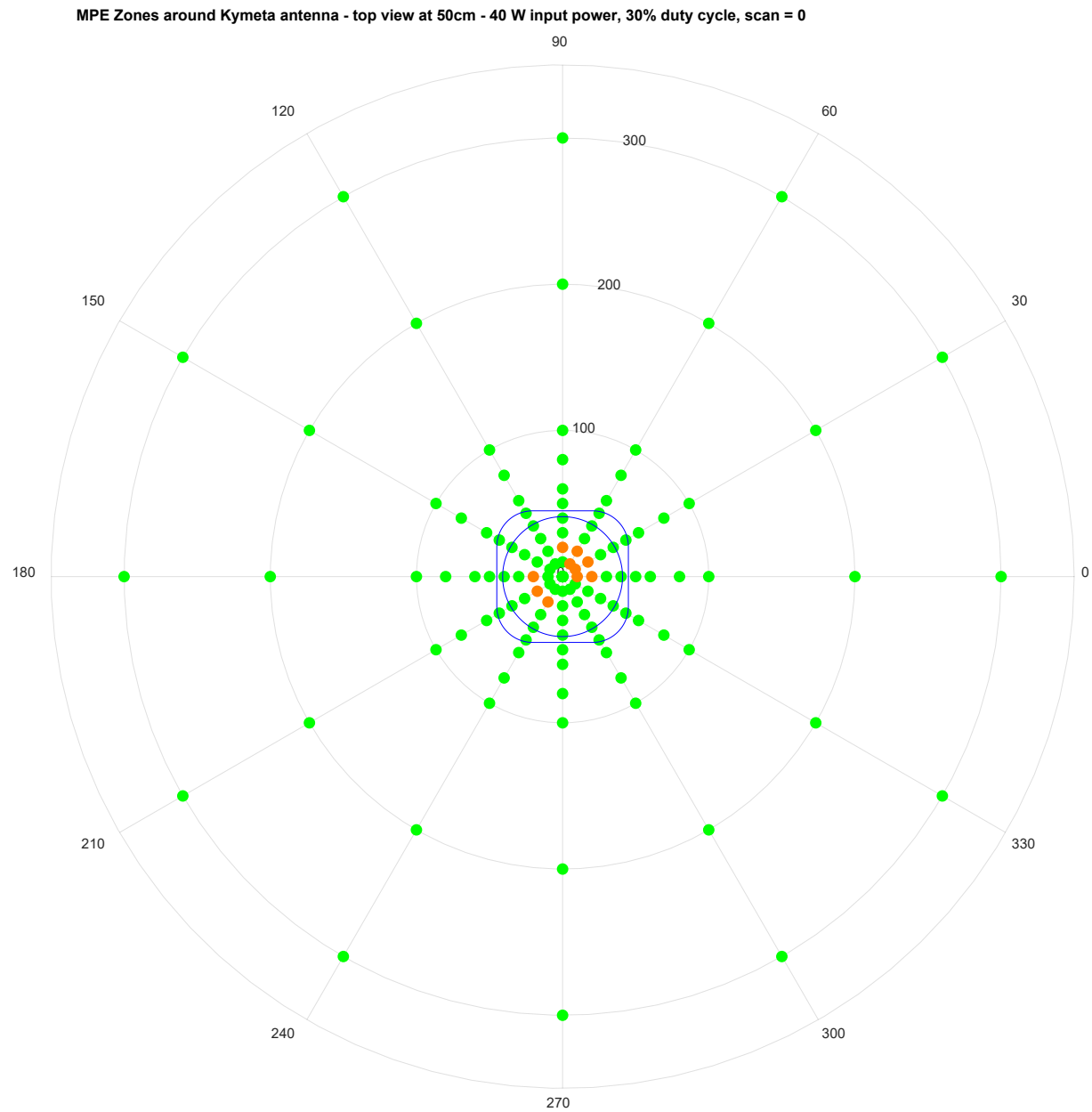
Figure 10: Height 50 cm, 40 W with 30% Duty Cycle, Scan 0 degrees
