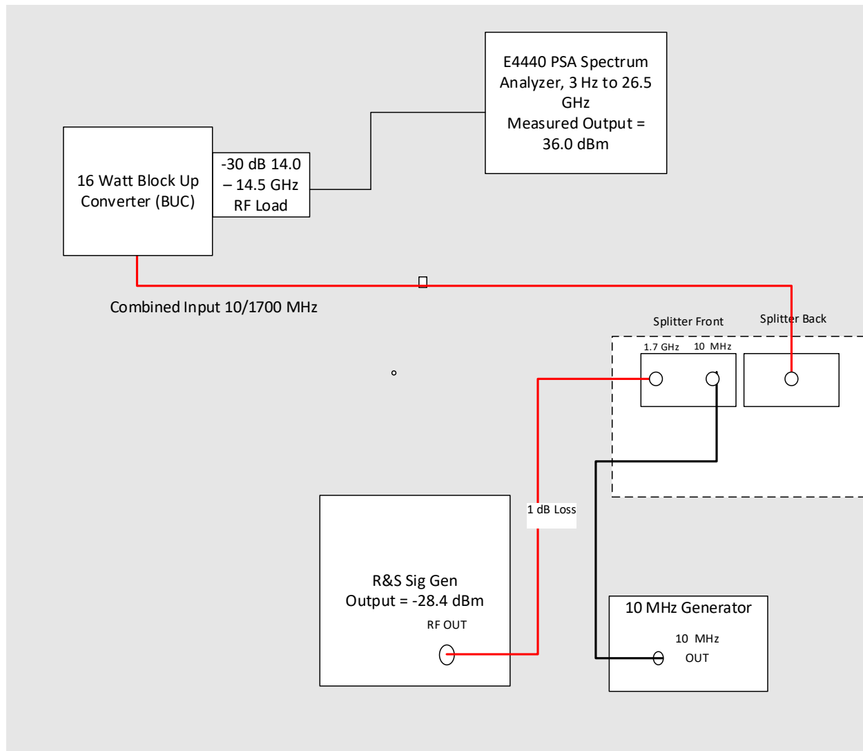
Figure 3: Input reference power calibration diagram
