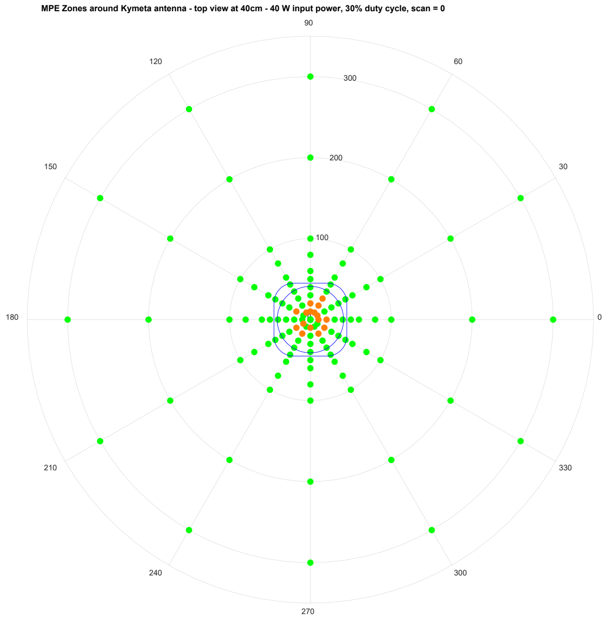
Figure 9: Height 40 cm, 40 W with 30% Duty Cycle, Scan 0 degrees
