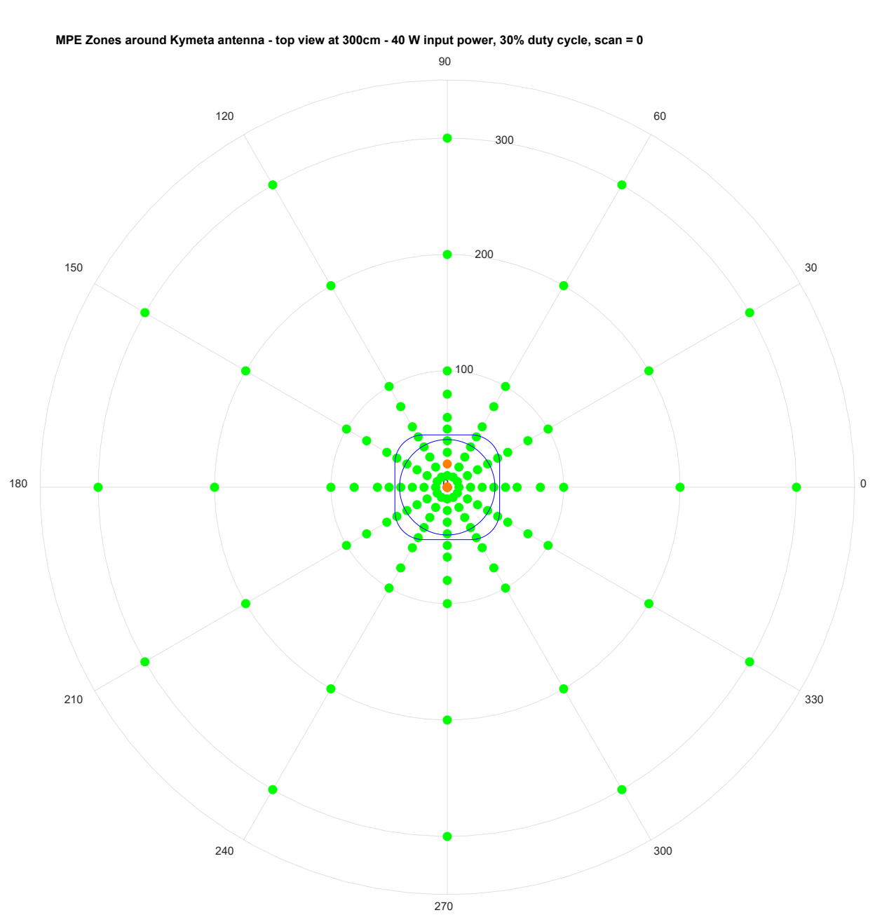
Figure 13: Height 300 cm, 40 W with 30% Duty Cycle, Scan 0 degrees
