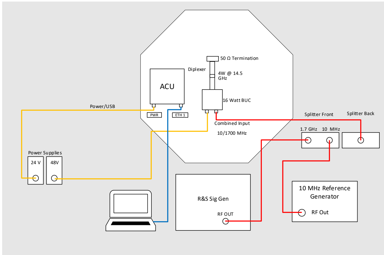
Figure 4: Kymeta terminal - transmit diagram
