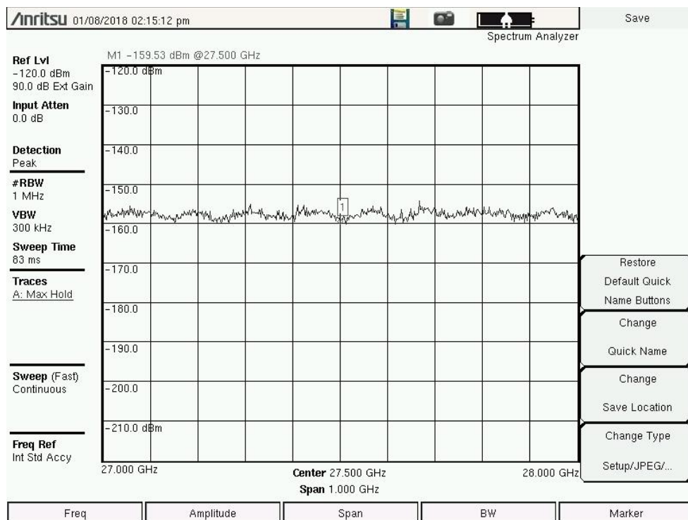
Figure 3.1-7 (C) Spectrum Photos 27-28 GHz 1MHz Res BW Vertical Pol 360°
