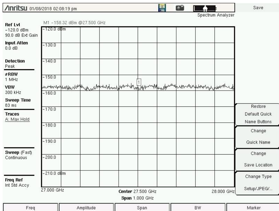
Figure 3.1-7 (A) Spectrum Photos 27-28 GHz 1MHz Res BW Horizontal Pol 360°
