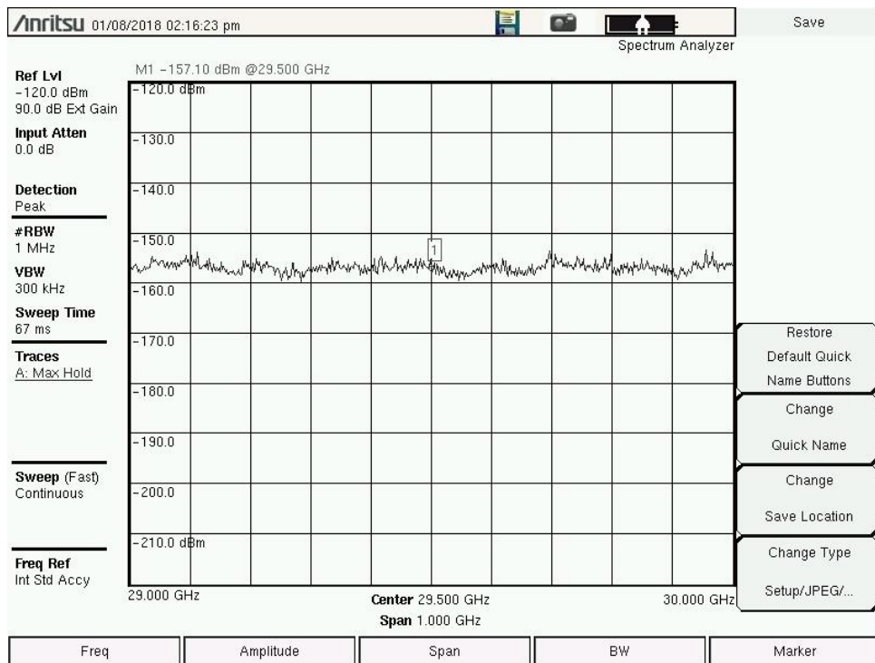
Figure 3.1-9 (C) Spectrum Photos 29-30 GHz 1MHz Res BW Vertical Pol 360°
