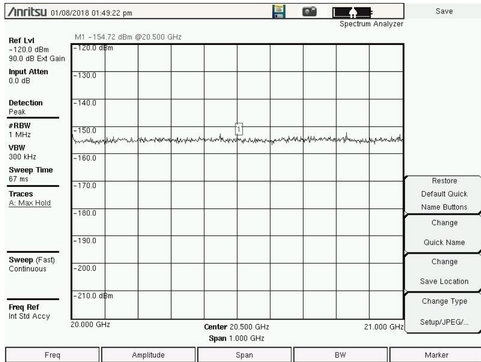
Figure 3.1-6 (G) Spectrum Photos 20-21 GHz 1MHz Res BW Vertical Pol Worst Case 225° Azimuth
