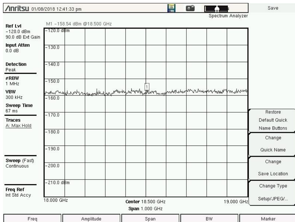
Figure 3.1-4 (A) Spectrum Photos 18-19 GHz 1 MHz Res BW Horizontal Pol 360°
