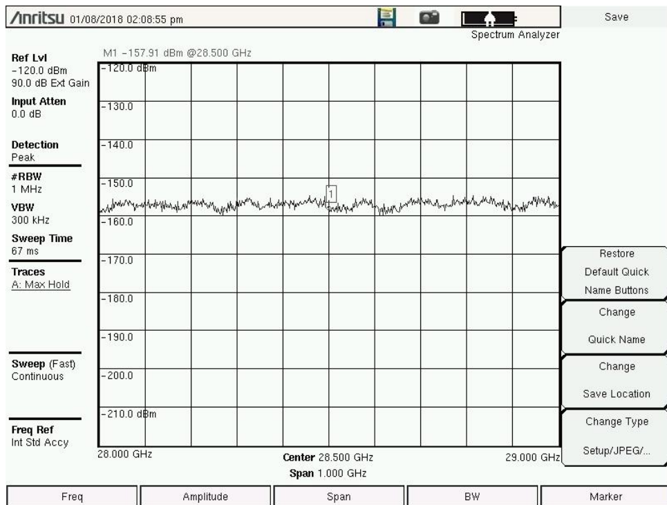
Figure 3.1-8 (C) Spectrum Photos 28-29 GHz 1MHz Res BW Vertical Pol 360°
