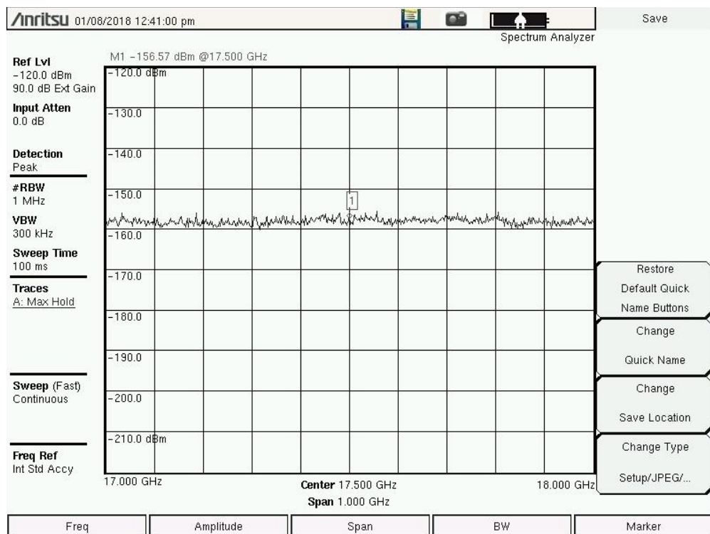
Figure 3.1-3 (A) Spectrum Photos 17-18 GHz 1MHz Res BW Horizontal Pol 360°
