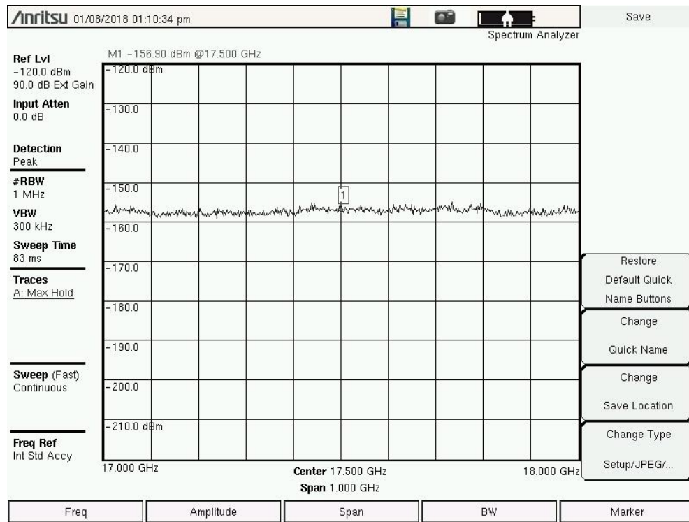
Figure 3.1-3 (C) Spectrum Photos 17-18 GHz 1 MHz Res BW Horizontal Pol Worst Case 225° Azimuth
