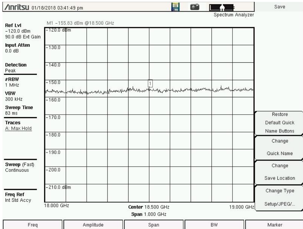
Figure 3.1-4 (C) Spectrum Photos 18-19 GHz 1 MHz Res BW Horizontal Pol Worst Case 130 degrees
