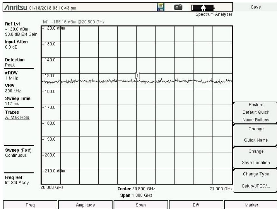
Figure 3.1-6 (G) Spectrum Photos 20-21 GHz 1MHz Res BW Vertical Pol Worst Case 130 degrees
