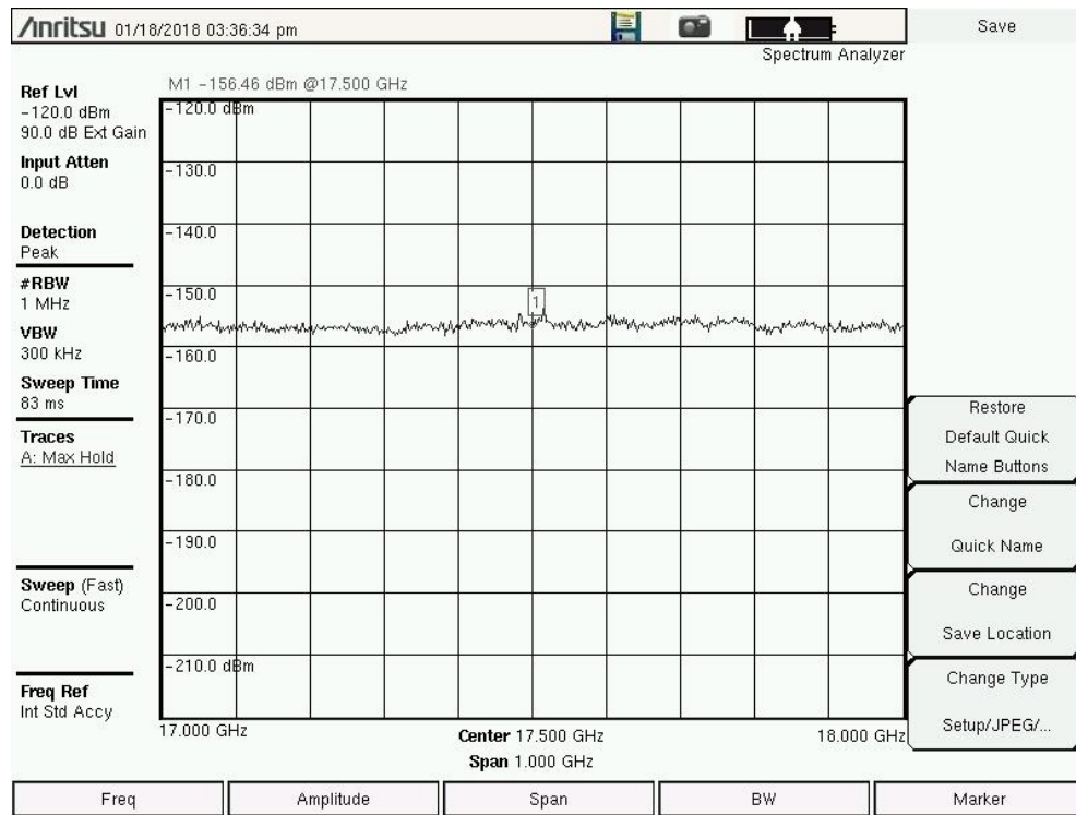
Figure 3.1-3 (C) Spectrum Photos 17-18 GHz 1 MHz Res BW Horizontal Pol Vertical Pol
