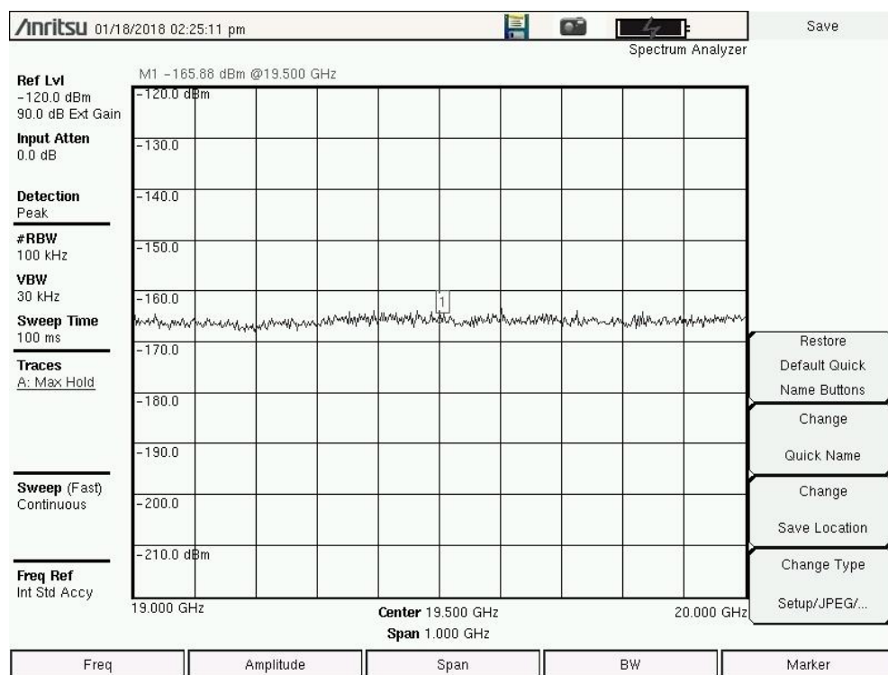
Figure 3.1-5 (B) Spectrum Photos 19-20 GHz 100 kHz Res BW Horizontal Pol 360°
