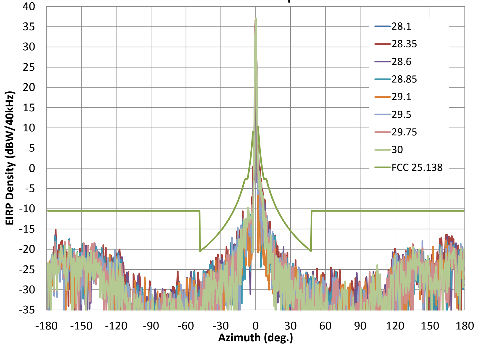
SatLite- Tx RHCP Azimuth Co-pol Patterns
