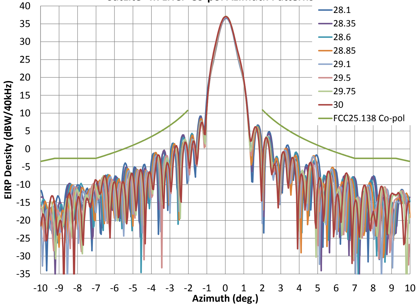
SatLite- Tx LHCP Co-pol Azimuth Patterns
