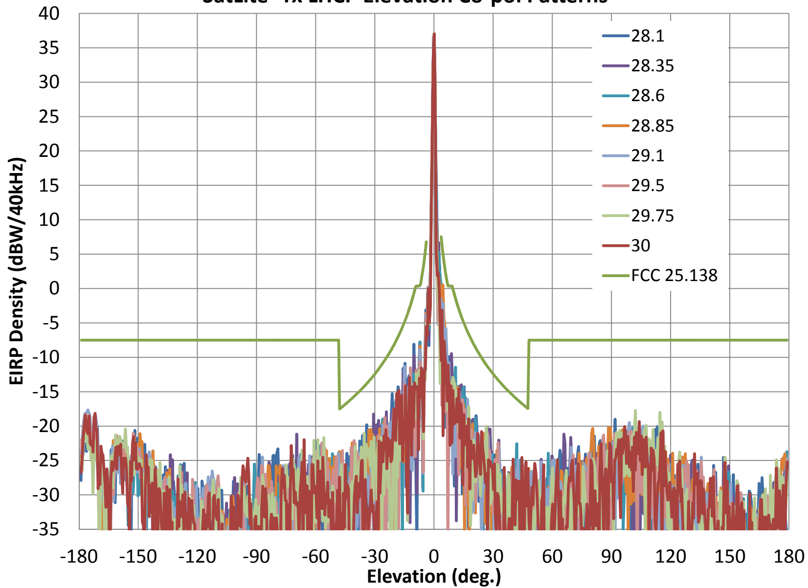
SatLite- Tx LHCP Elevation Co-pol Patterns
