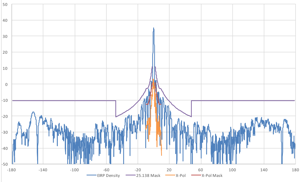
29.1 GHz RHCP EIRP Density Plots
