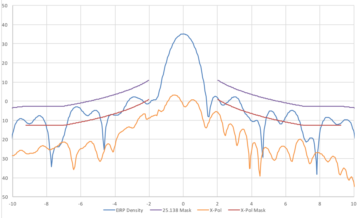
29.1 GHz EIRP Density Plots
