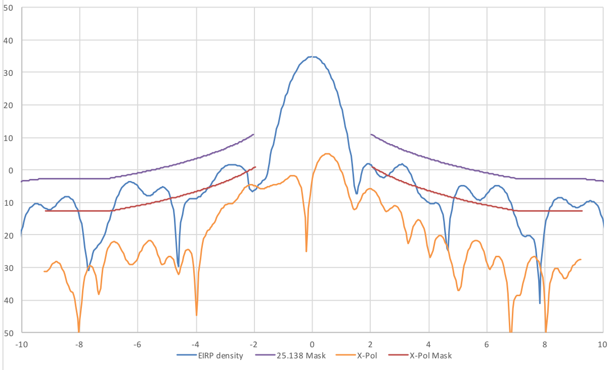
29.1 GHz EIRP Density Plots
