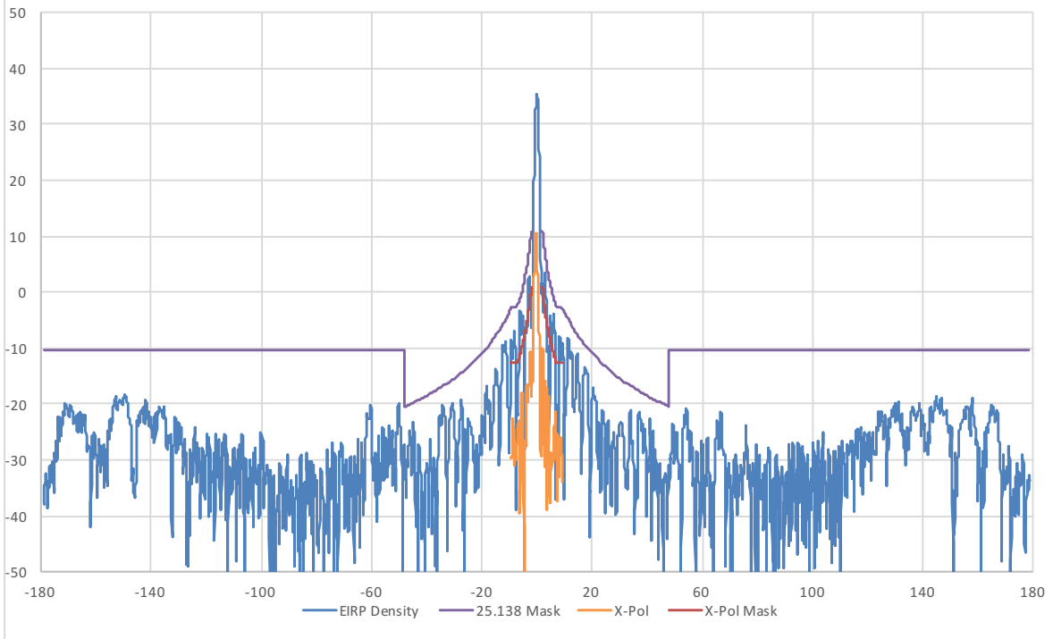
30 GHz Az RHCP EIRP Density Plots
