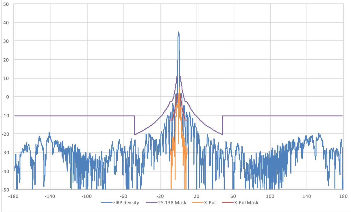
29.1 GHz LHCP EIRP Density Plots
