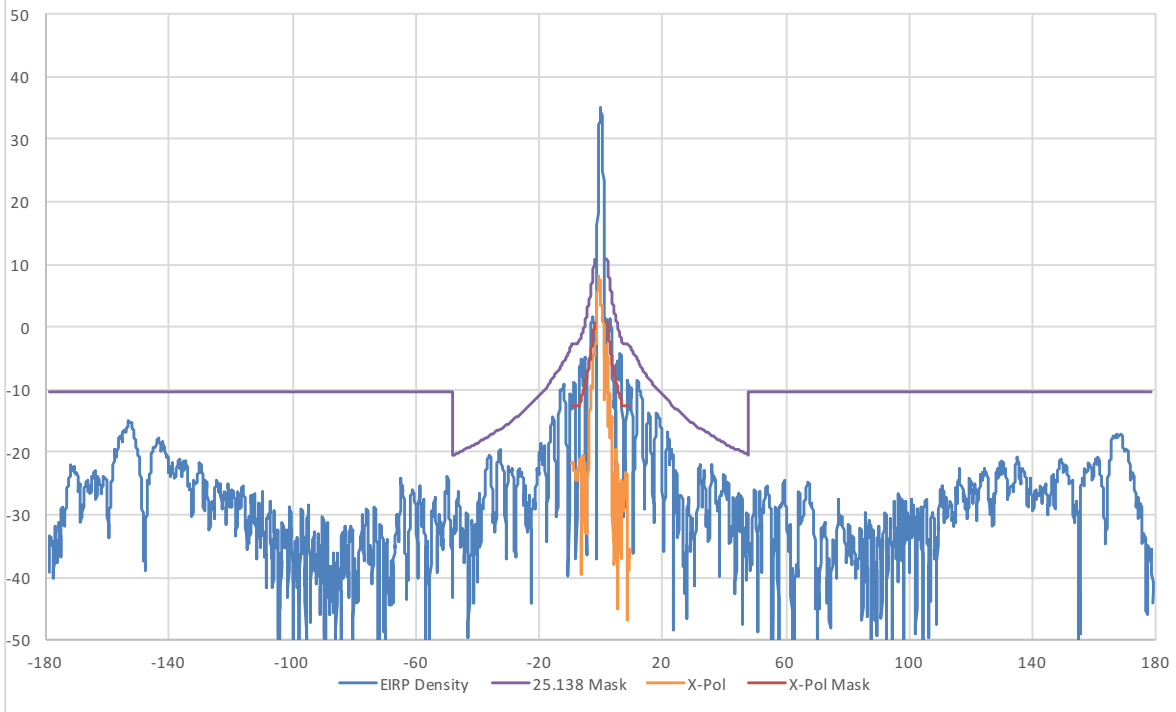
28.35 GHz Az RHCP EIRP Density Plots
