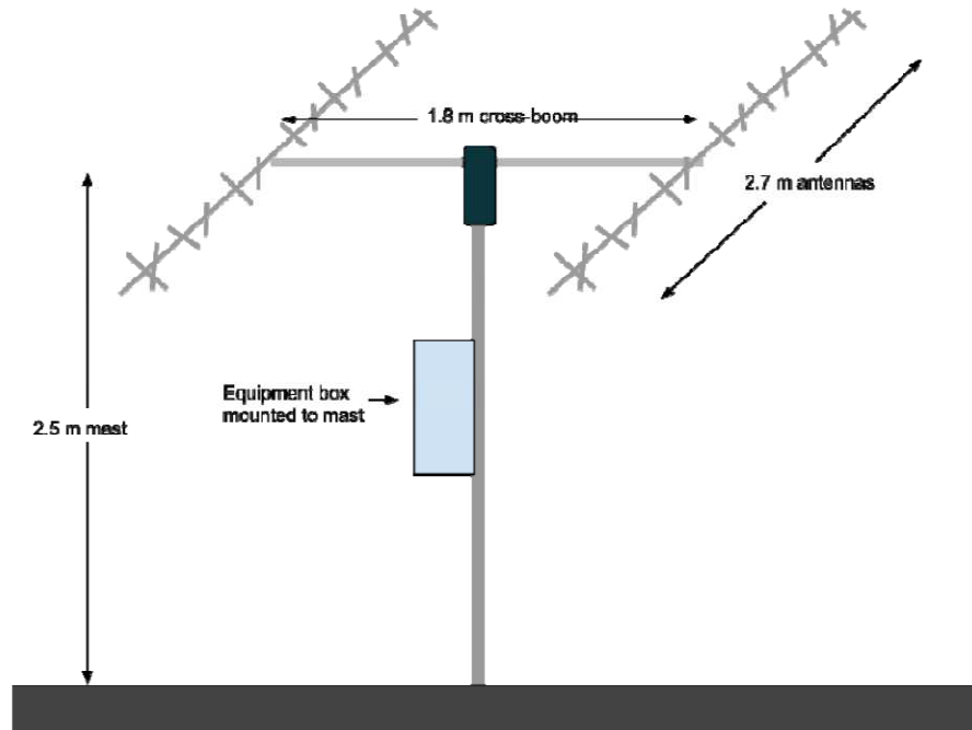
Figure 1 UHF earth station diagram
