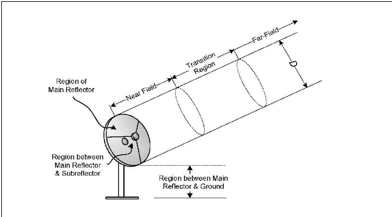
Figure 1. EM Fields as a Function of Distance
