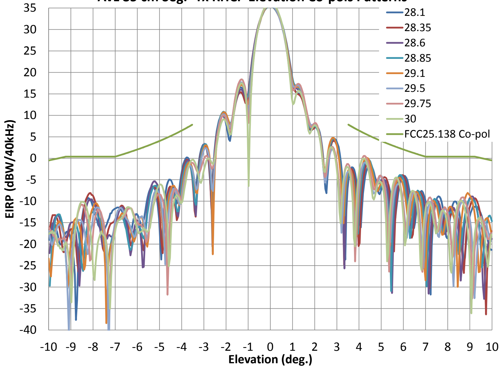
AvL 85 cm Seg.- Tx RHCP Elevation Co-pols Patterns
