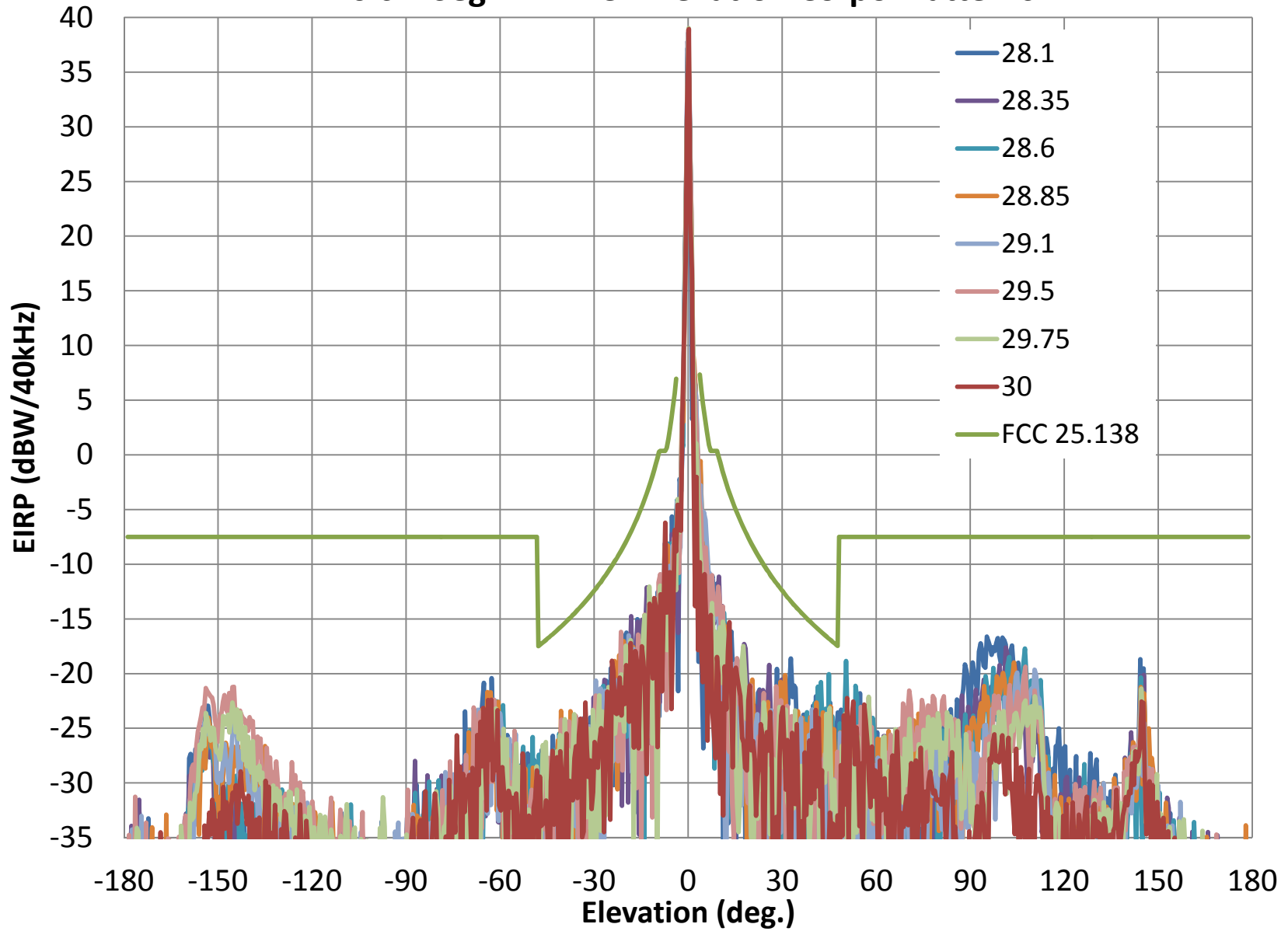
AvL 120 cm Seg.- Tx LHCP Elevation Co-pol Patterns
