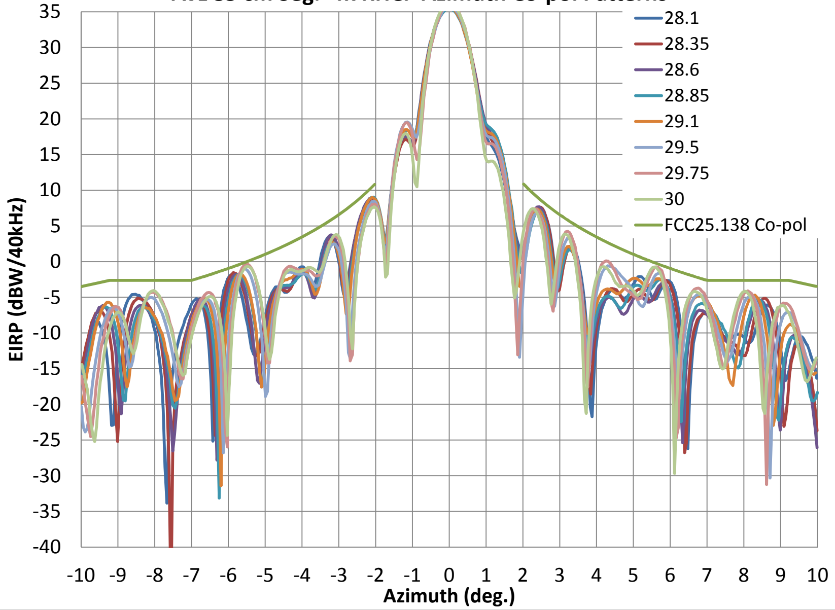
AvL 85 cm Seg.- Tx RHCP Azimuth Co-pol Patterns
