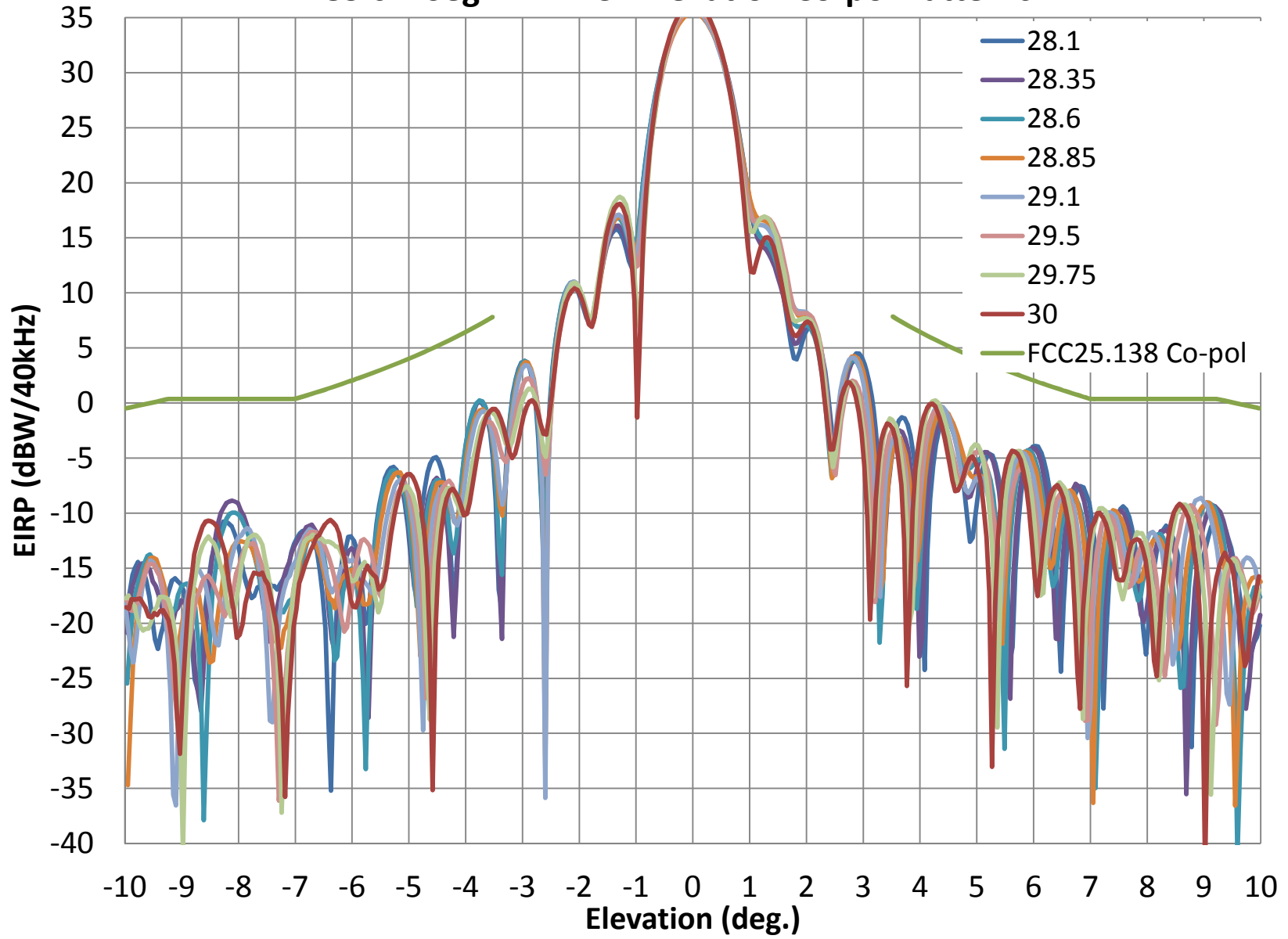
AvL 85 cm Seg.- Tx LHCP Elevation Co-pol Patterns
