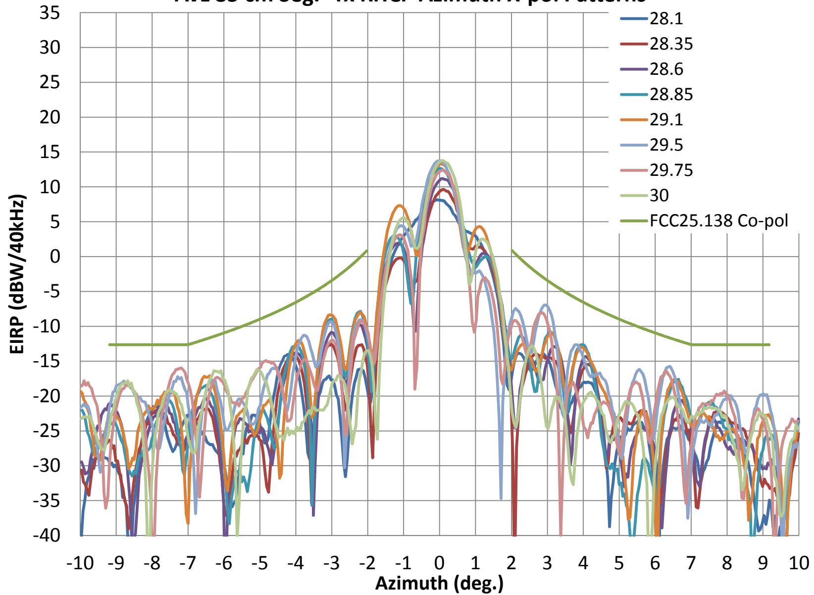
AvL 85 cm Seg.- Tx RHCP Azimuth X-pol Patterns
