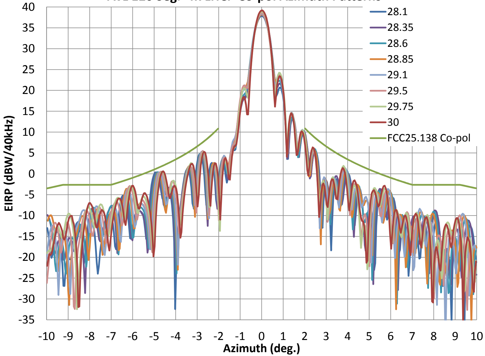
AvL 120 Seg.- Tx LHCP Co-pol Azimuth Patterns
