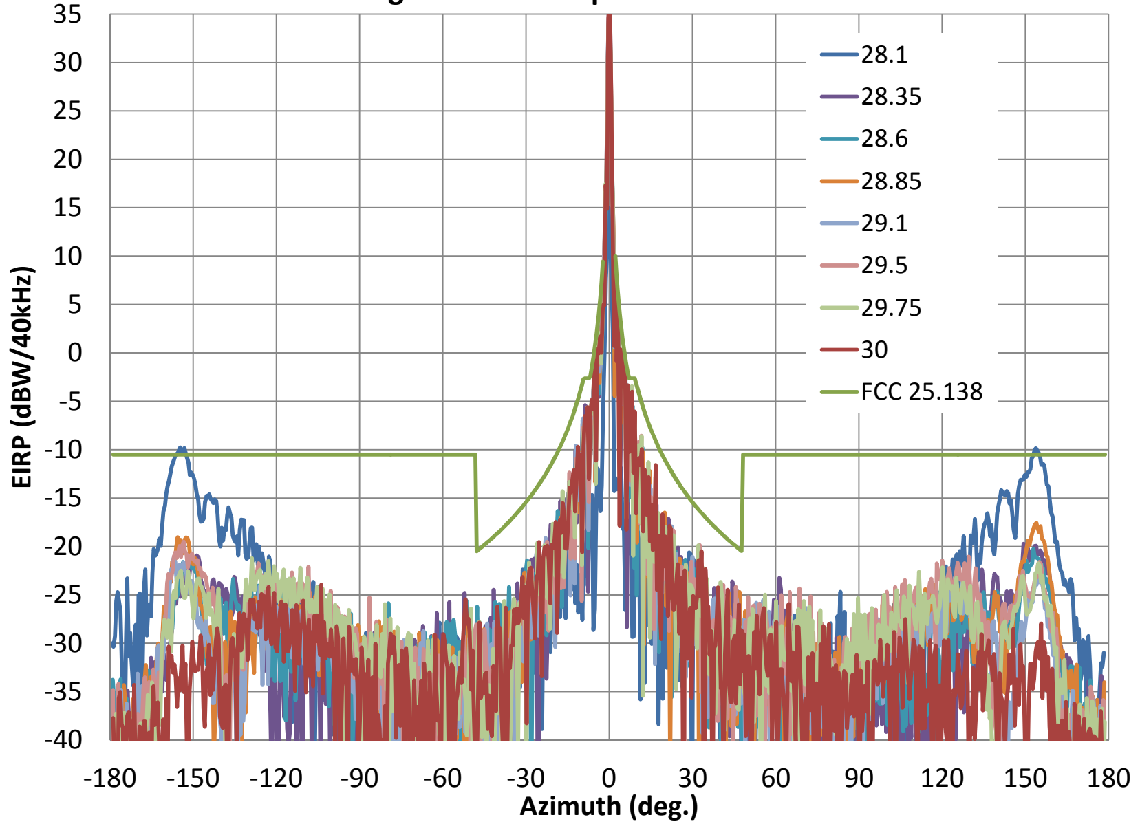
AvL 85 Seg.- Tx LHCP Co-pol Azimuth Patterns
