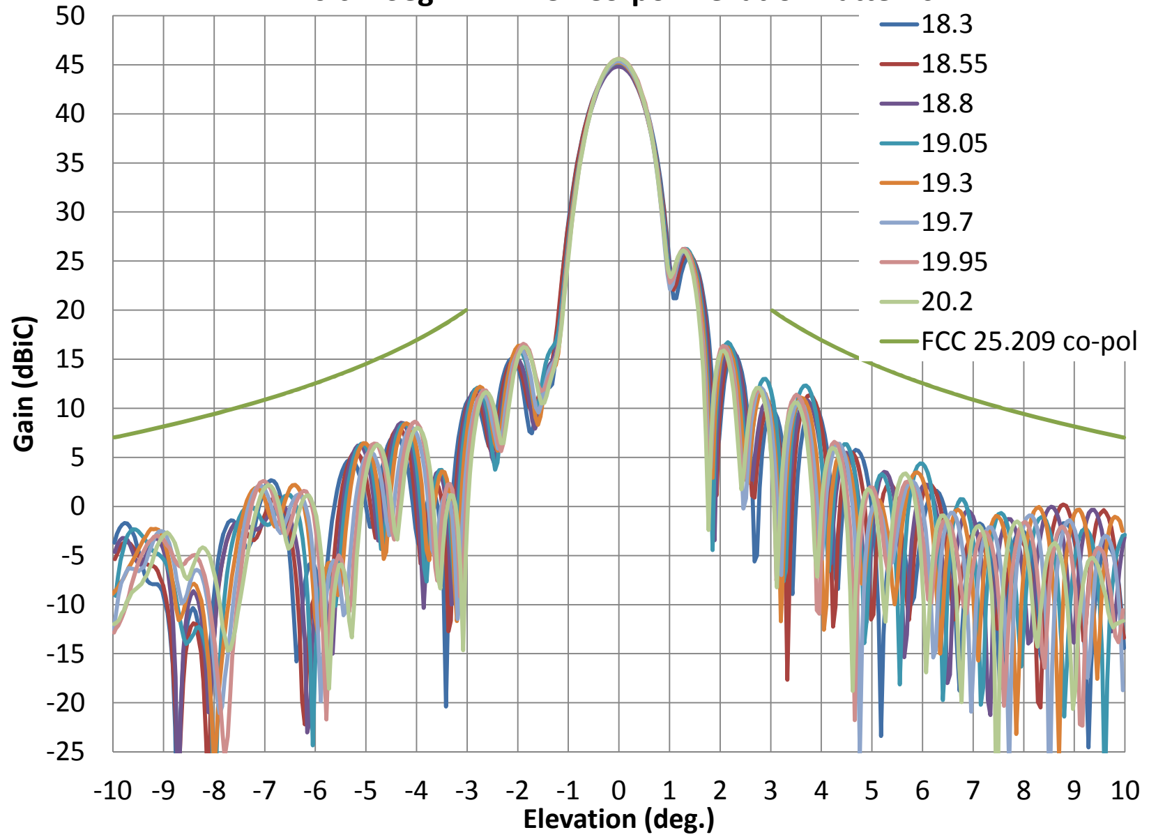
AvL 120 cm Seg.- Rx RHCP Co-pol Elevation Patterns
