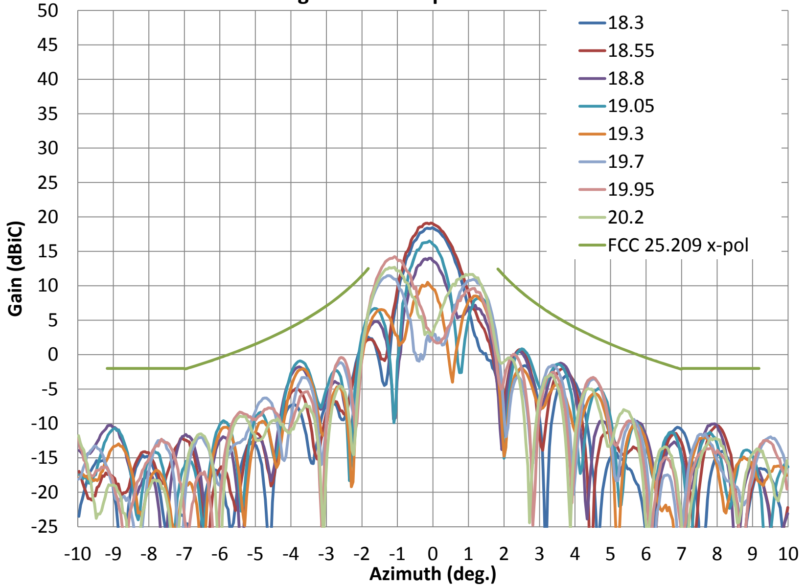
AvL 85 cm Seg.- Rx LHCP X-pol Azimuth Patterns
