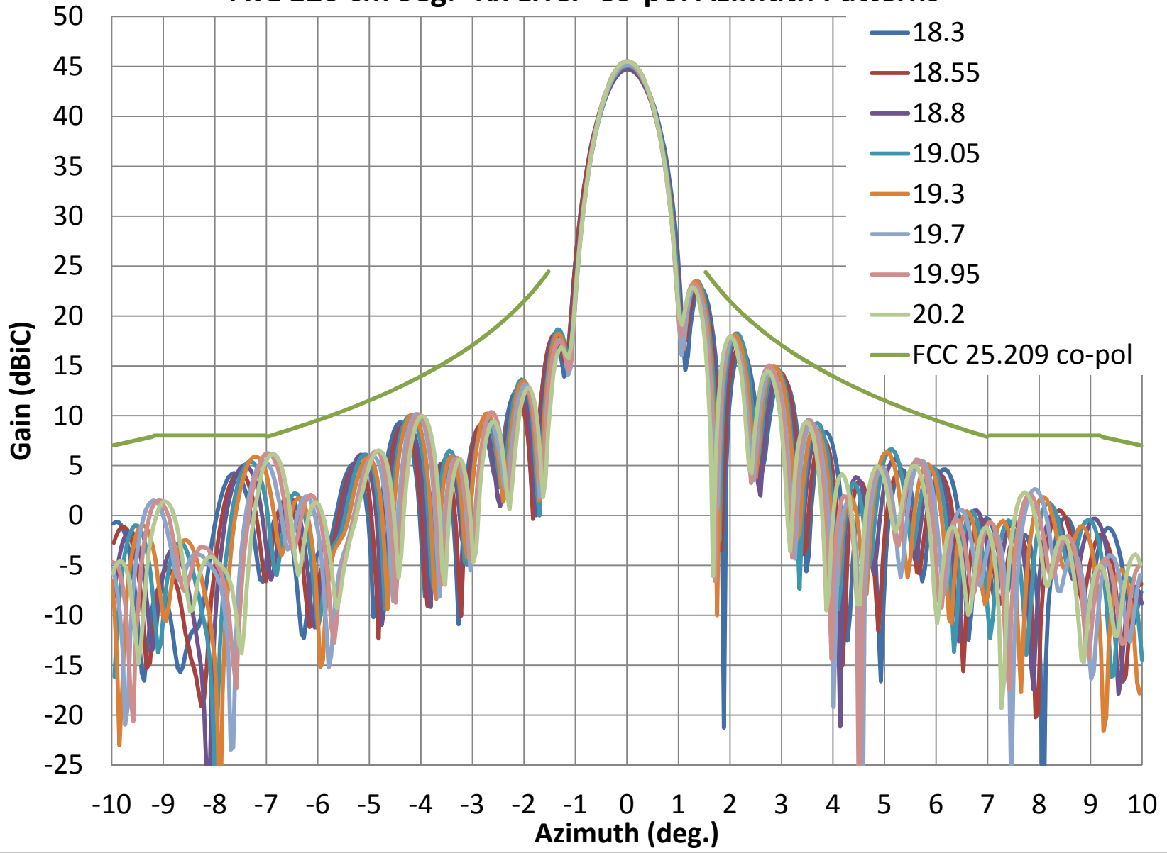
AvL 120 cm Seg.- Rx LHCP Co-pol Azimuth Patterns
