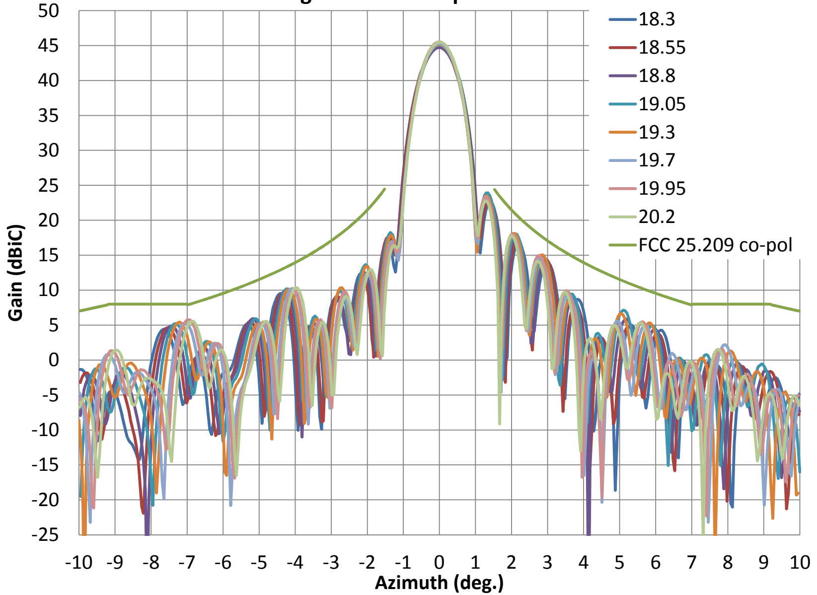
AvL 120 cm Seg.- Rx RHCP Co-pol Azimuth Patterns
