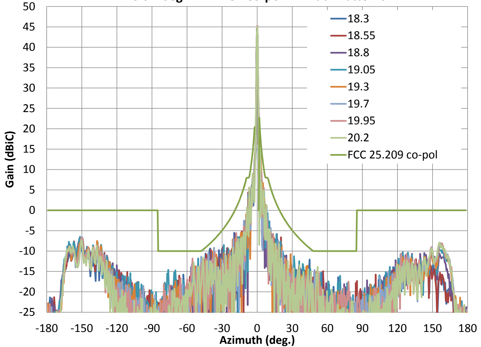
AvL 120 cm Seg.- Rx RHCP Co-pol Azimuth Patterns
