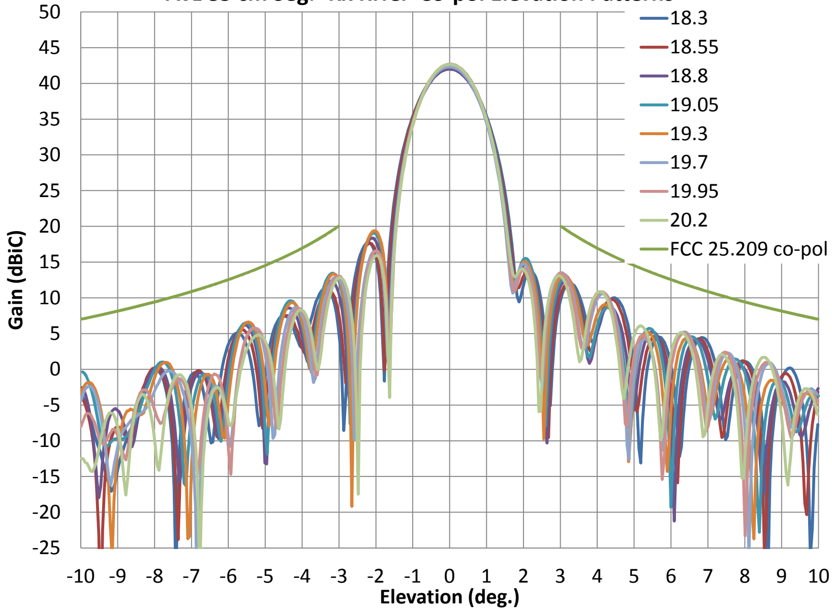
AvL 85 cm Seg.- Rx RHCP Co-pol Elevation Patterns
