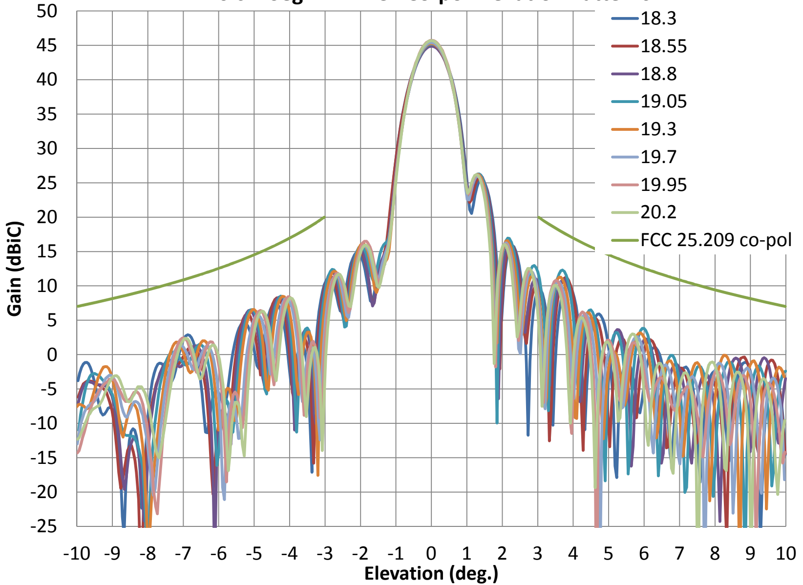
AvL 120 cm Seg.- Rx LHCP Co-pol Elevation Patterns
