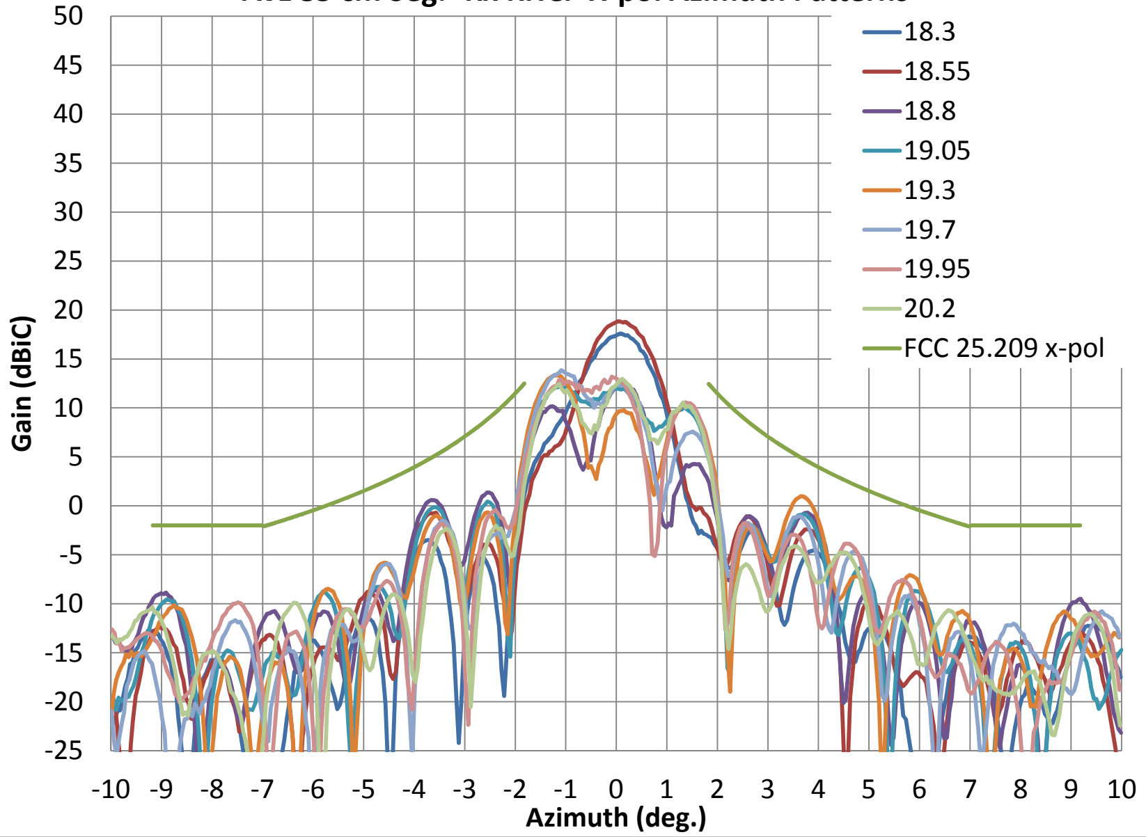
AvL 85 cm Seg.- Rx RHCP X-pol Azimuth Patterns
