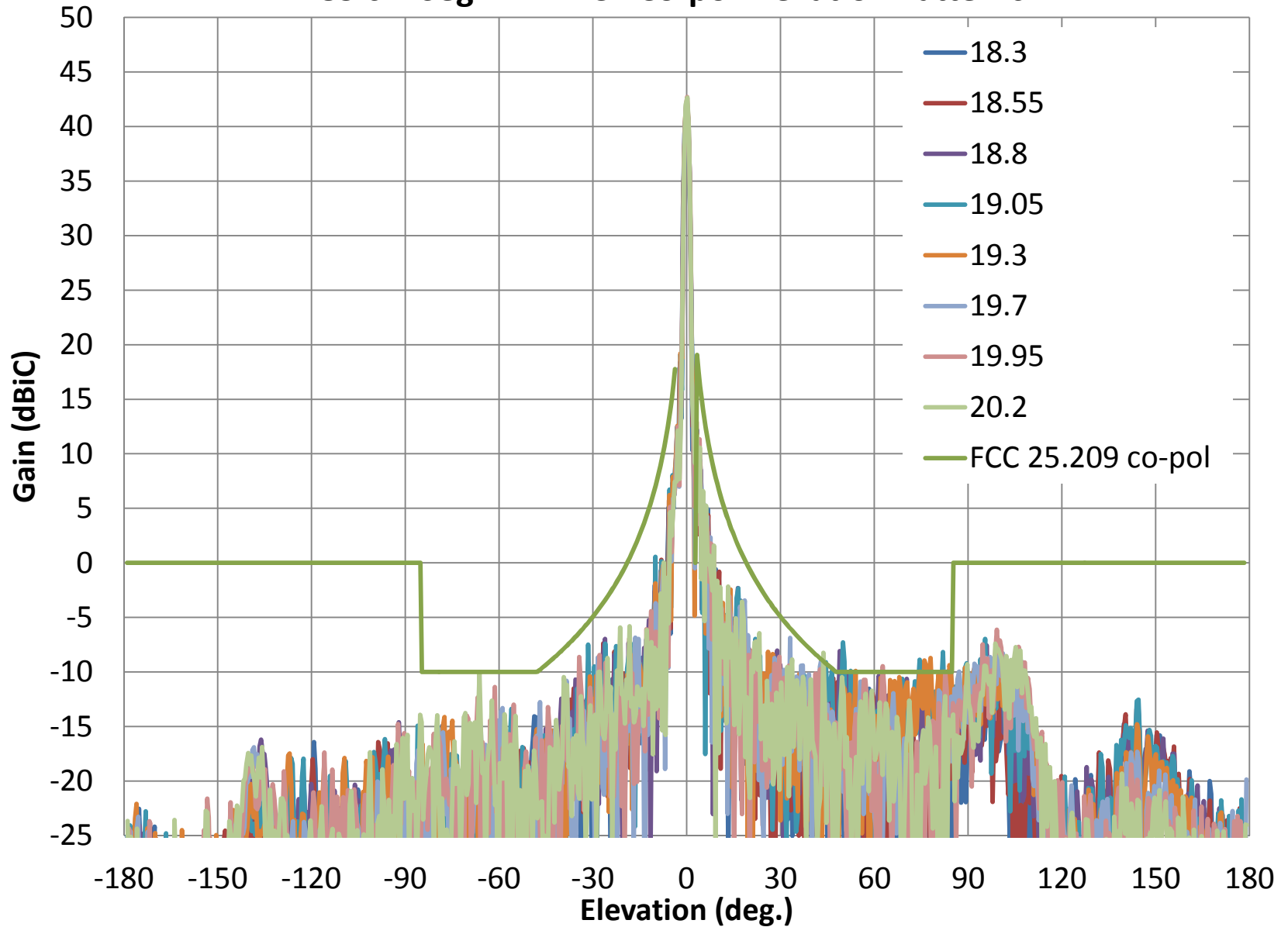
AvL 85 cm Seg.- Rx LHCP Co-pol Elevation Patterns
