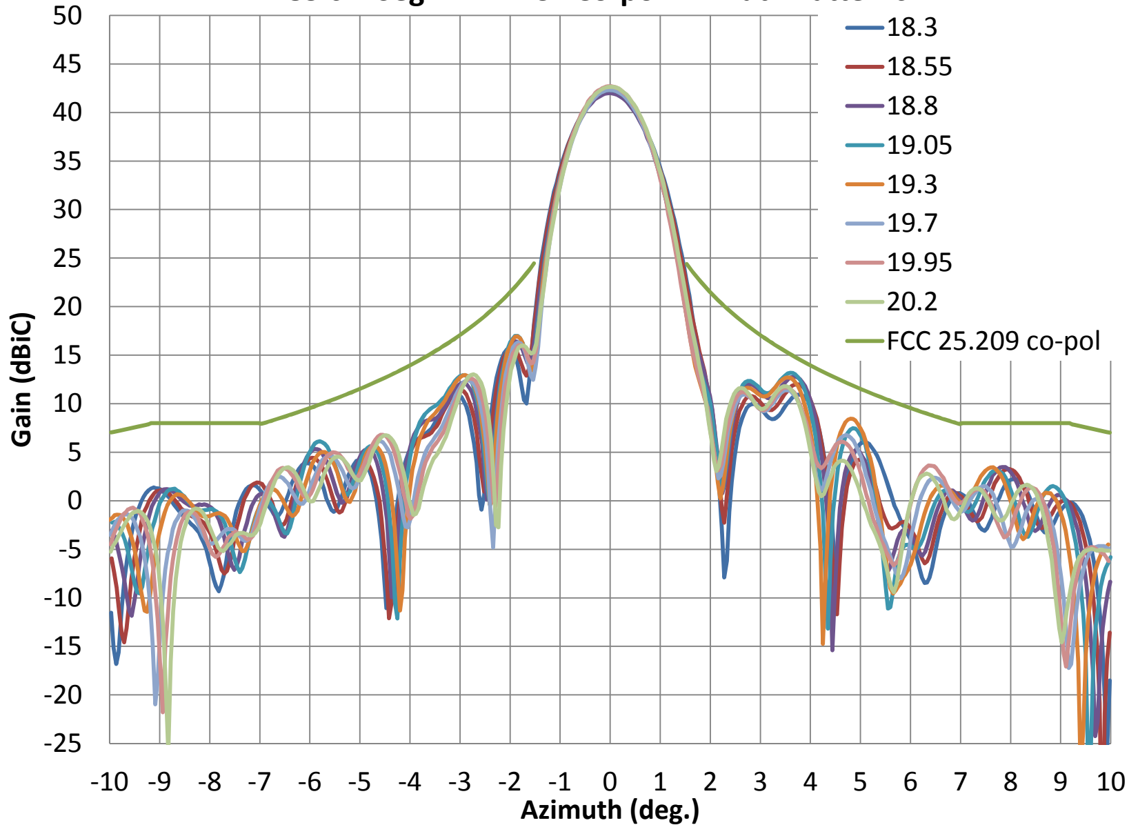
AvL 85 cm Seg.- Rx RHCP Co-pol Azimuth Patterns
