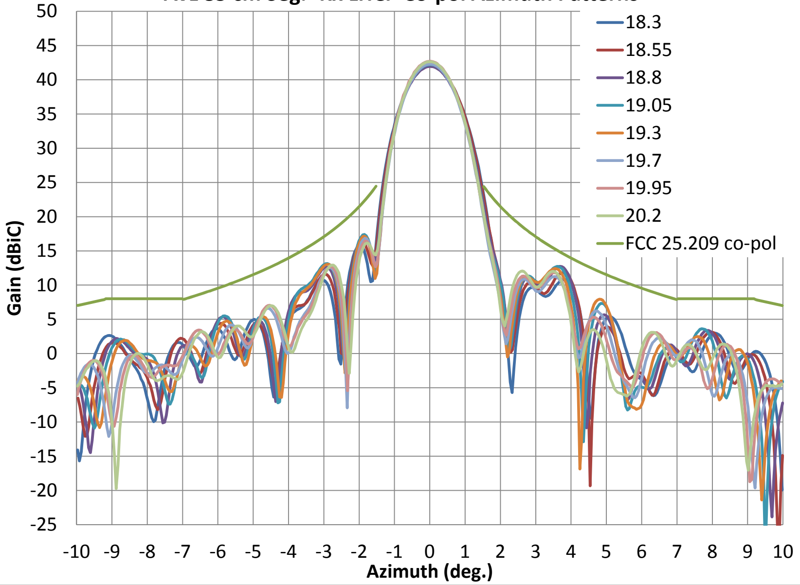
AvL 85 cm Seg.- Rx LHCP Co-pol Azimuth Patterns
