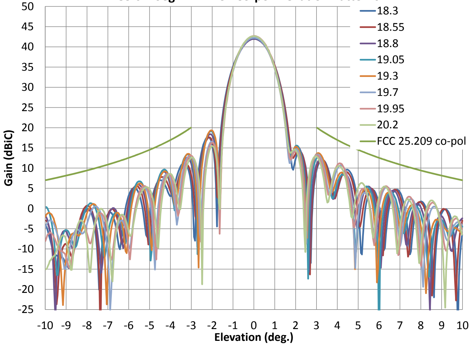
AvL 85 cm Seg.- Rx LHCP Co-pol Elevation Patterns
