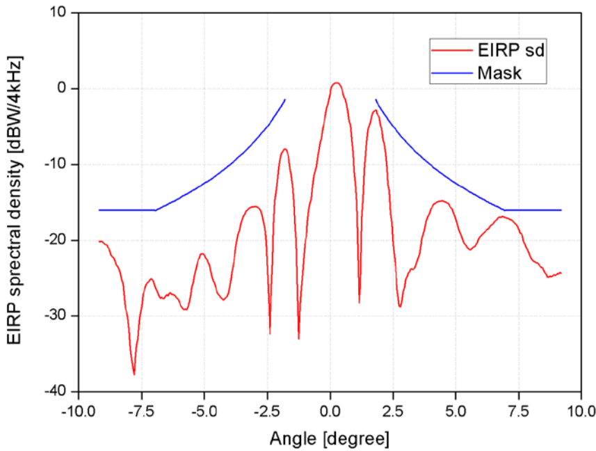
14.25GHz EIRP spectral density @ -13.82 dBW/4kHz Input power spectral density
