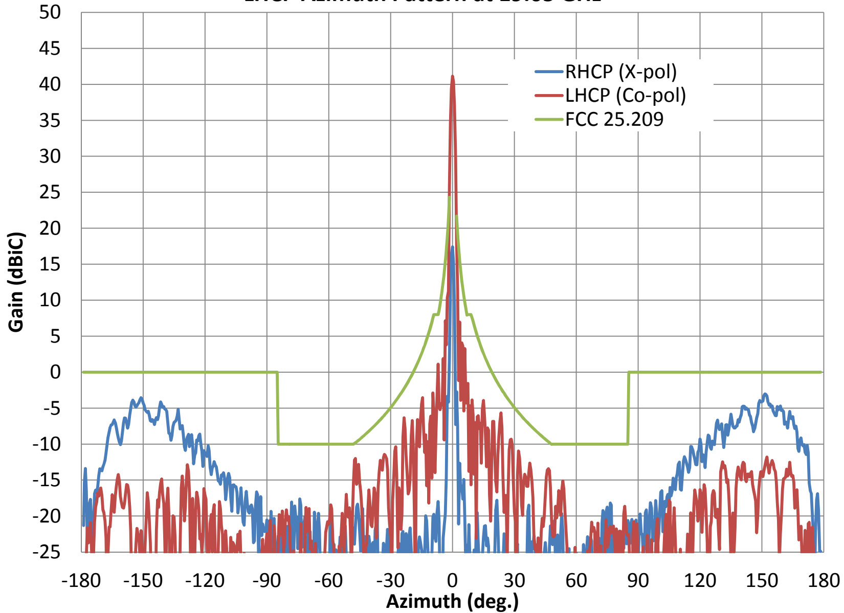
LHCP Azimuth Pattern at 19.05 GHz
