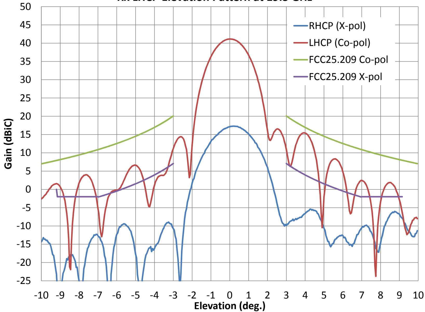
Rx LHCP Elevation Pattern at 19.3 GHz
