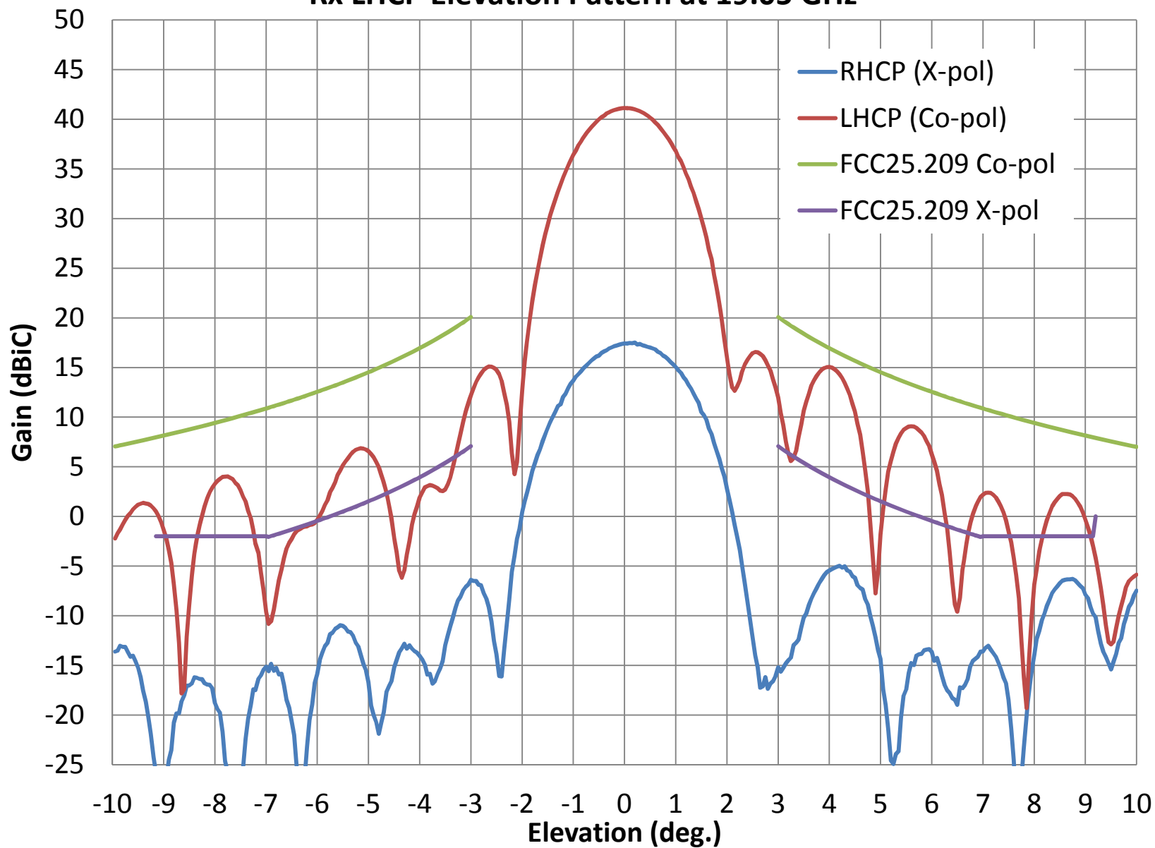
Rx LHCP Elevation Pattern at 19.05 GHz
