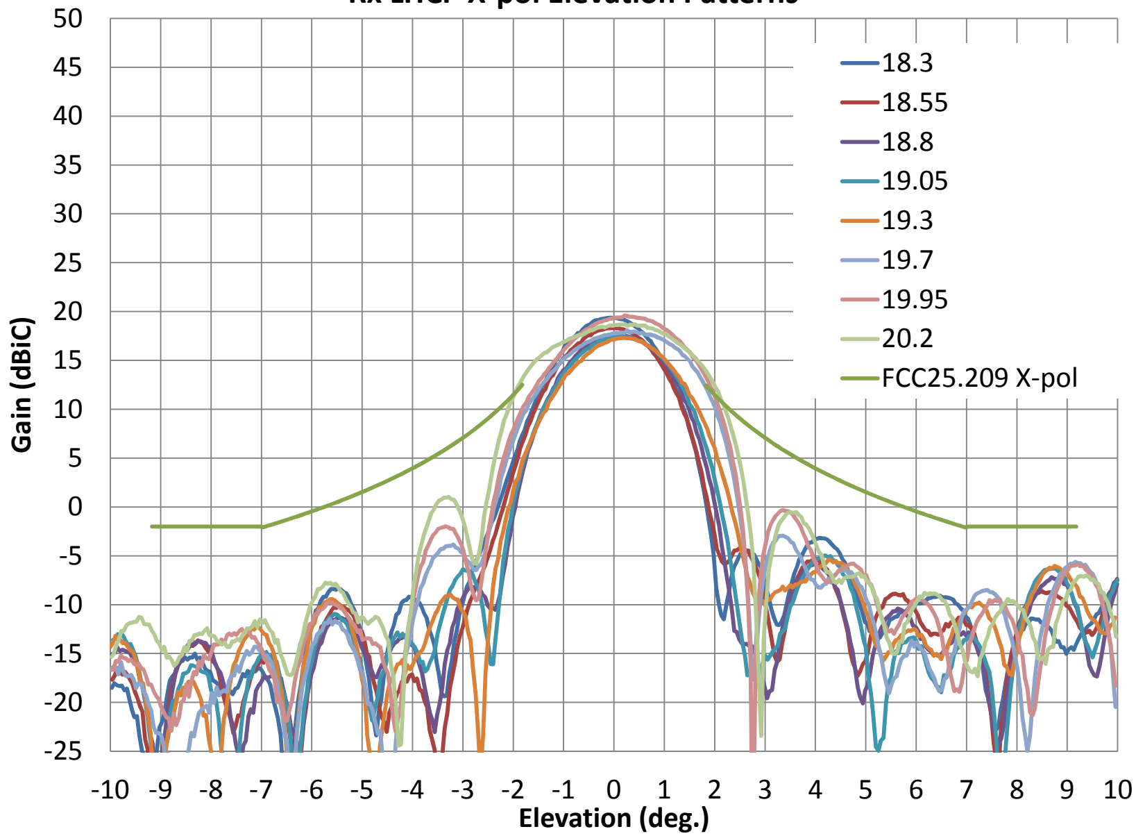
Rx LHCP X-pol Elevation Patterns
