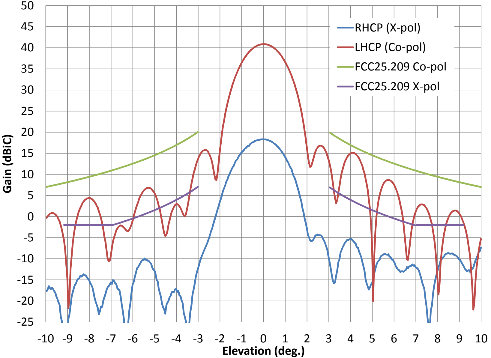
Rx LHCP Elevation Pattern at 18.55 GHz
