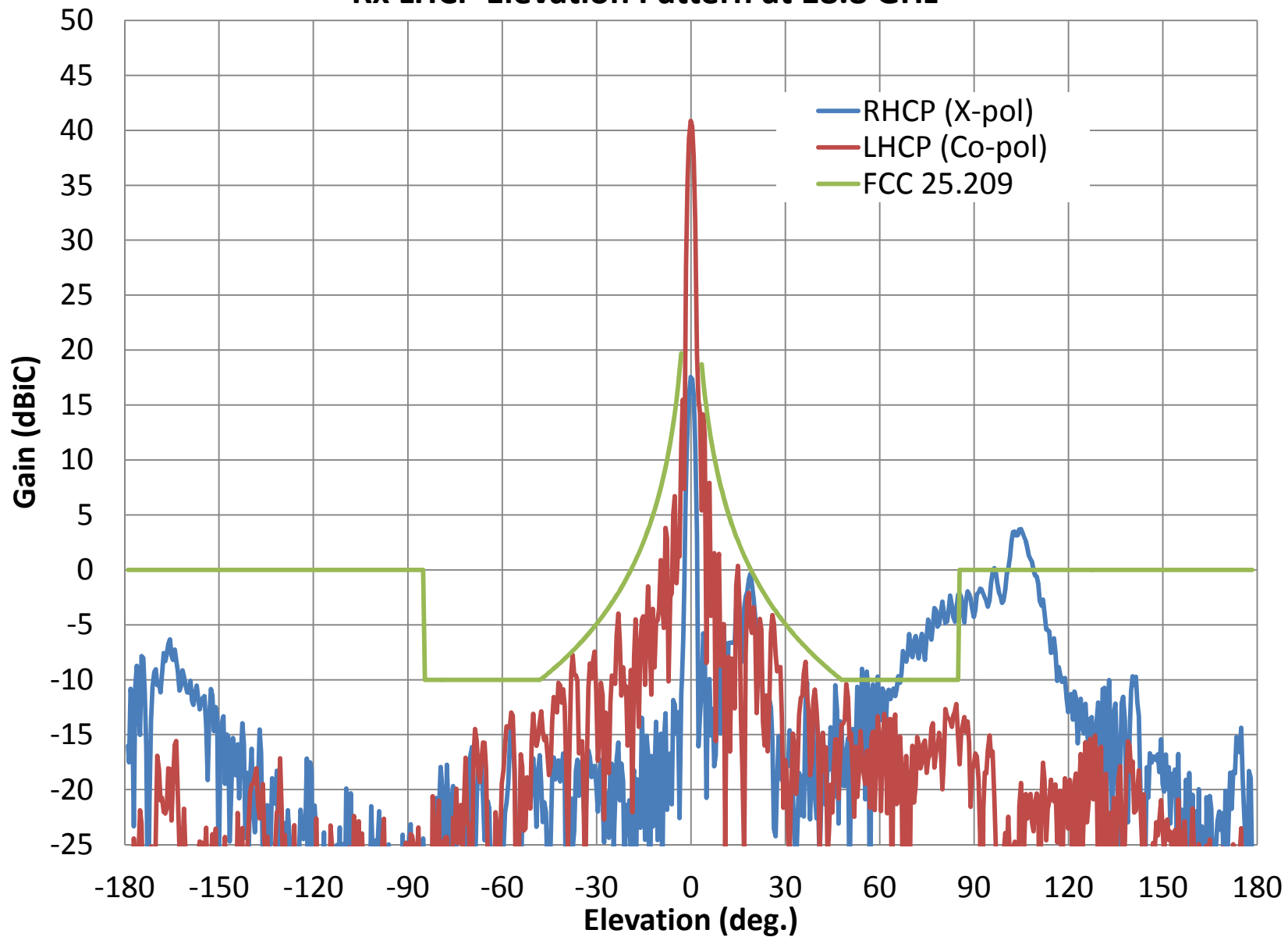
Rx LHCP Elevation Pattern at 18.8 GHz
