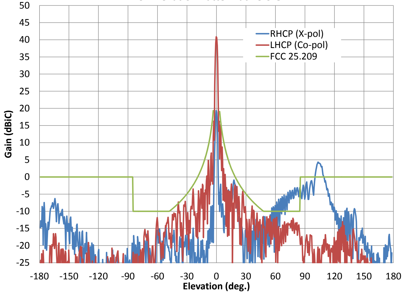
Rx LHCP Elevation Pattern at 18.3 GHz
