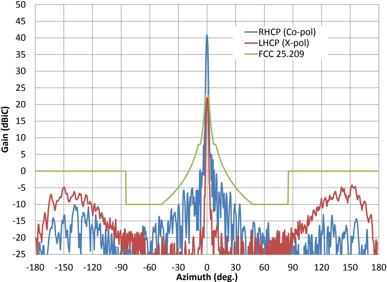
Rx RHCP Azimuth Pattern at 18.3 GHz
