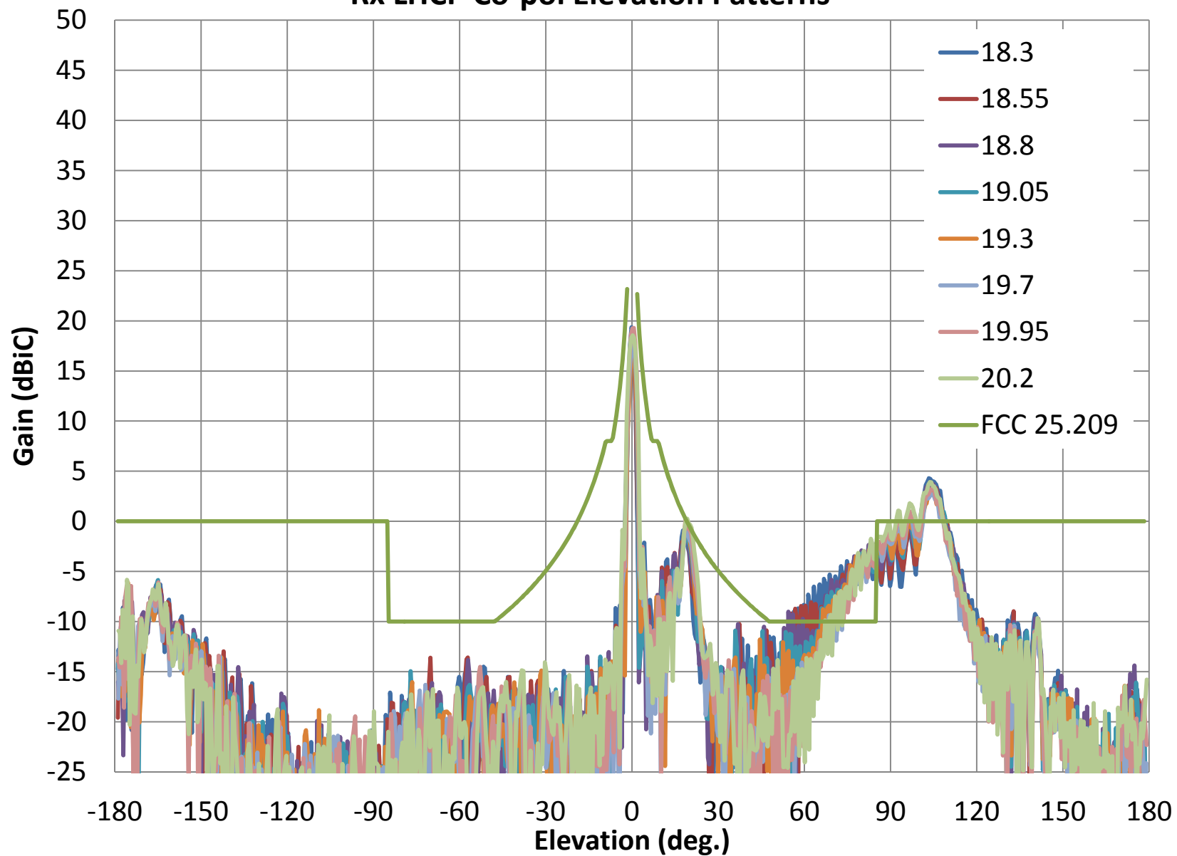
Rx LHCP Co-pol Elevation Patterns
