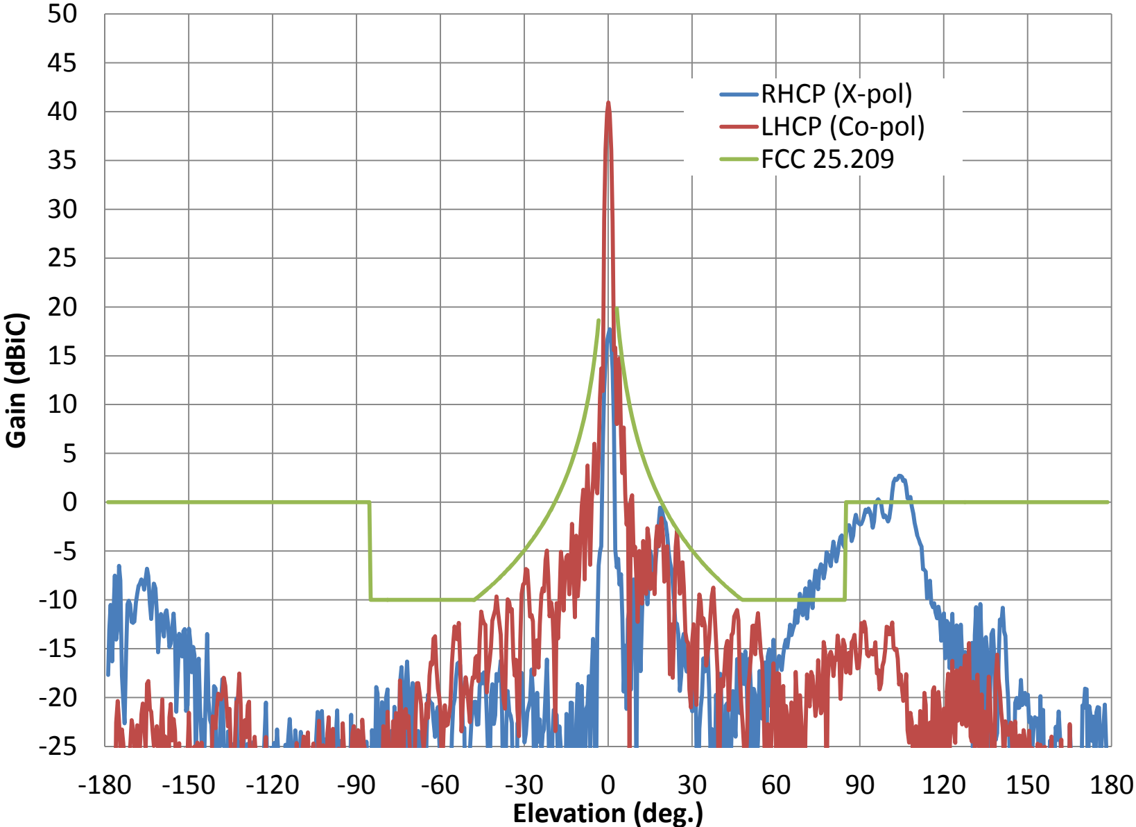
Rx LHCP Elevation Pattern at 19.7 GHz
