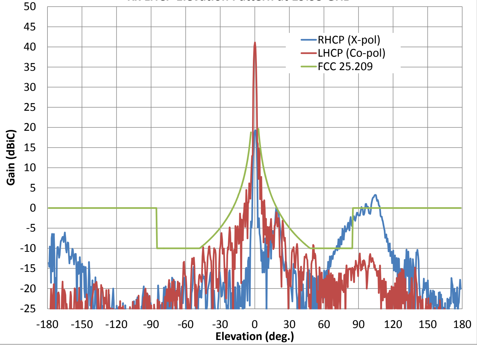
Rx LHCP Elevation Pattern at 19.95 GHz
