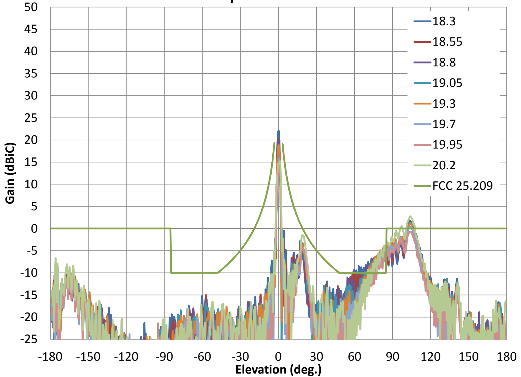
Rx RHCP Co-pol Elevation Patterns
