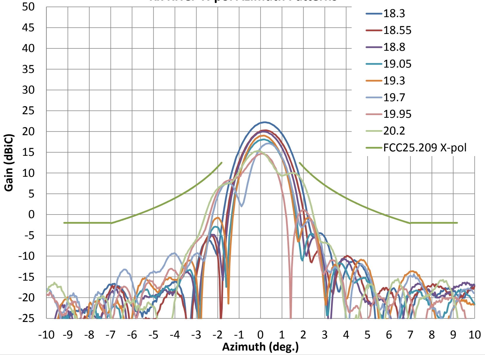
Rx RHCP X-pol Azimuth Patterns
