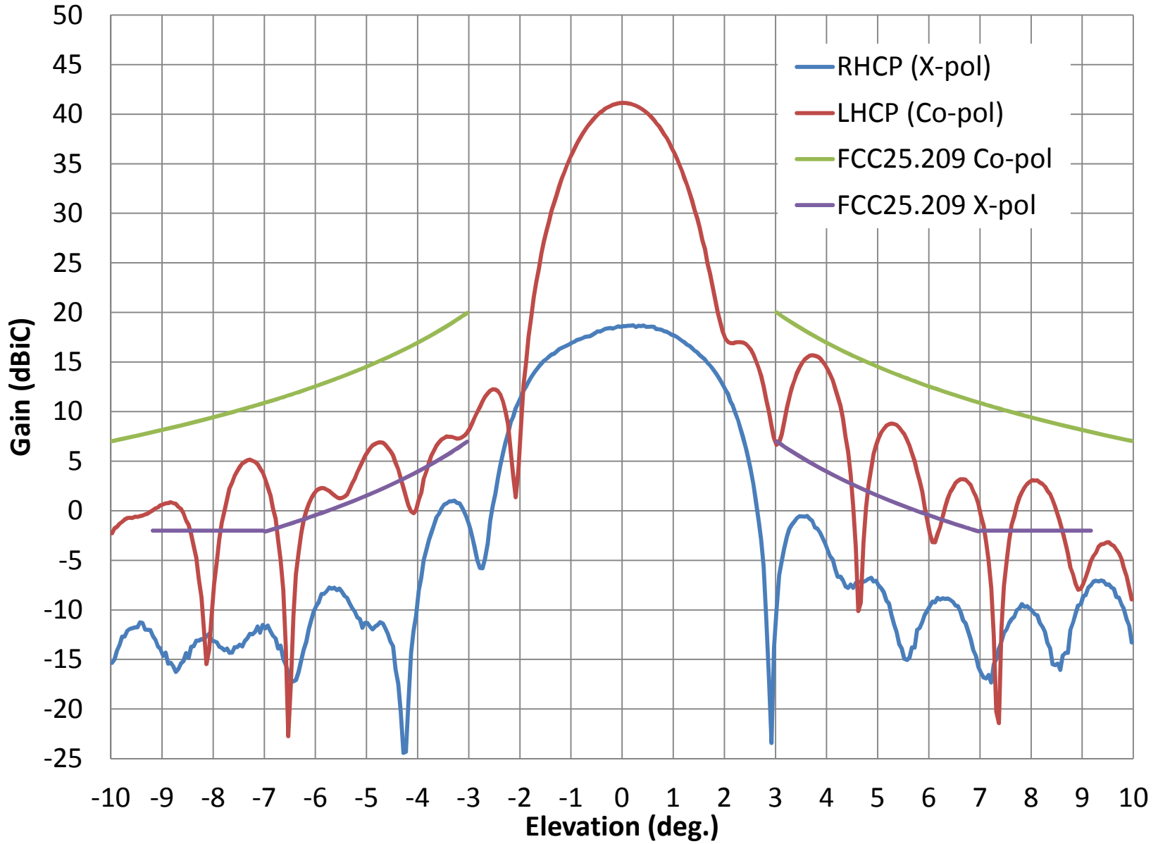
Rx LHCP Elevation Pattern at 20.2 GHz
