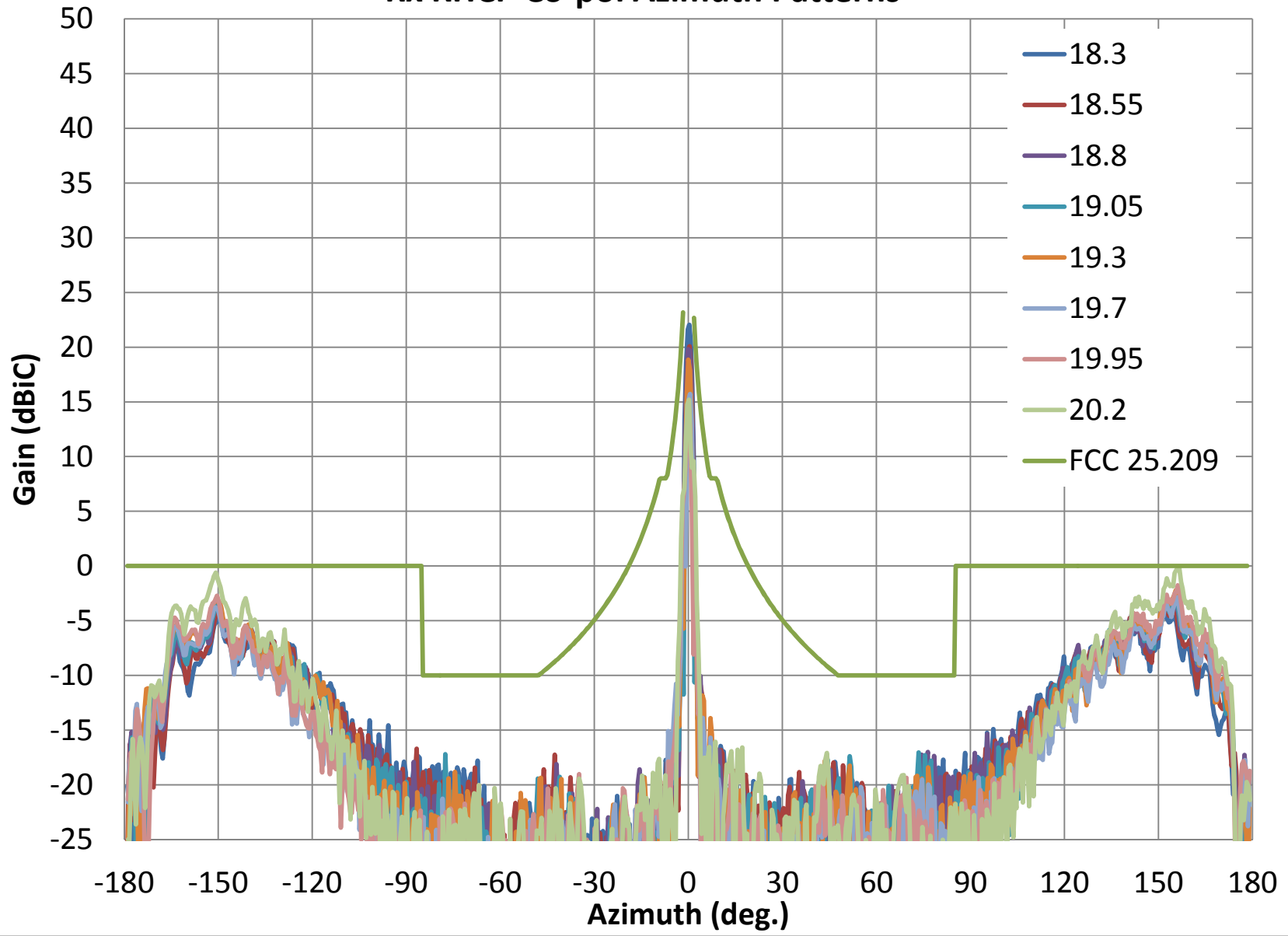
Rx RHCP Co-pol Azimuth Patterns
