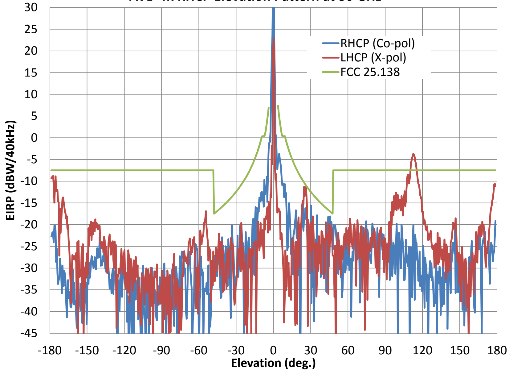
AVL- Tx RHCP Elevation Pattern at 30 GHz
