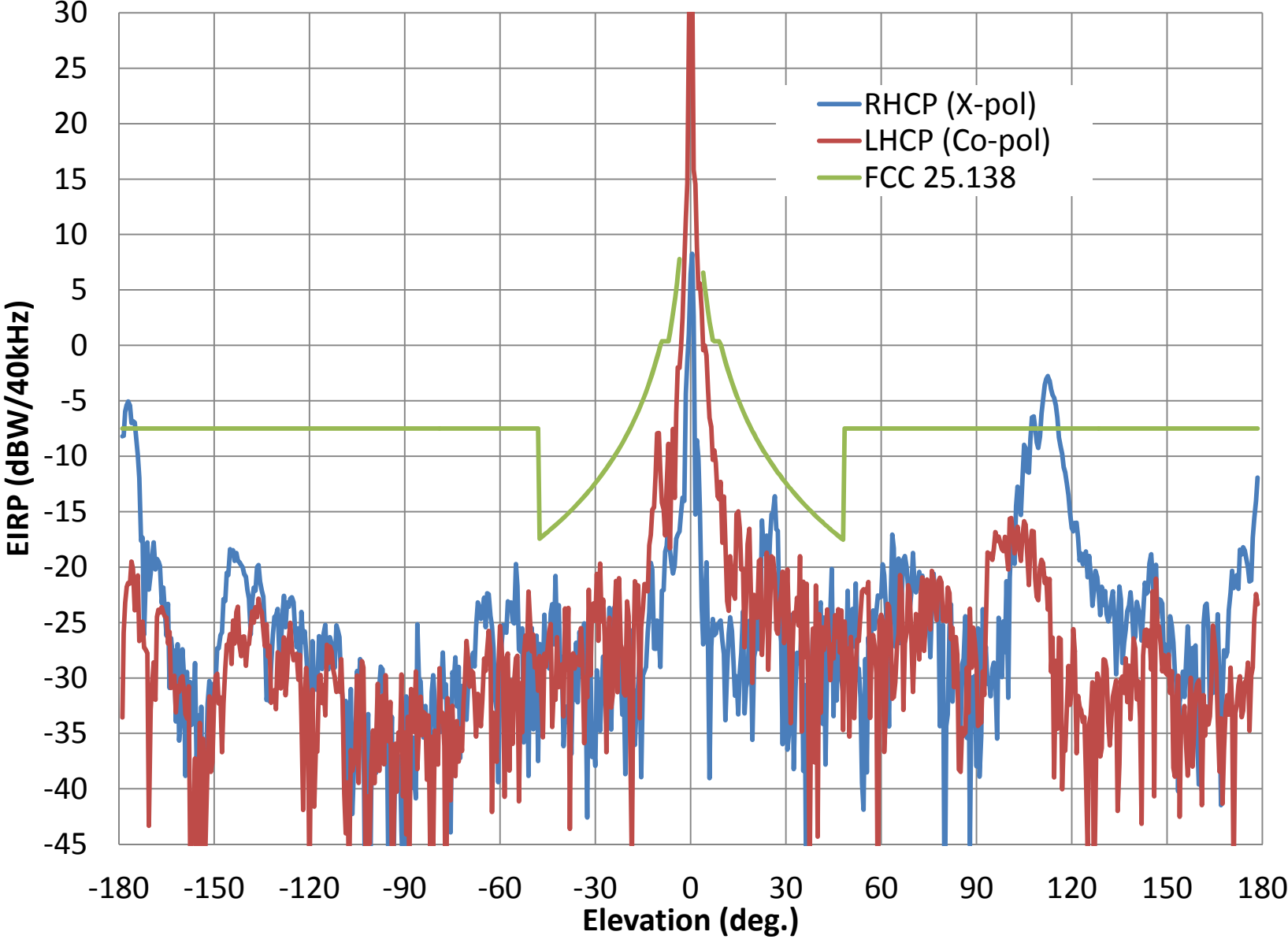
AVL- Tx LHCP Elevation Pattern at 28.85 GHz
