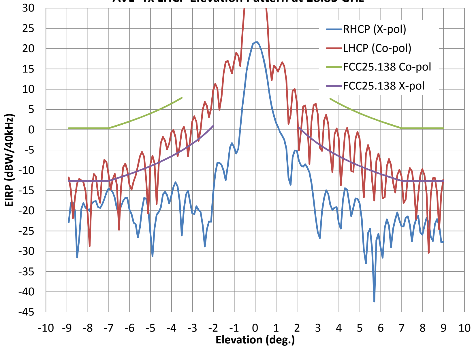
AVL- Tx LHCP Elevation Pattern at 28.85 GHz
