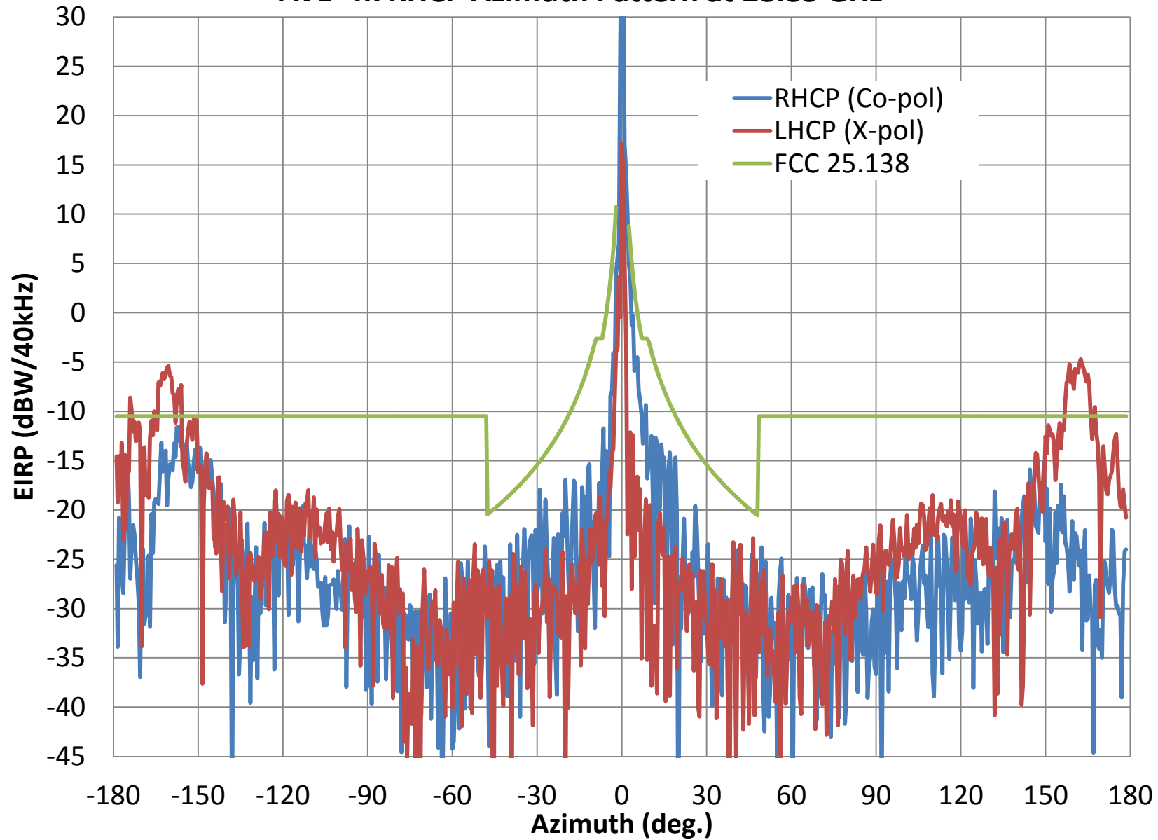
AVL- Tx RHCP Azimuth Pattern at 28.85 GHz
