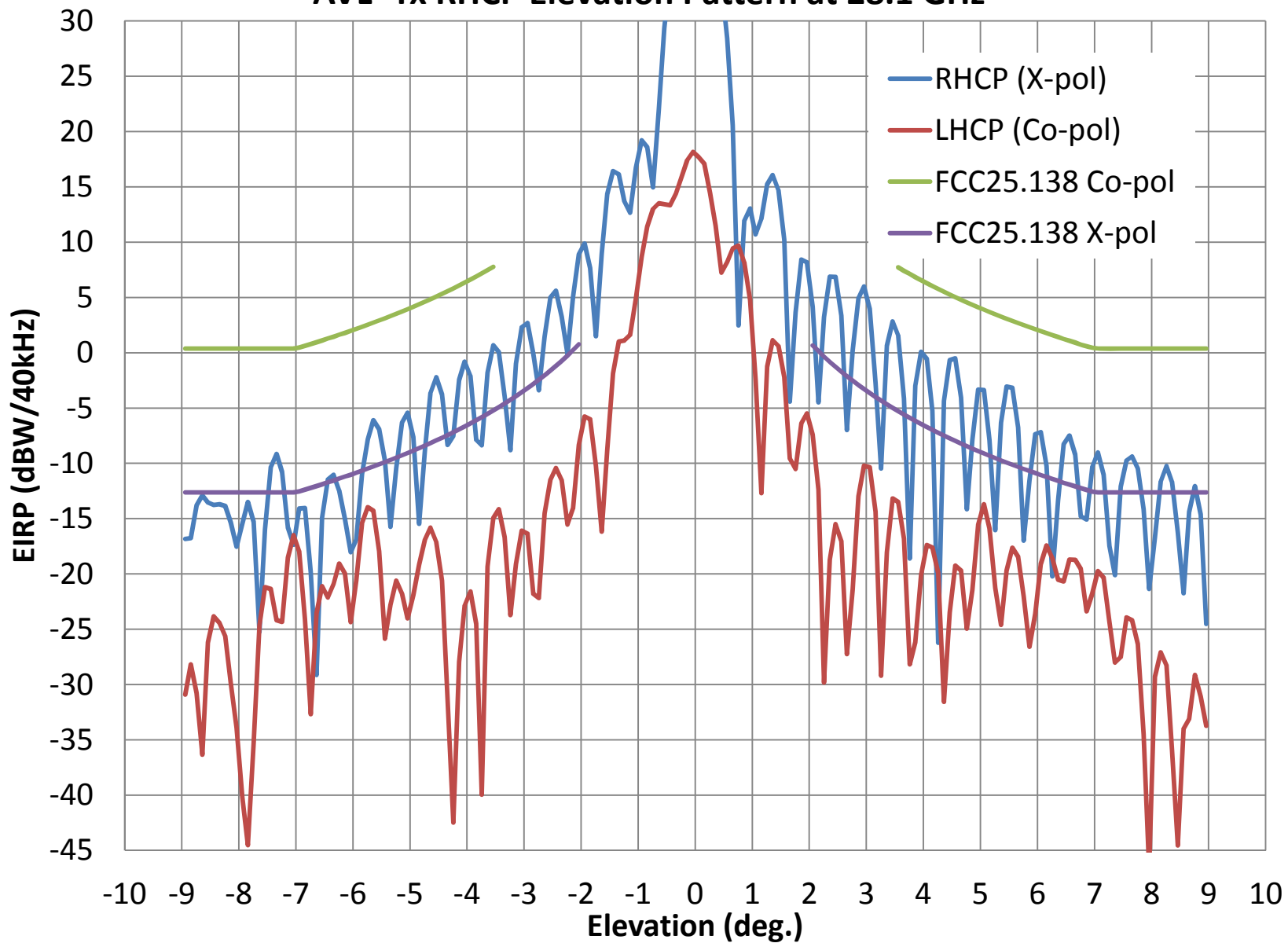
AVL- Tx RHCP Elevation Pattern at 28.1 GHz
