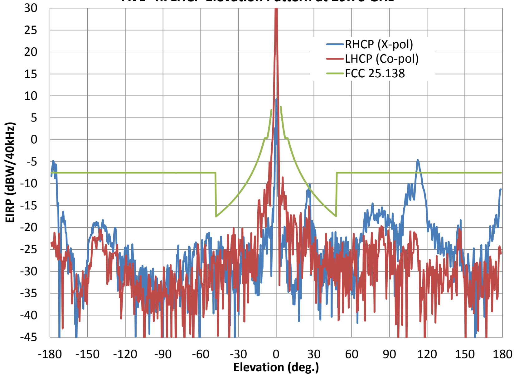
AVL- Tx LHCP Elevation Pattern at 29.75 GHz
