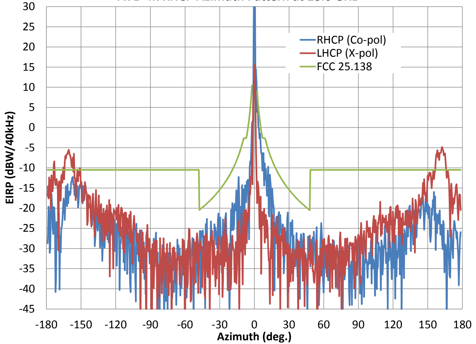
AVL- Tx RHCP Azimuth Pattern at 28.6 GHz
