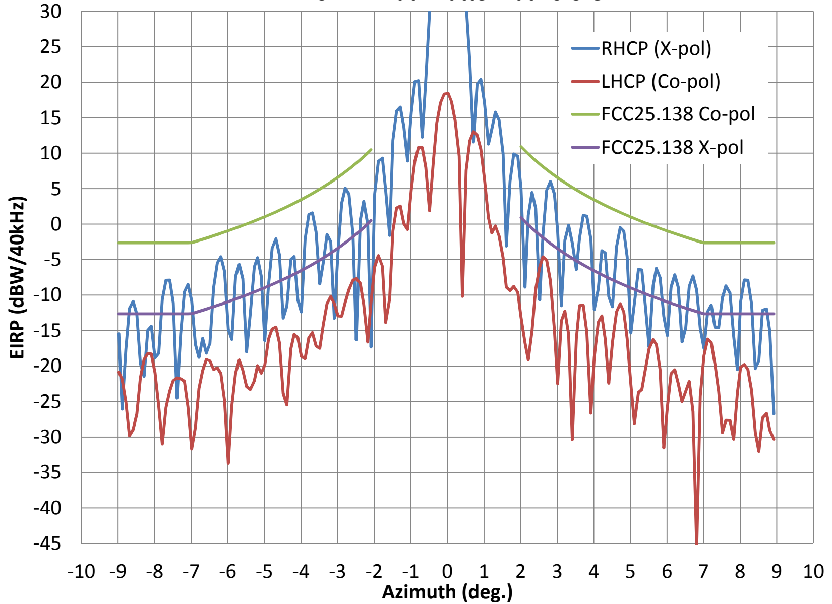
AVL- Tx RHCP Azimuth Pattern at 29.5 GHz
