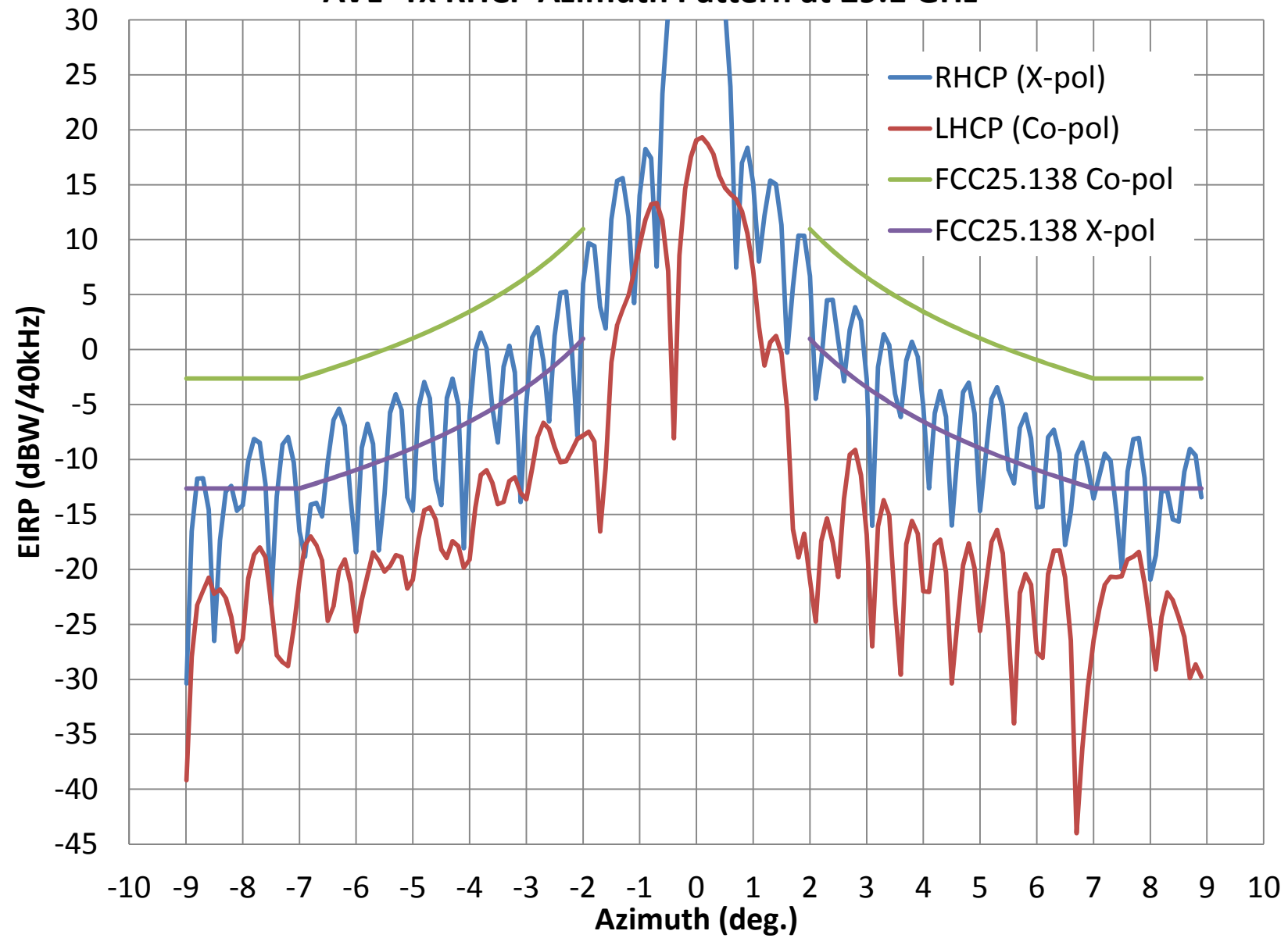
AVL- Tx RHCP Azimuth Pattern at 29.1 GHz
