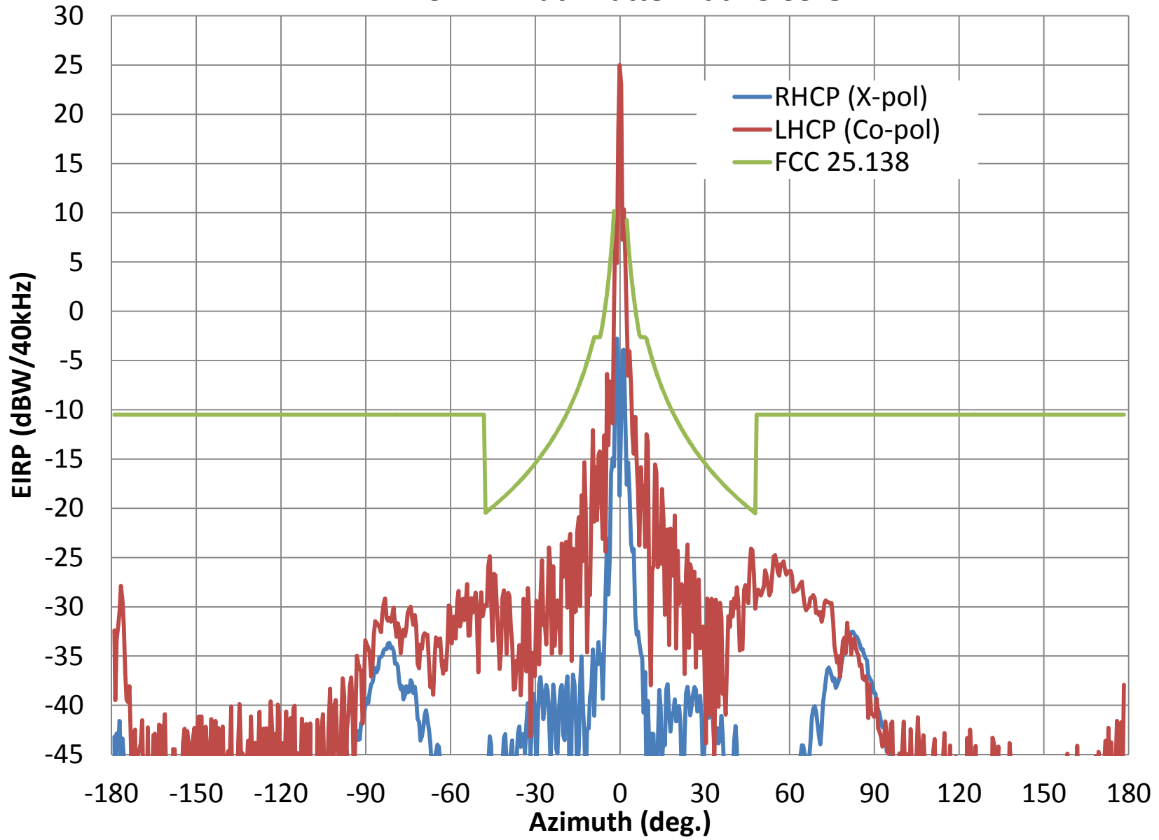
AVL- Tx LHCP Azimuth Pattern at 28.35 GHz
