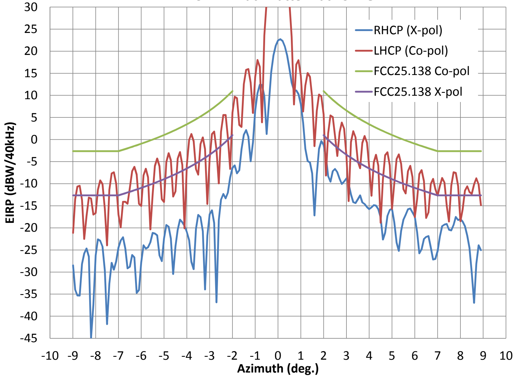
AVL- Tx LHCP Azimuth Pattern at 29.1 GHz
