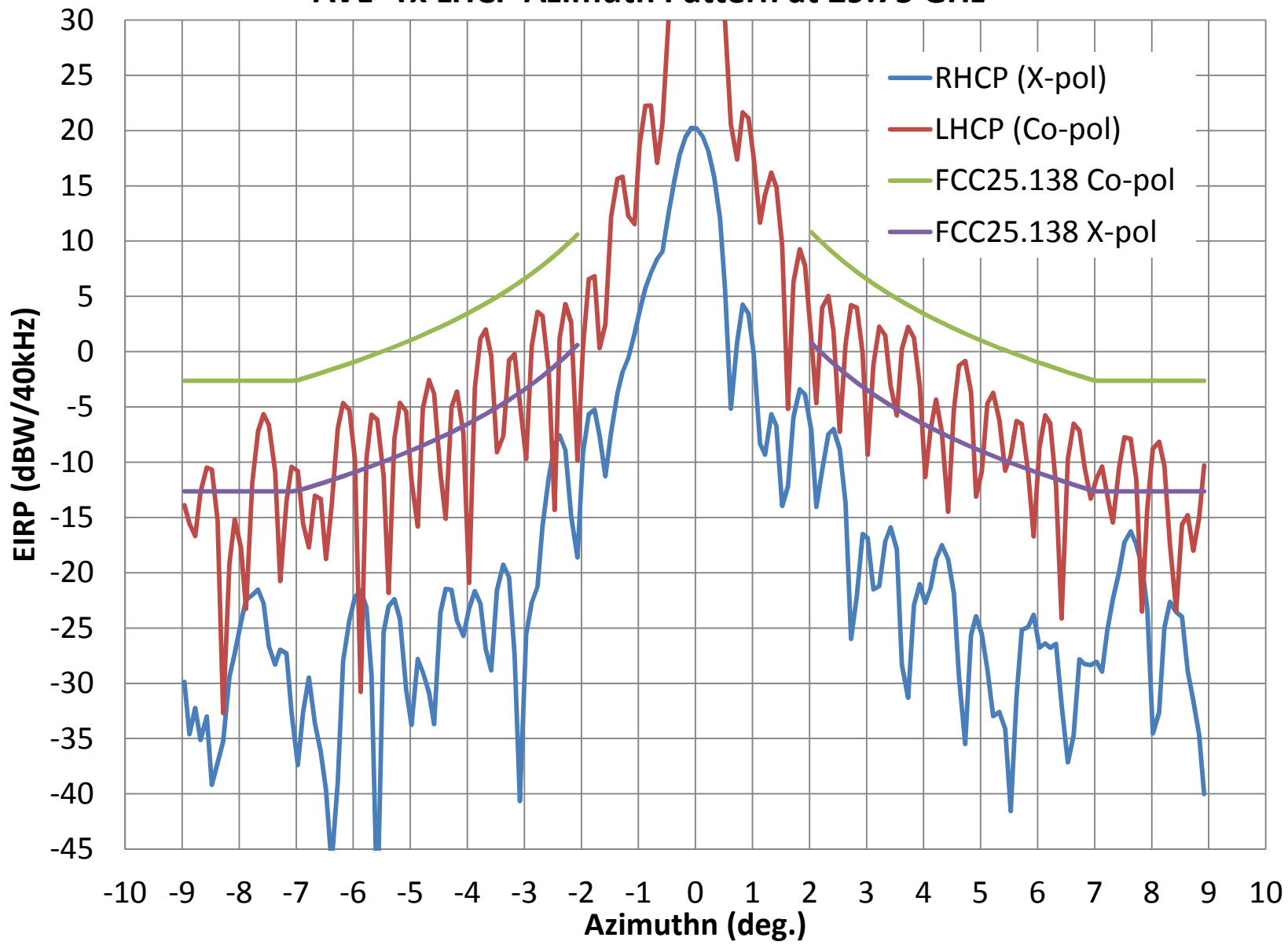
AVL- Tx LHCP Azimuth Pattern at 29.75 GHz
