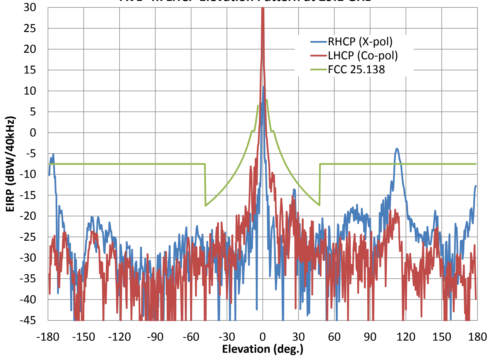
AVL- Tx LHCP Elevation Pattern at 29.1 GHz
