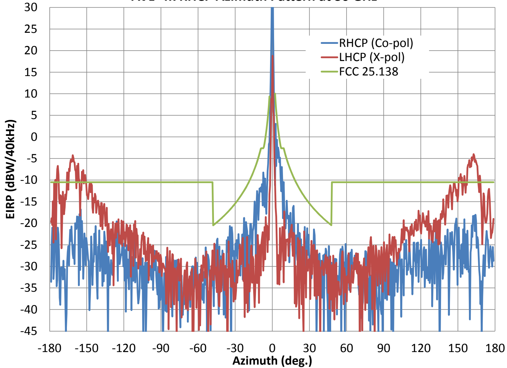
AVL- Tx RHCP Azimuth Pattern at 30 GHz
