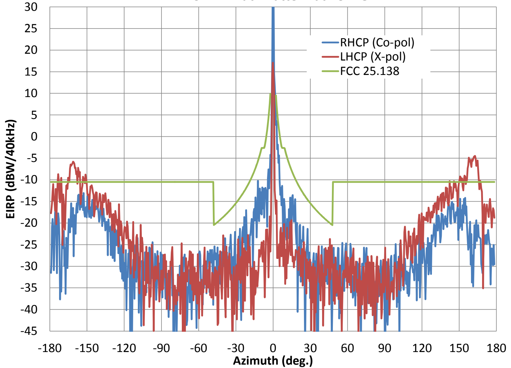
AVL- Tx RHCP Azimuth Pattern at 28.1 GHz
