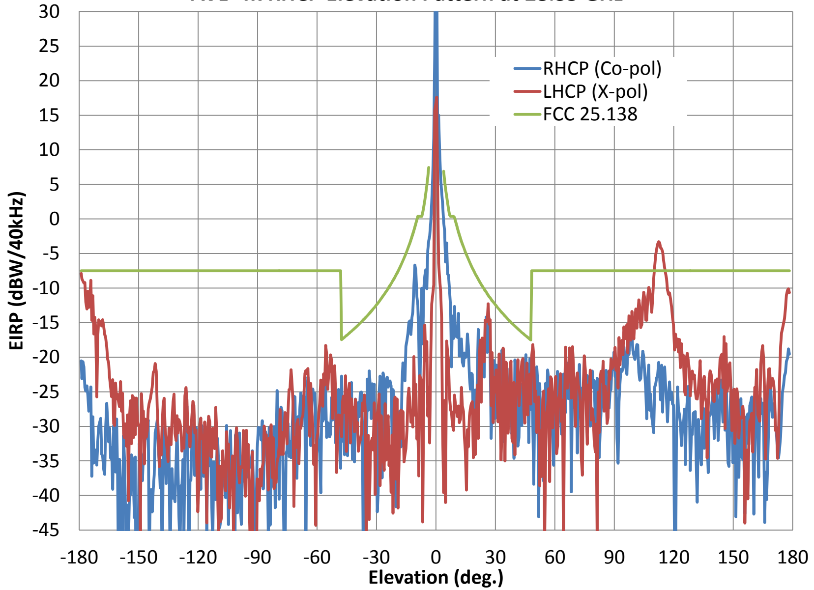
AVL- Tx RHCP Elevation Pattern at 28.35 GHz
