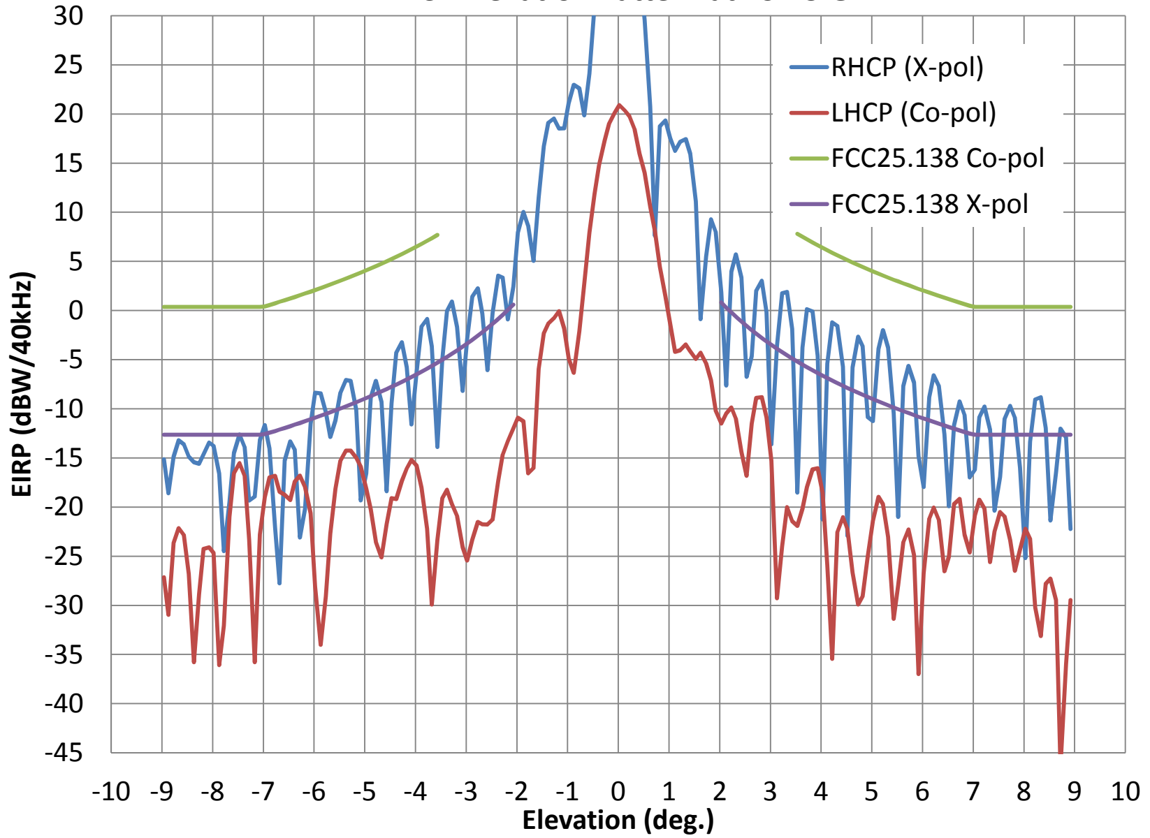
AVL- Tx RHCP Elevation Pattern at 29.75 GHz
