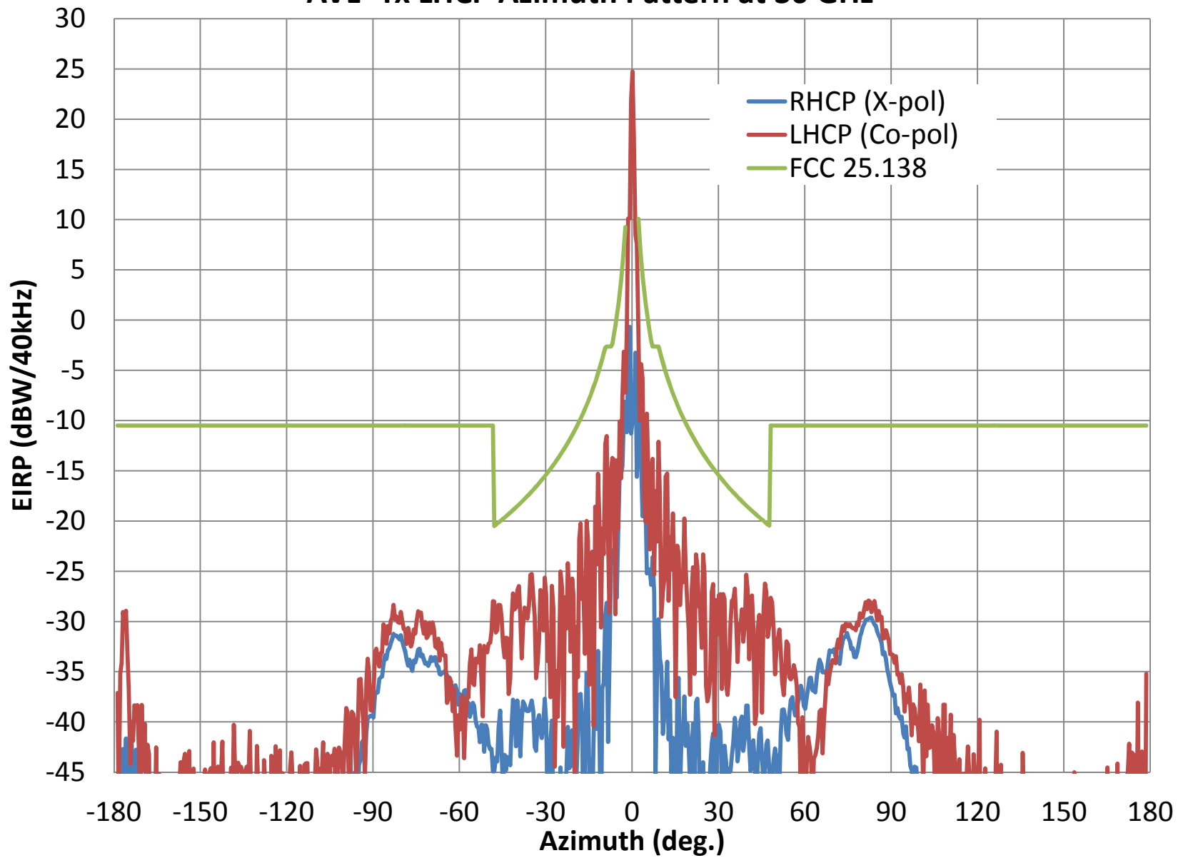
AVL- Tx LHCP Azimuth Pattern at 30 GHz
