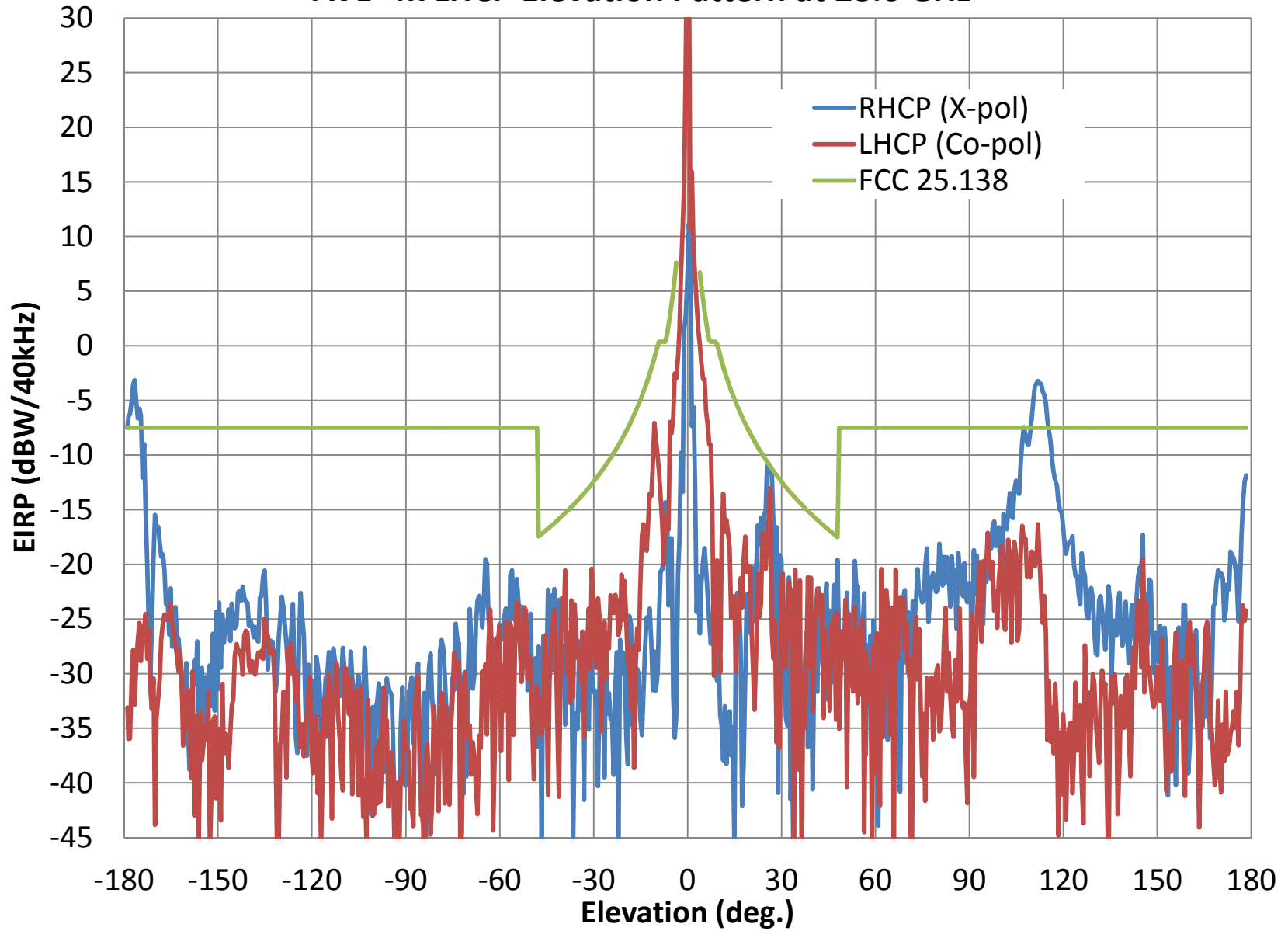
AVL- Tx LHCP Elevation Pattern at 28.6 GHz
