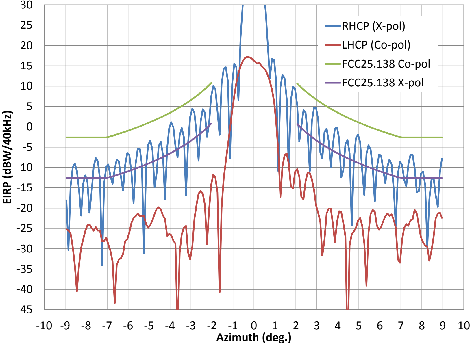
AVL- Tx RHCP Azimuth Pattern at 28.1 GHz
