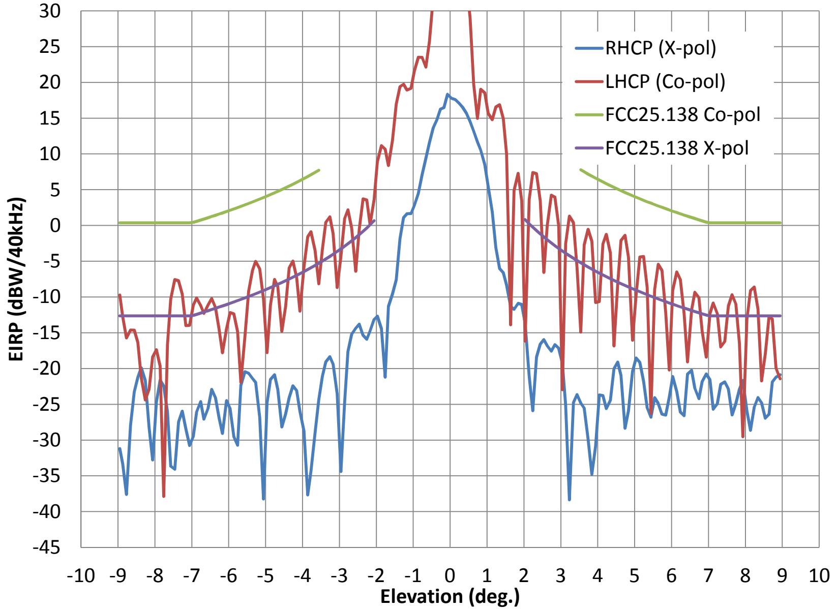
AVL- Tx LHCP Elevation Pattern at 30 GHz
