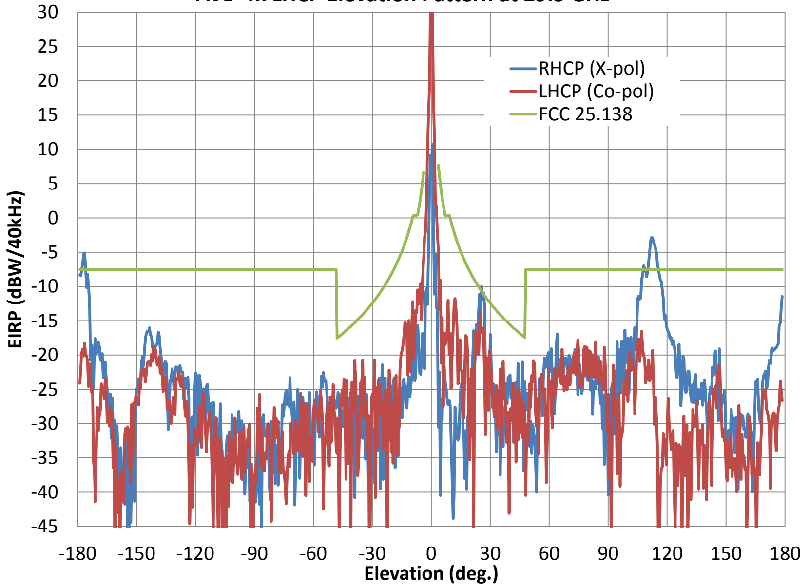
AVL- Tx LHCP Elevation Pattern at 29.5 GHz
