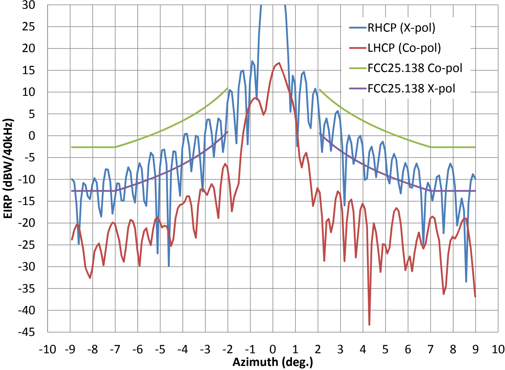
AVL- Tx RHCP Azimuth Pattern at 28.6 GHz
