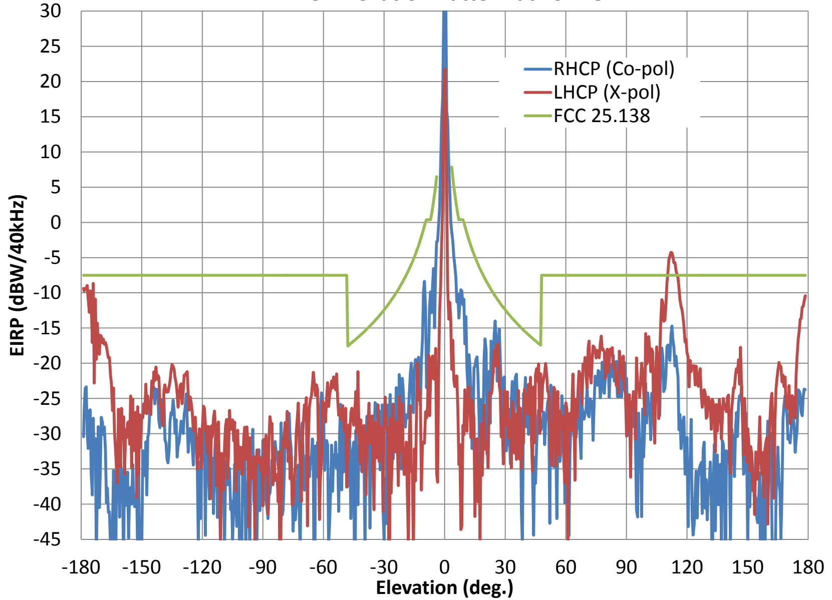
AVL- Tx RHCP Elevation Pattern at 29.1 GHz
