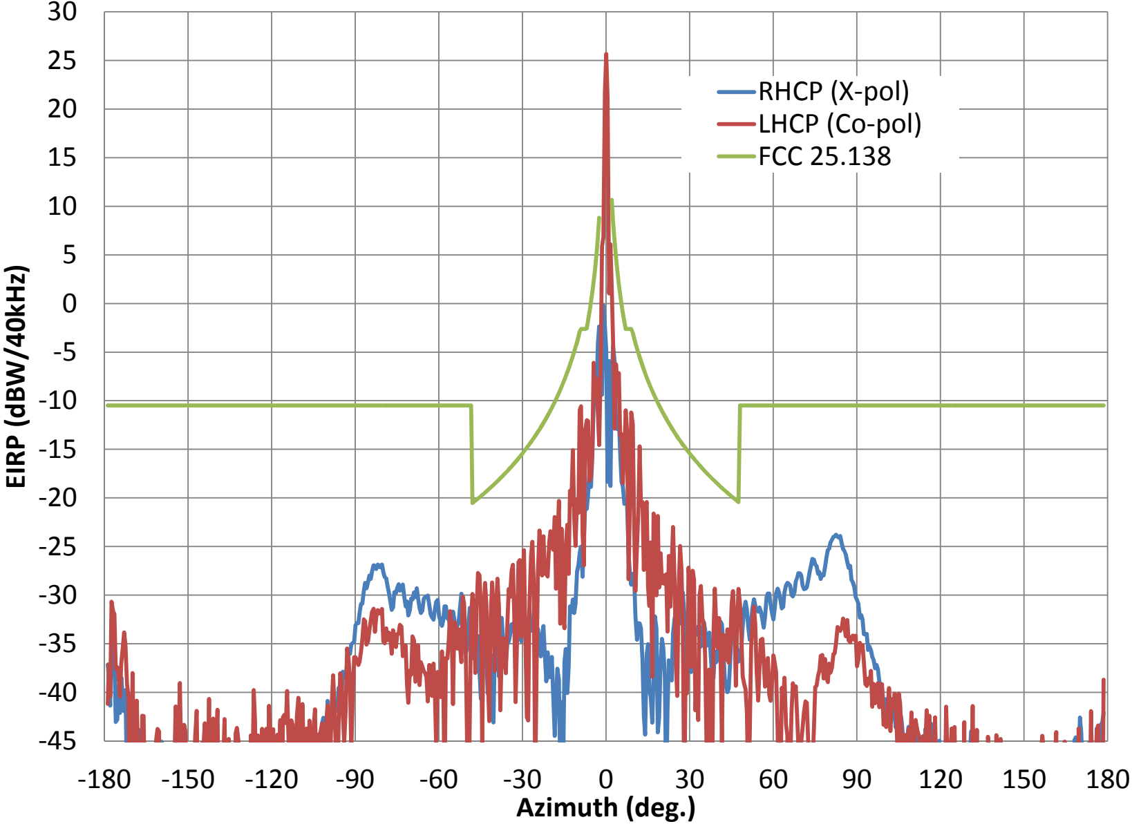
AVL- Tx LHCP Azimuth Pattern at 29.5 GHz
