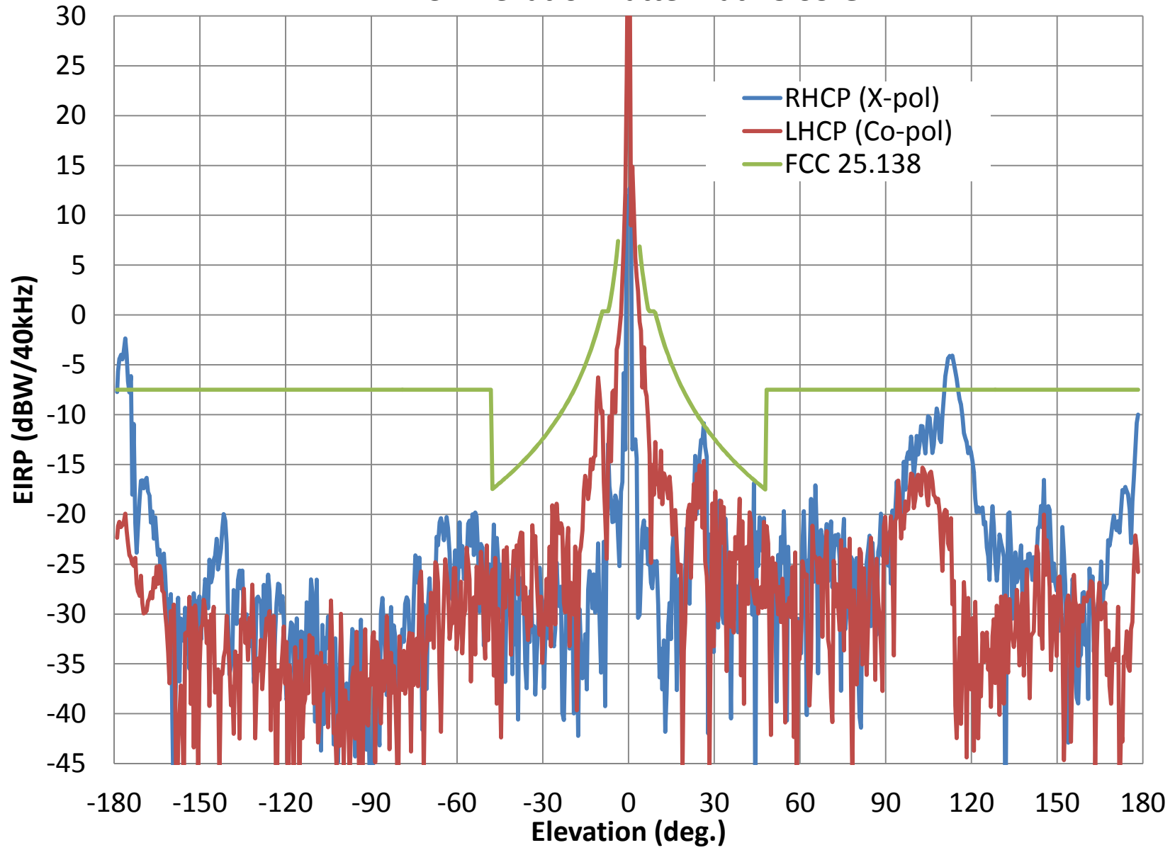
AVL- Tx LHCP Elevation Pattern at 28.35 GHz
