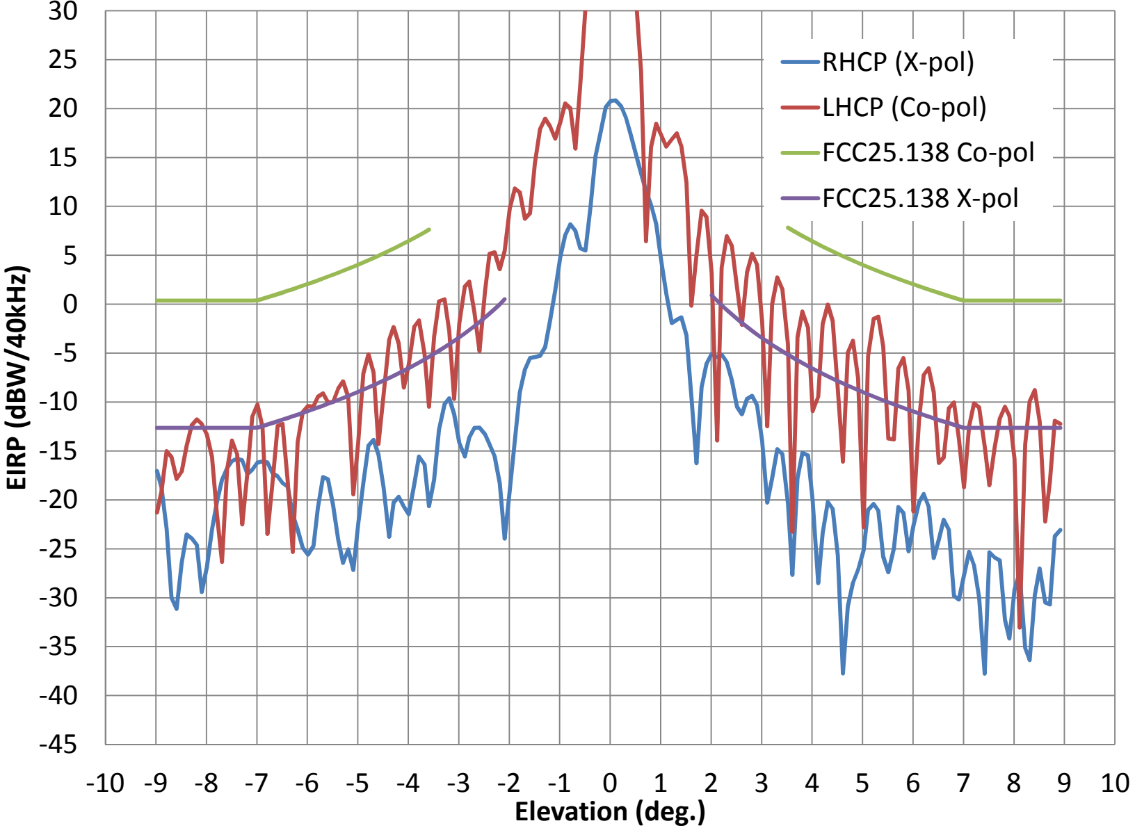
AVL- Tx LHCP Elevation Pattern at 29.5 GHz
