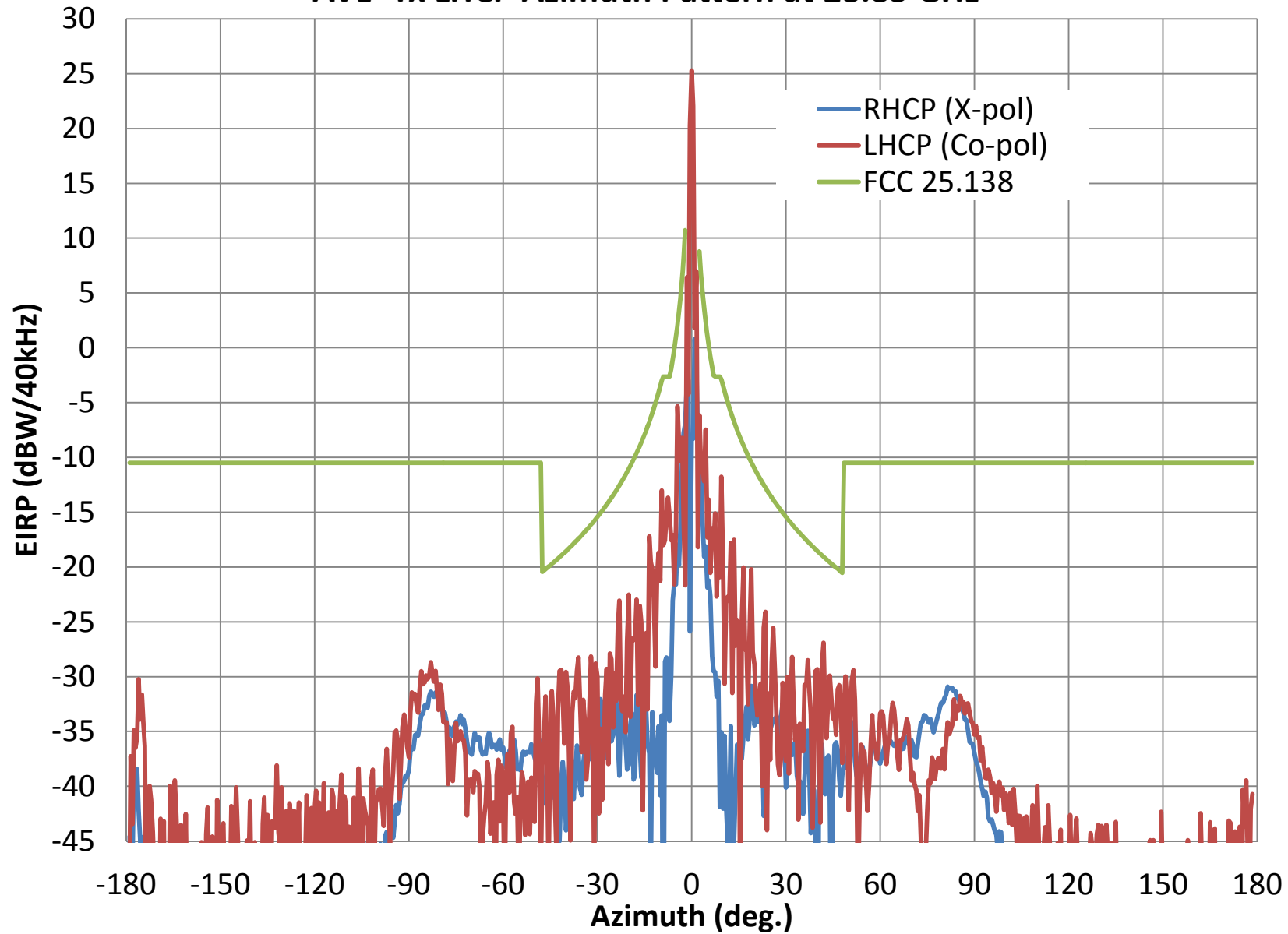
AVL- Tx LHCP Azimuth Pattern at 28.85 GHz
