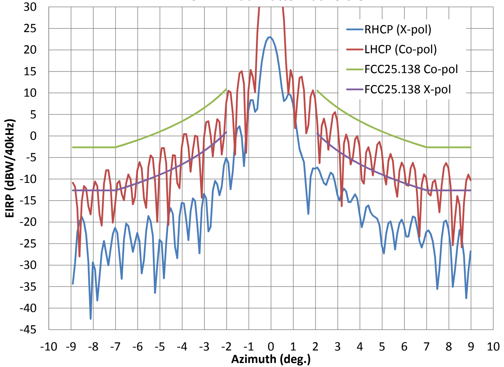
AVL- Tx LHCP Azimuth Pattern at 28.6 GHz
