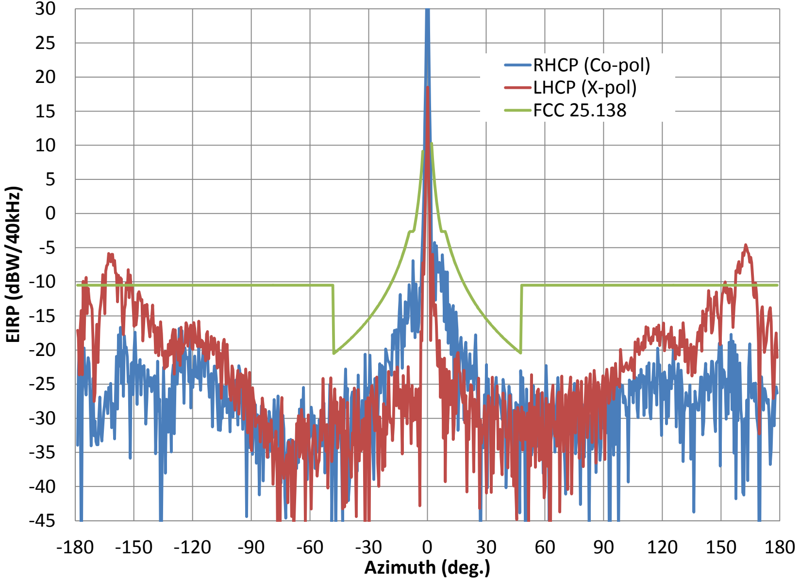
AVL- Tx RHCP Azimuth Pattern at 29.75 GHz
