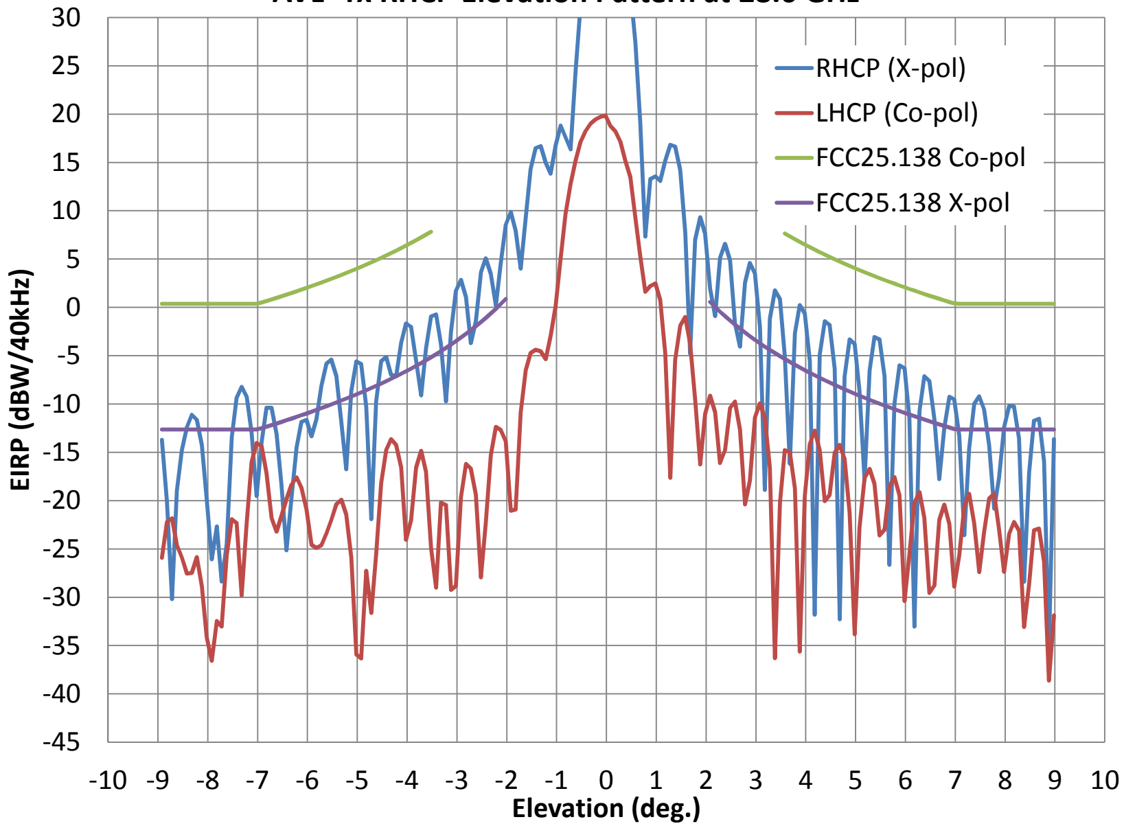
AVL- Tx RHCP Elevation Pattern at 28.6 GHz
