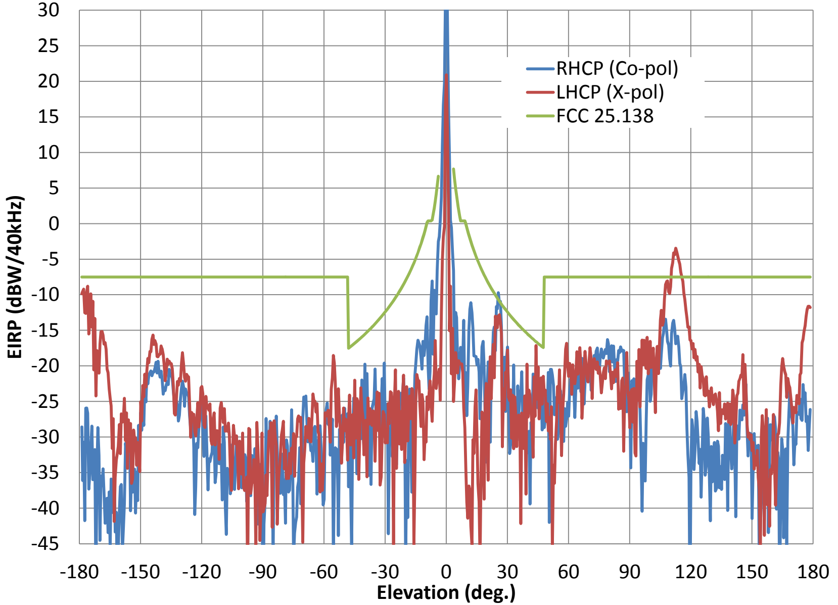
AVL- Tx RHCP Elevation Pattern at 29.5 GHz
