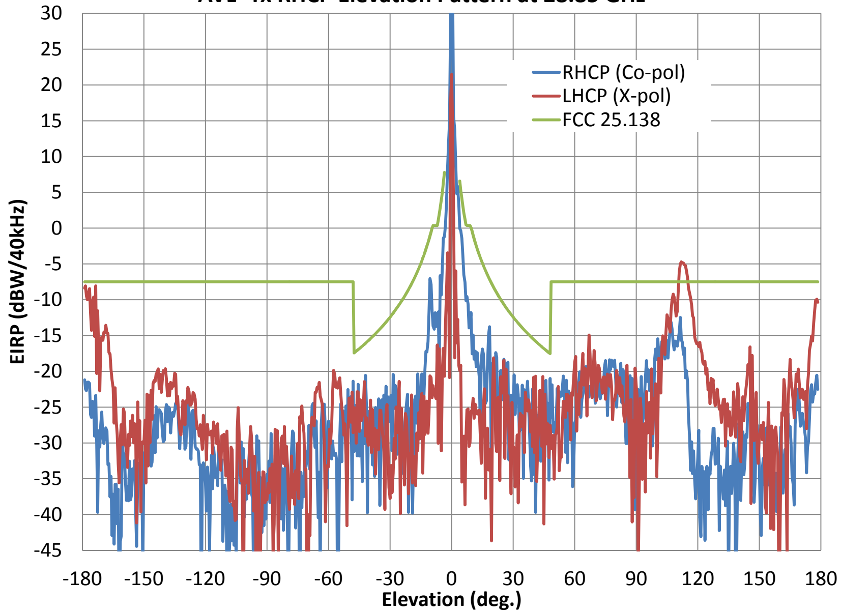
AVL- Tx RHCP Elevation Pattern at 28.85 GHz
