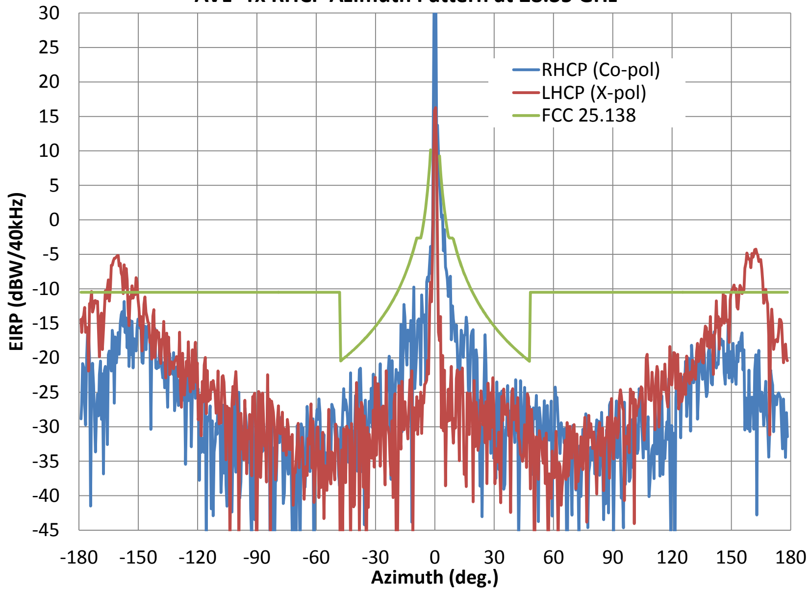
AVL- Tx RHCP Azimuth Pattern at 28.35 GHz
