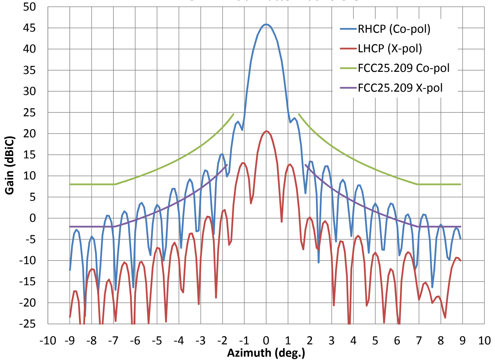
AVL- Rx RHCP Azimuth Pattern at 19.3 GHz
