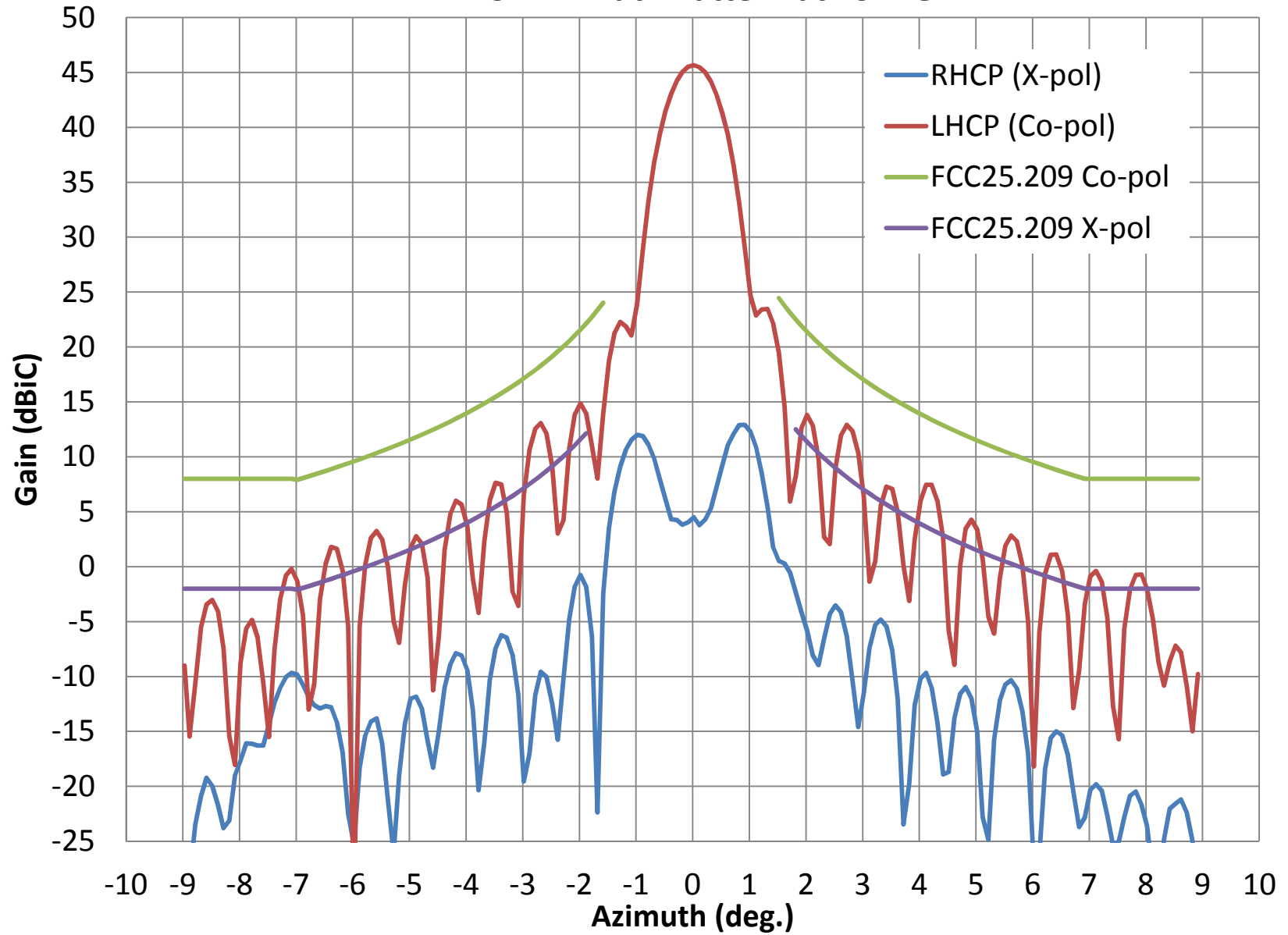
AVL- Rx LHCP Azimuth Pattern at 19.7 GHz
