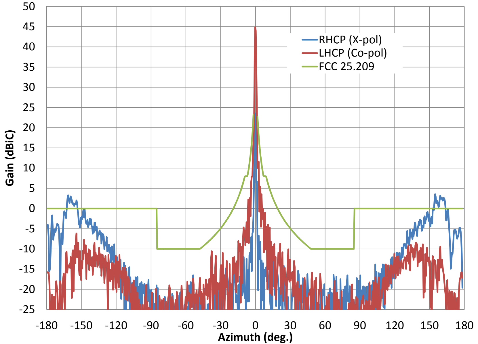
AVL- Rx LHCP Azimuth Pattern at 18.3 GHz
