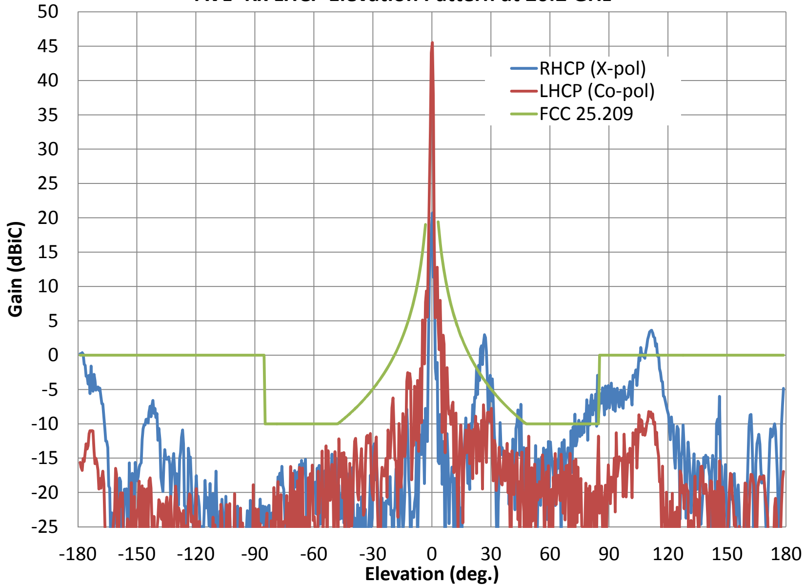
AVL- Rx LHCP Elevation Pattern at 20.2 GHz
