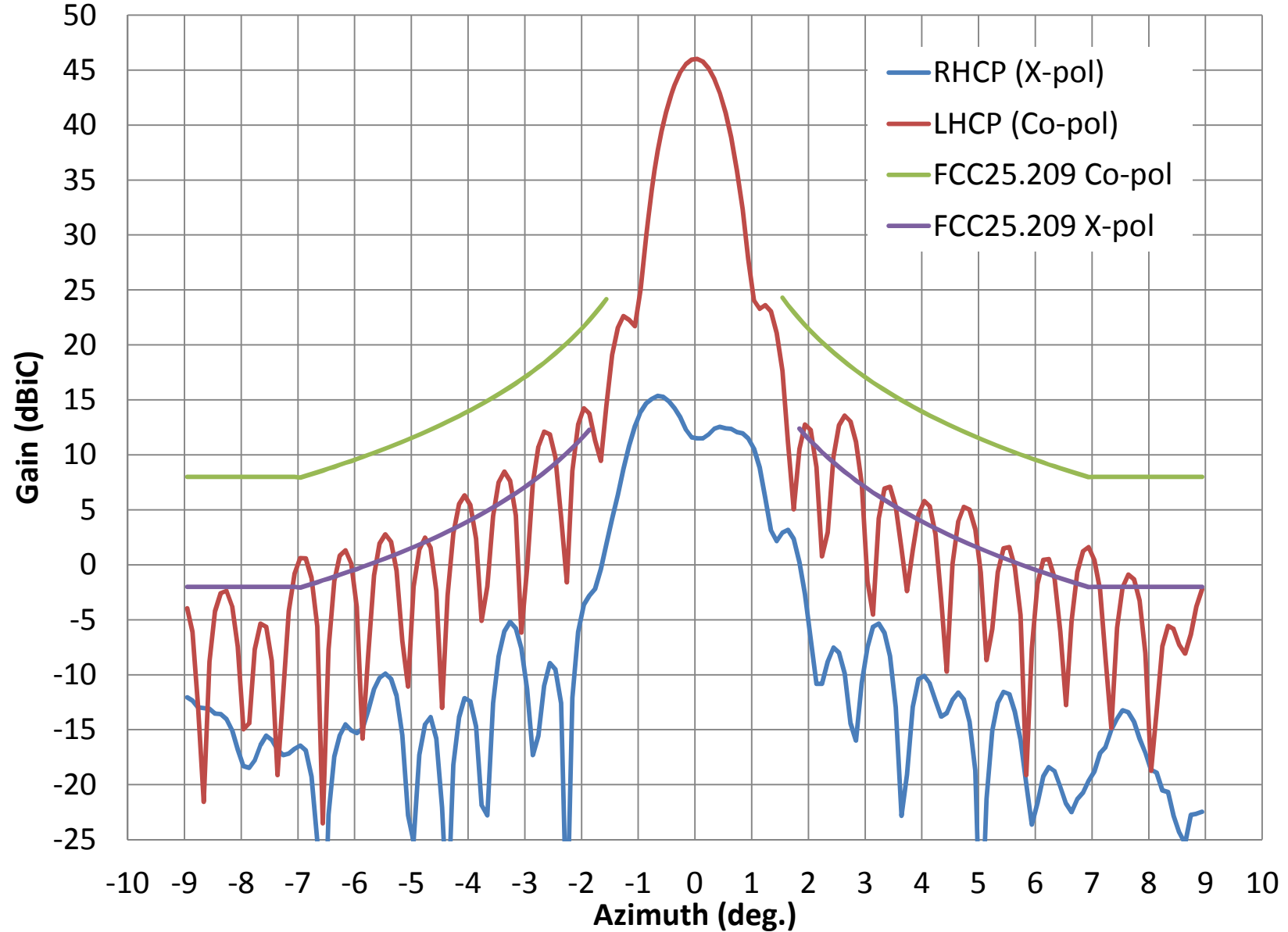
AVL- Rx LHCP Azimuth Pattern at 20.2 GHz
