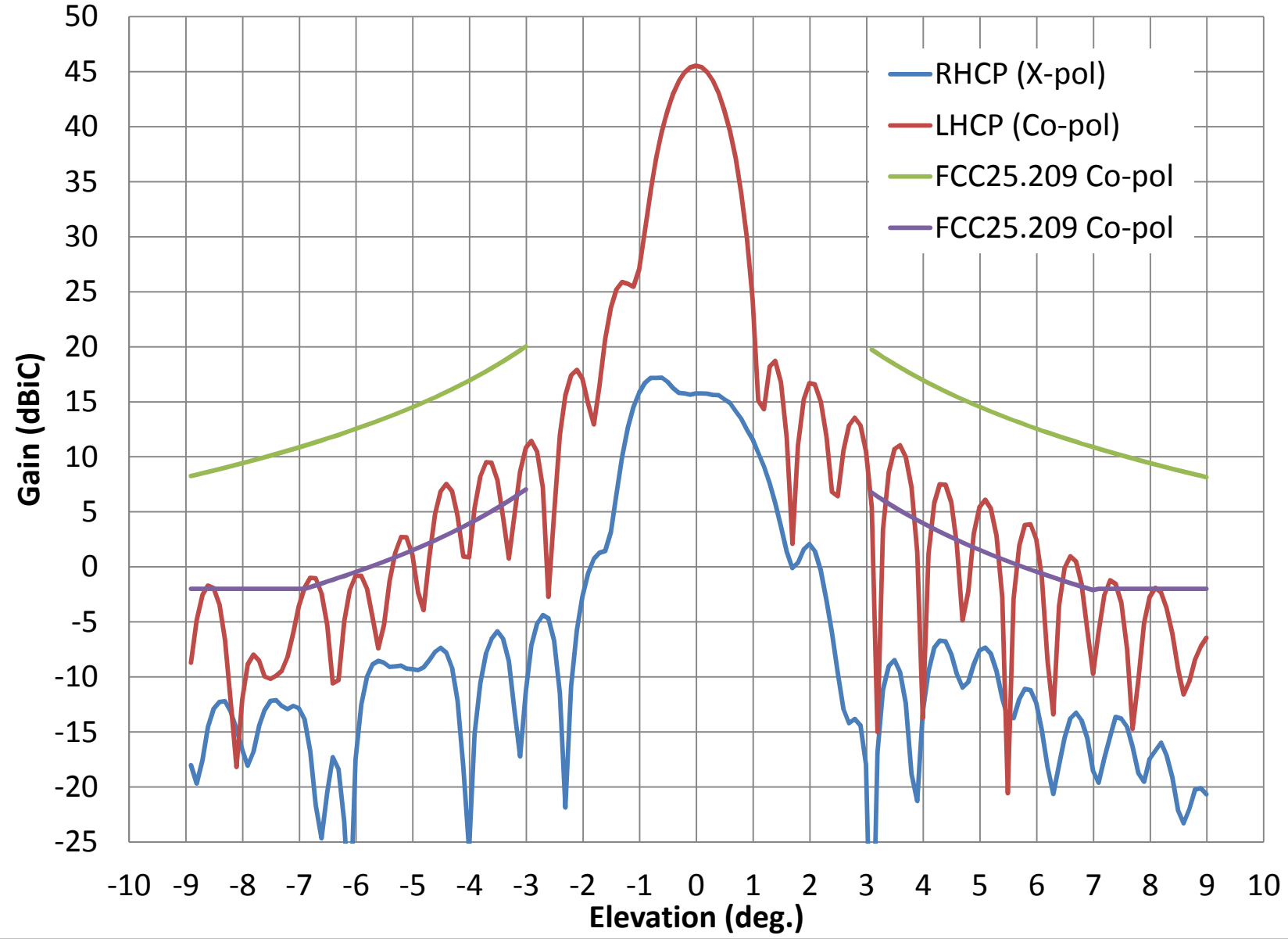
AVL- Rx LHCP Elevation Pattern at 19.05 GHz
