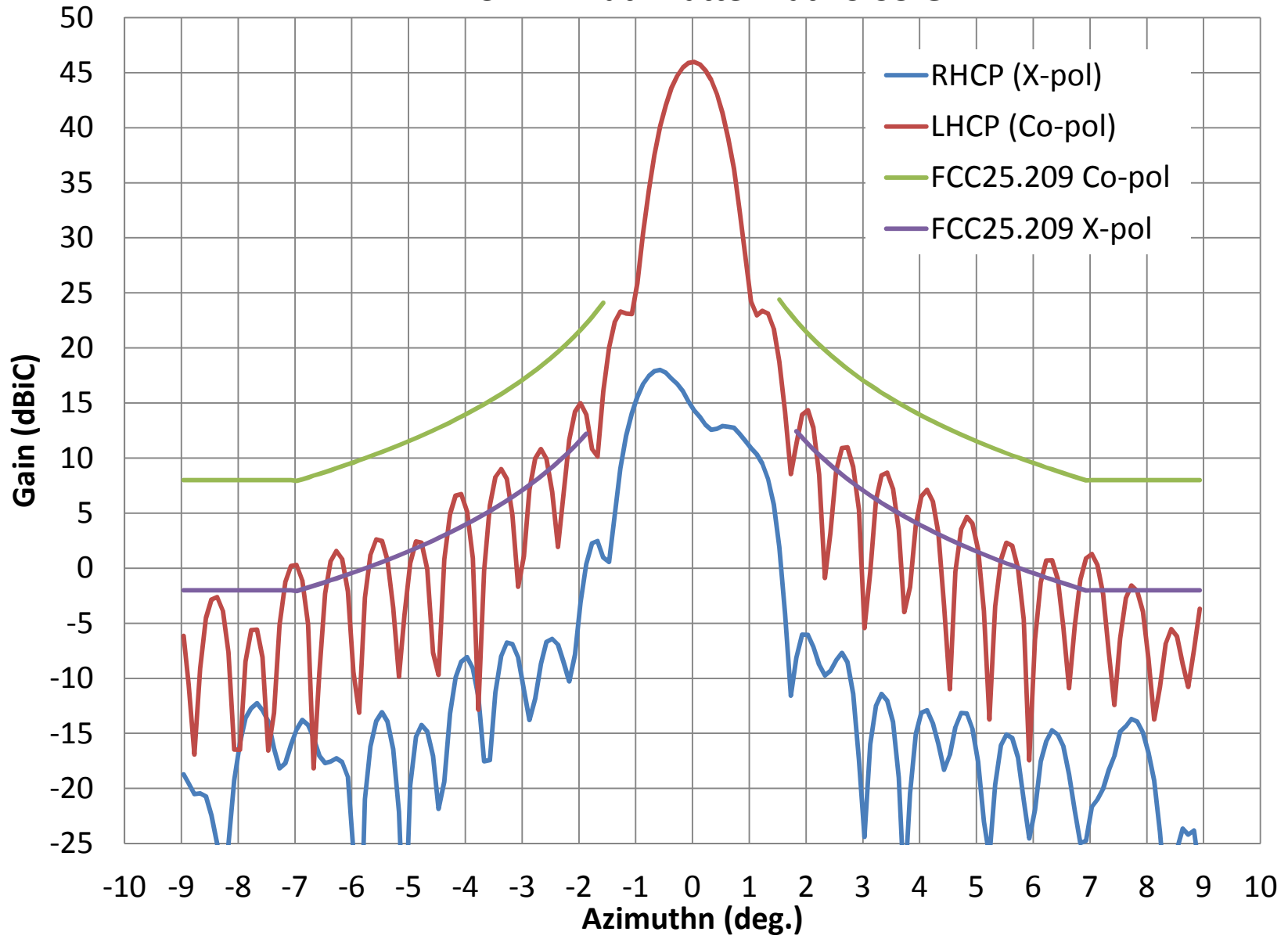
AVL- Rx LHCP Azimuth Pattern at 19.95 GHz
