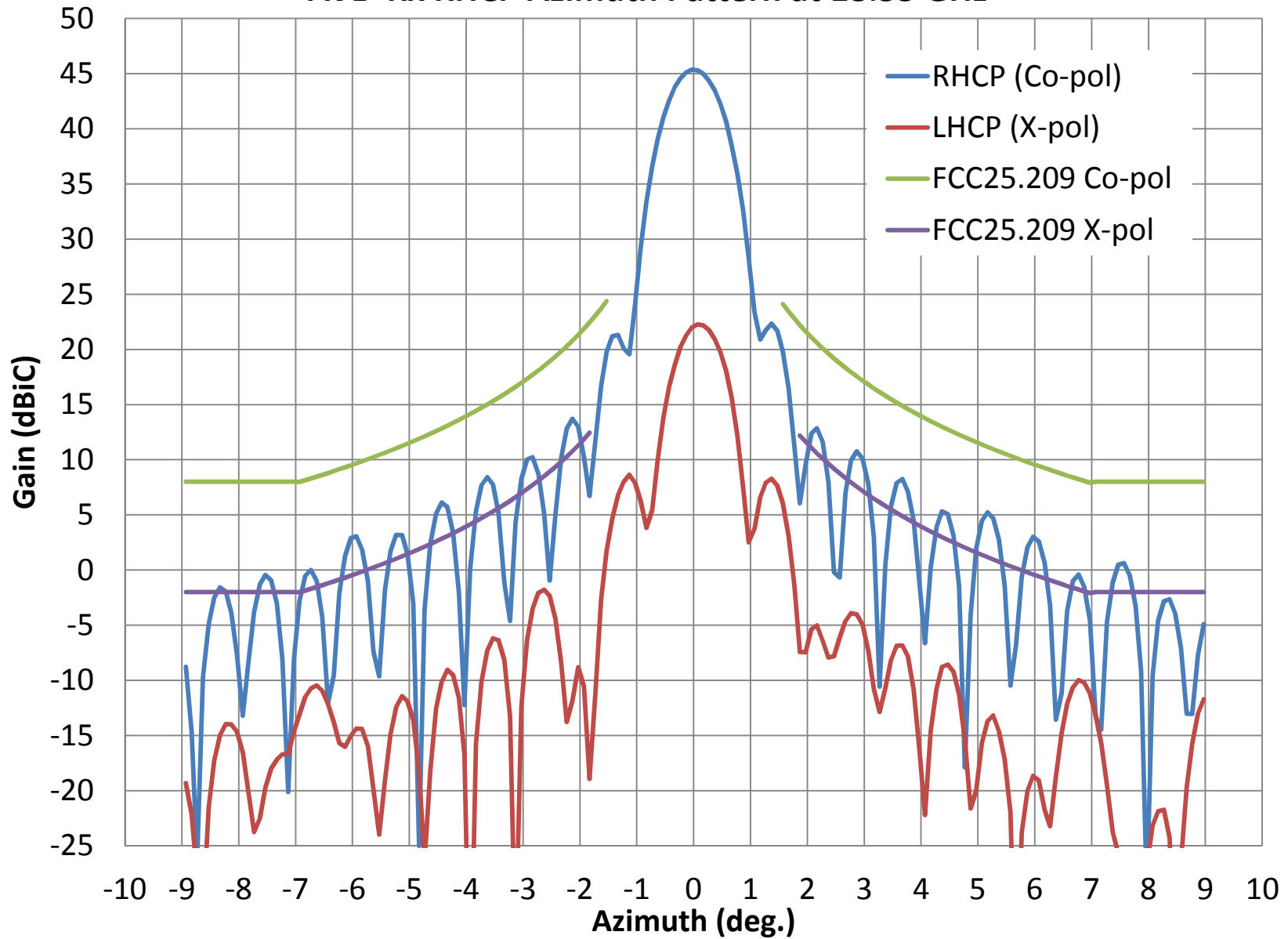
AVL- Rx RHCP Azimuth Pattern at 18.55 GHz
