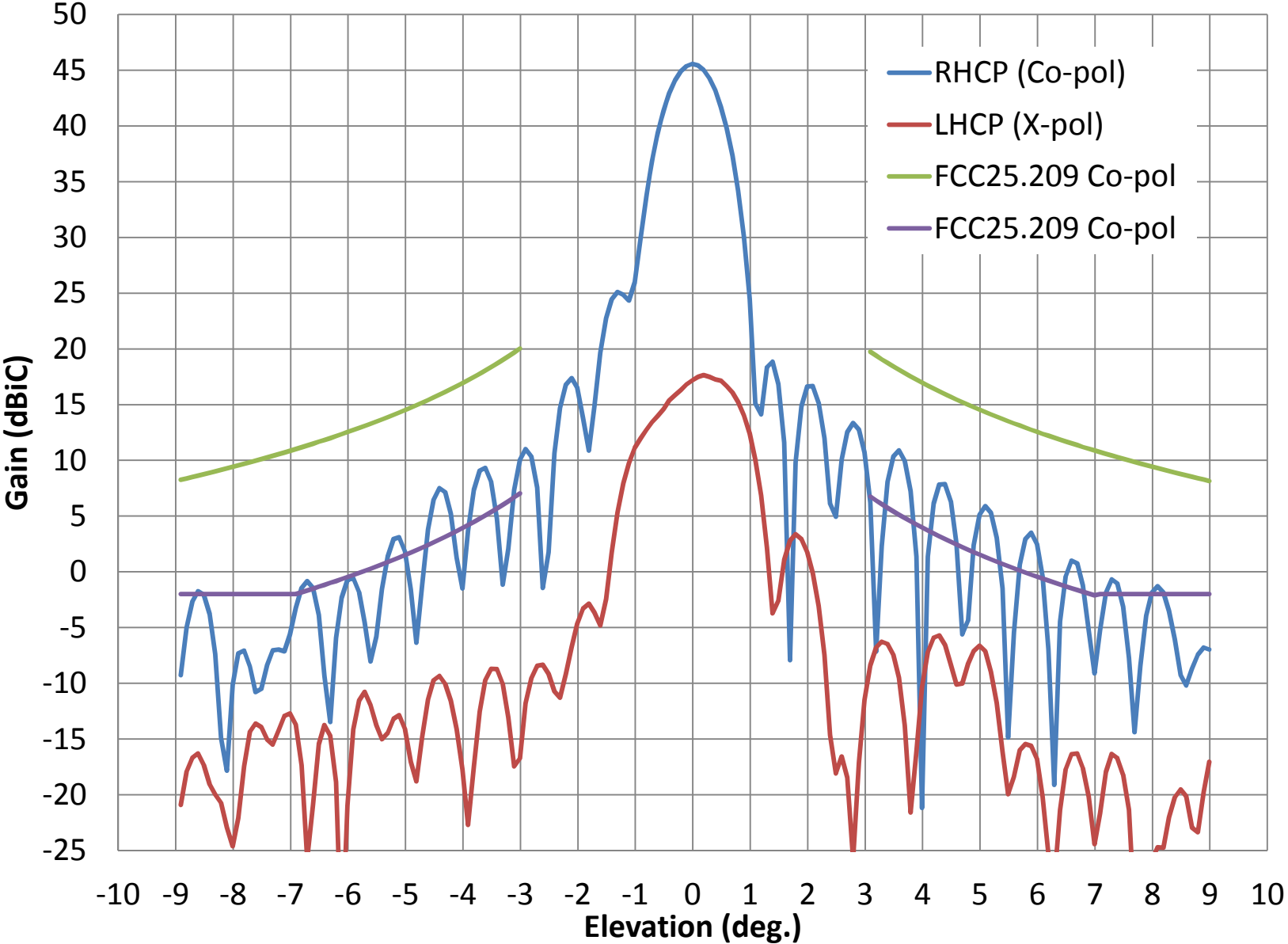
AVL- Rx RHCP Elevation Pattern at 19.05 GHz
