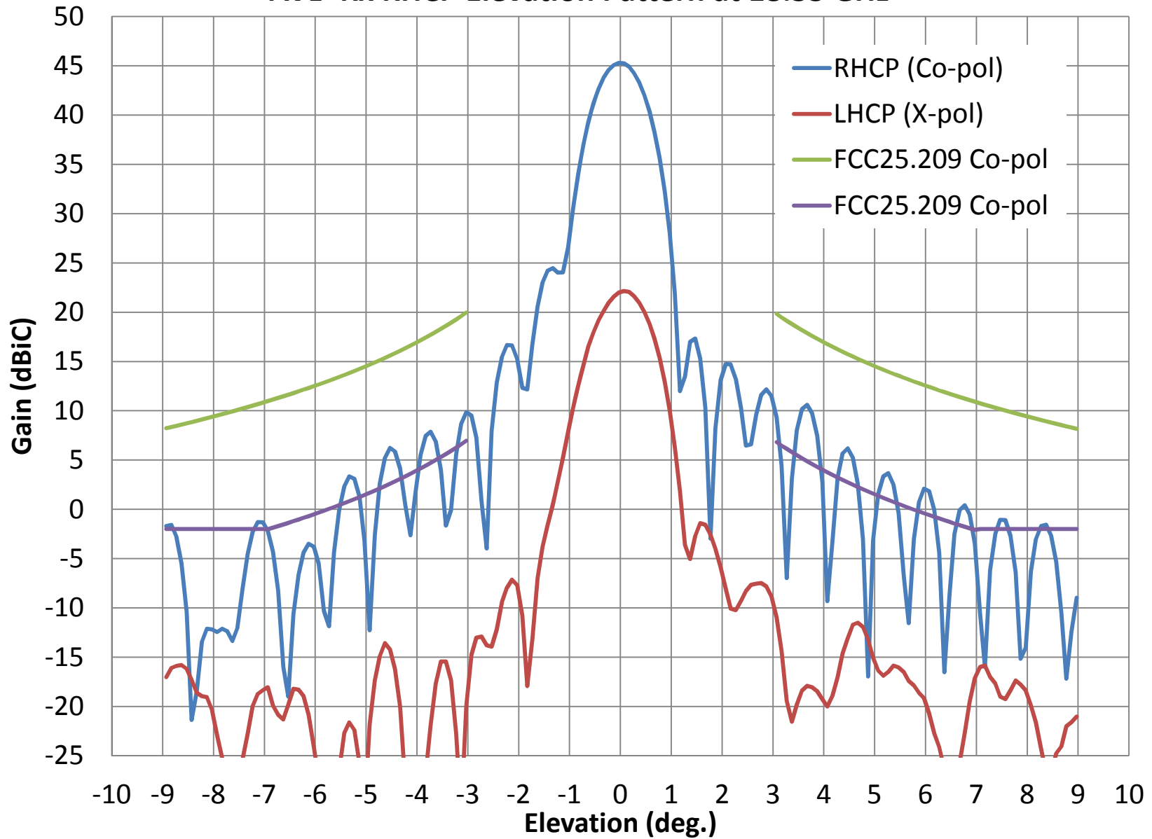
AVL- Rx RHCP Elevation Pattern at 18.55 GHz
