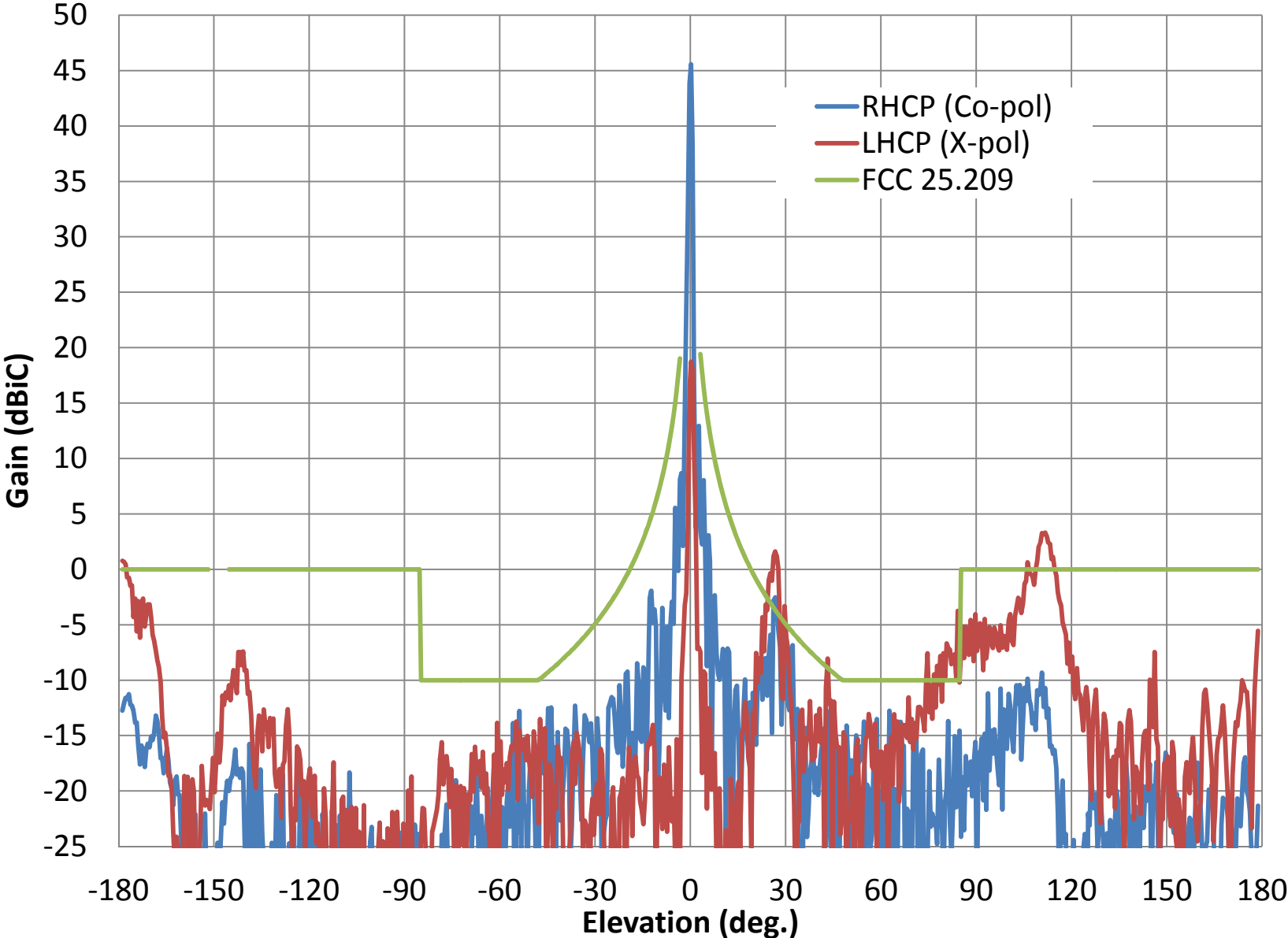
AVL- Rx RHCP Elevation Pattern at 20.2 GHz
