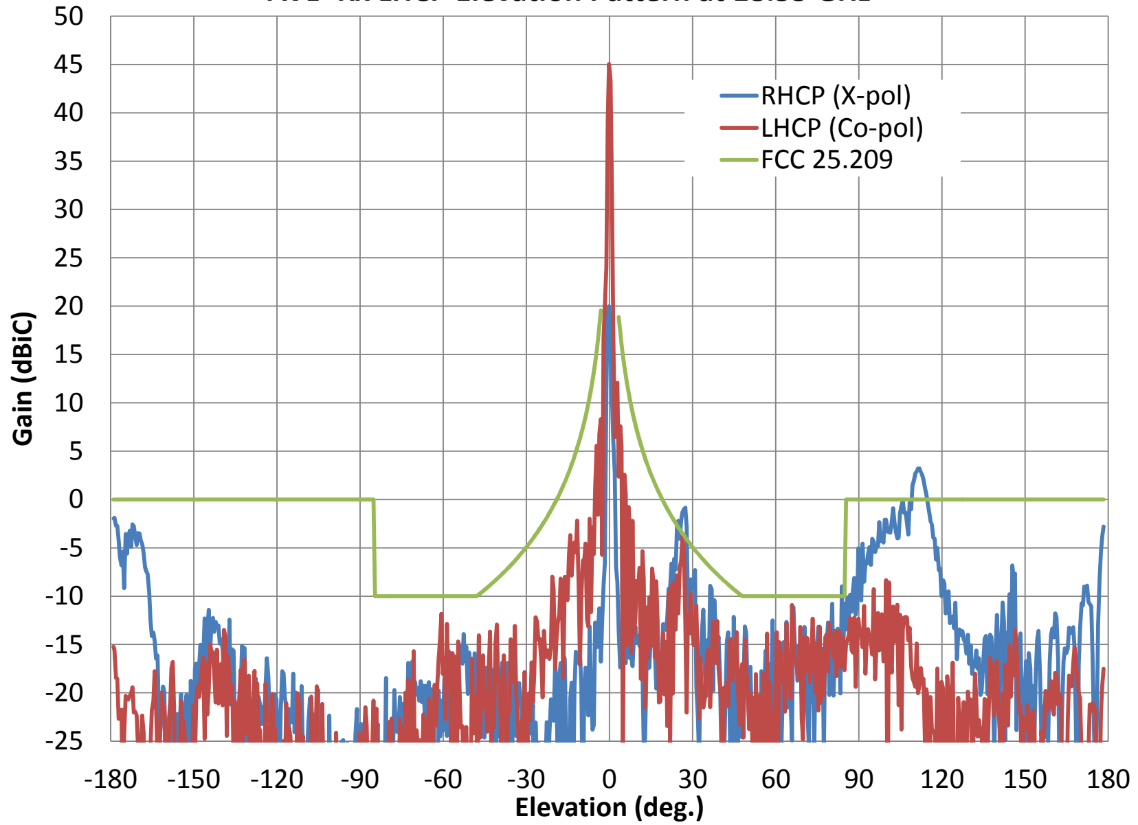
AVL- Rx LHCP Elevation Pattern at 18.55 GHz
