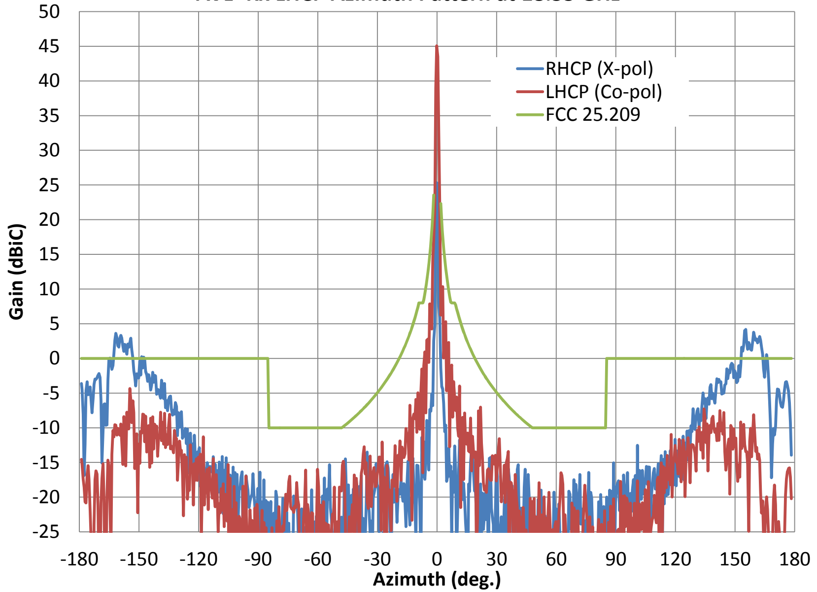
AVL- Rx LHCP Azimuth Pattern at 18.55 GHz
