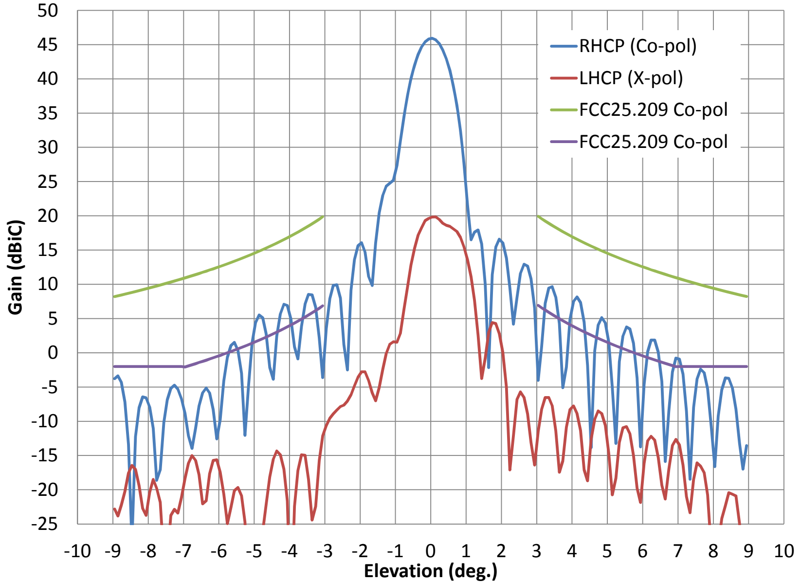
AVL- Rx RHCP Elevation Pattern at 20.2 GHz
