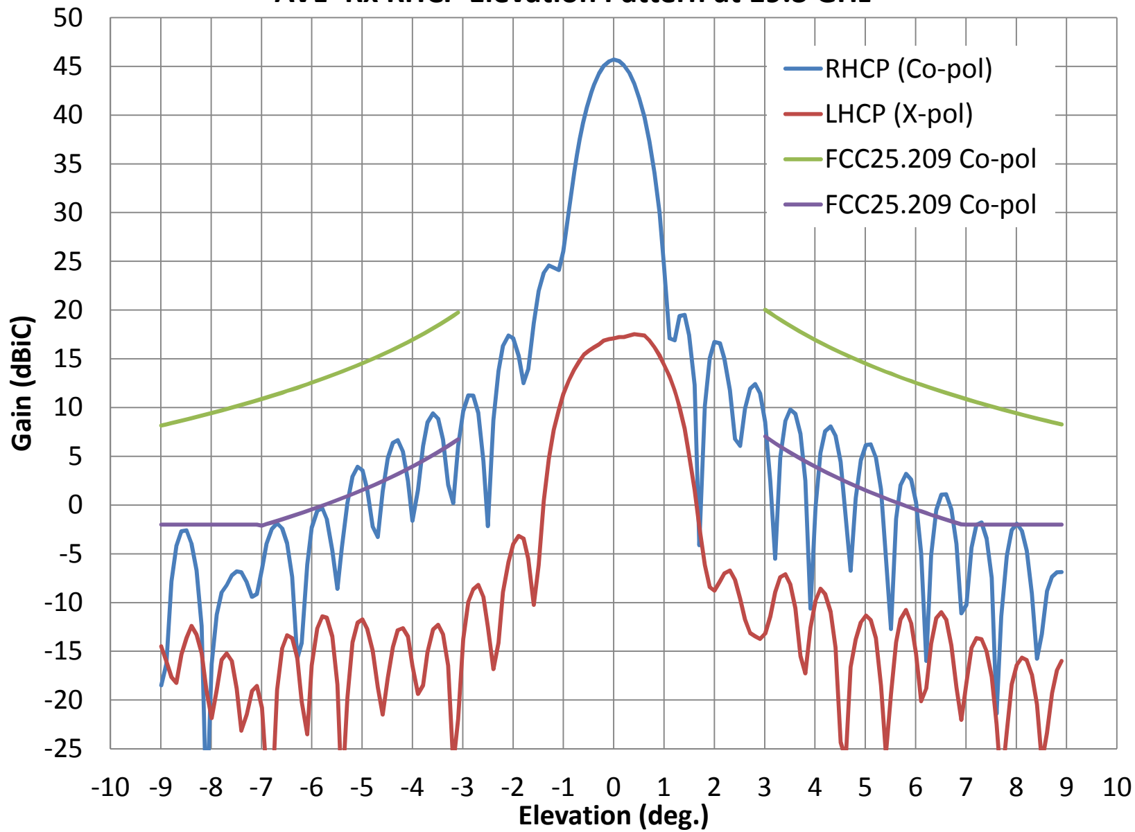
AVL- Rx RHCP Elevation Pattern at 19.3 GHz
