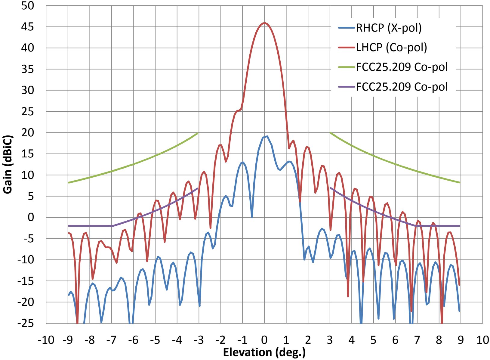
AVL- Rx LHCP Elevation Pattern at 19.95 GHz
