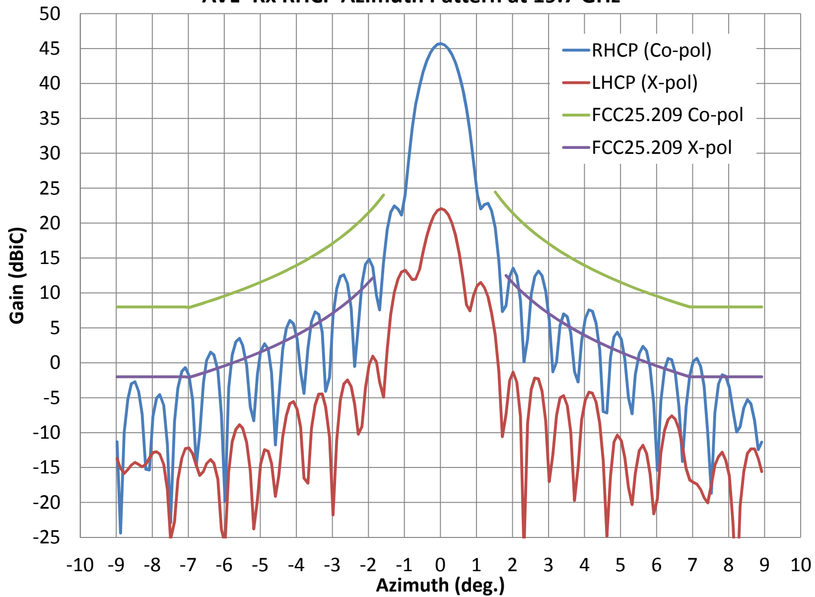
AVL- Rx RHCP Azimuth Pattern at 19.7 GHz
