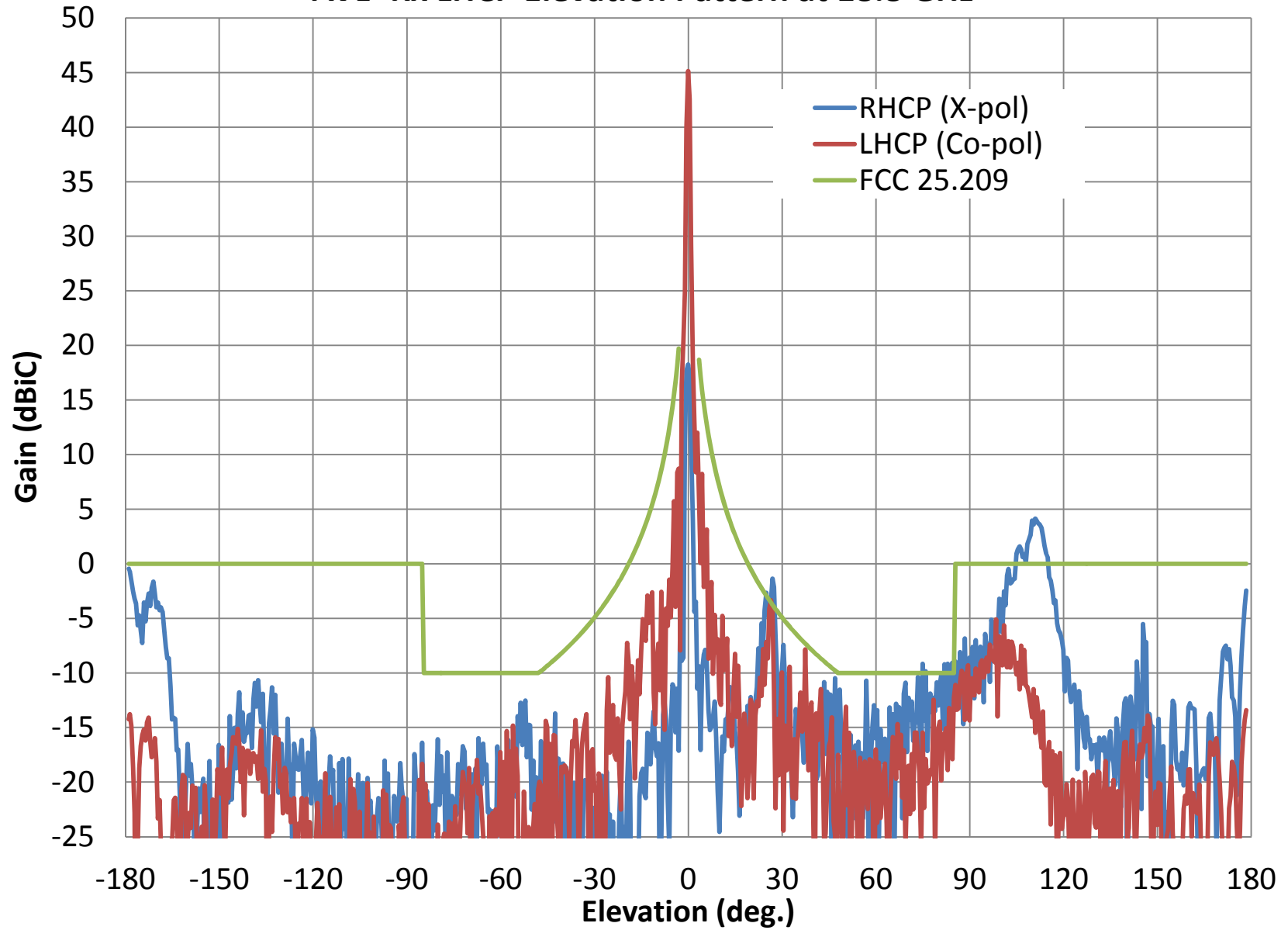
AVL- Rx LHCP Elevation Pattern at 18.8 GHz
