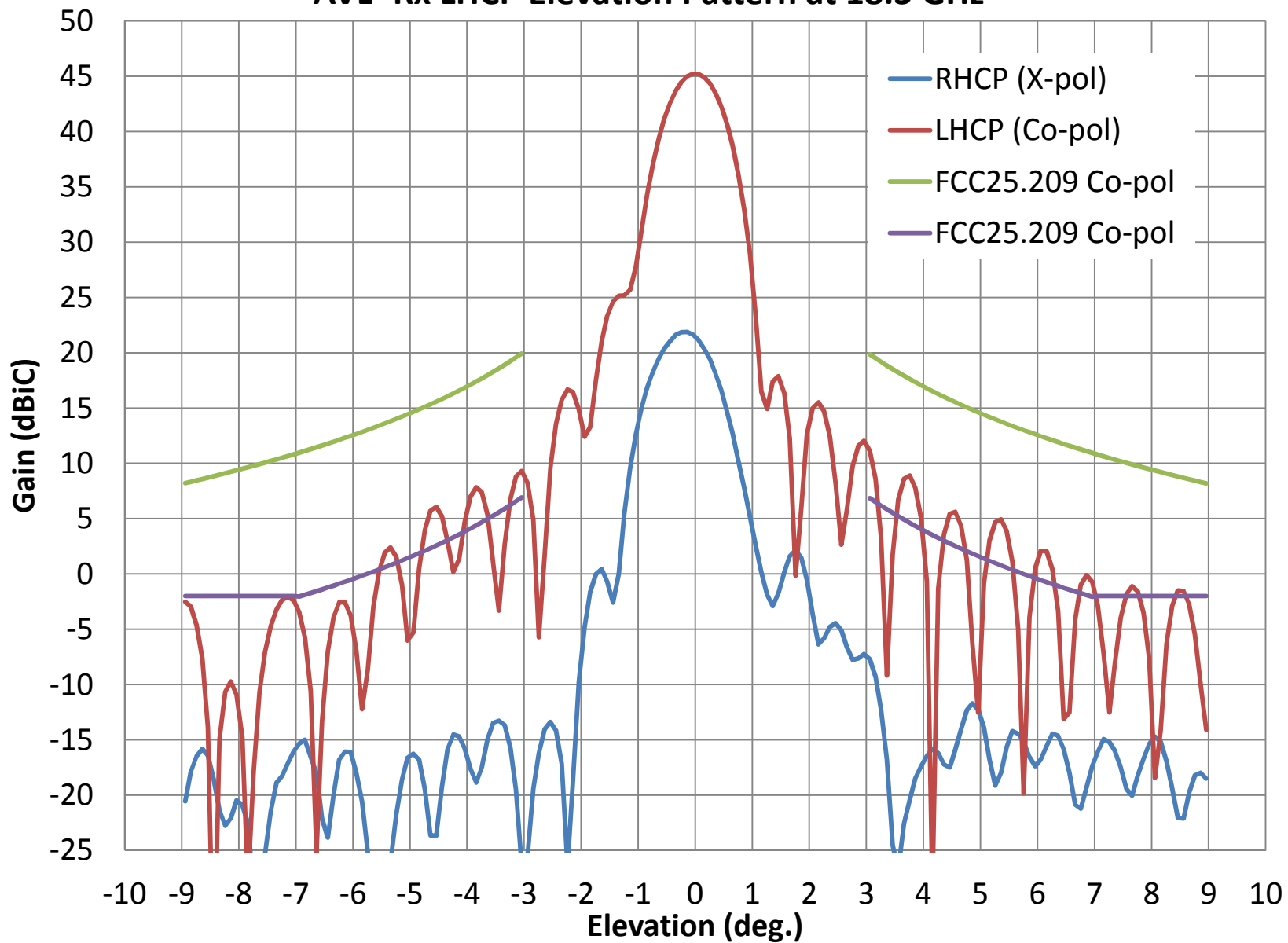
AVL- Rx LHCP Elevation Pattern at 18.3 GHz
