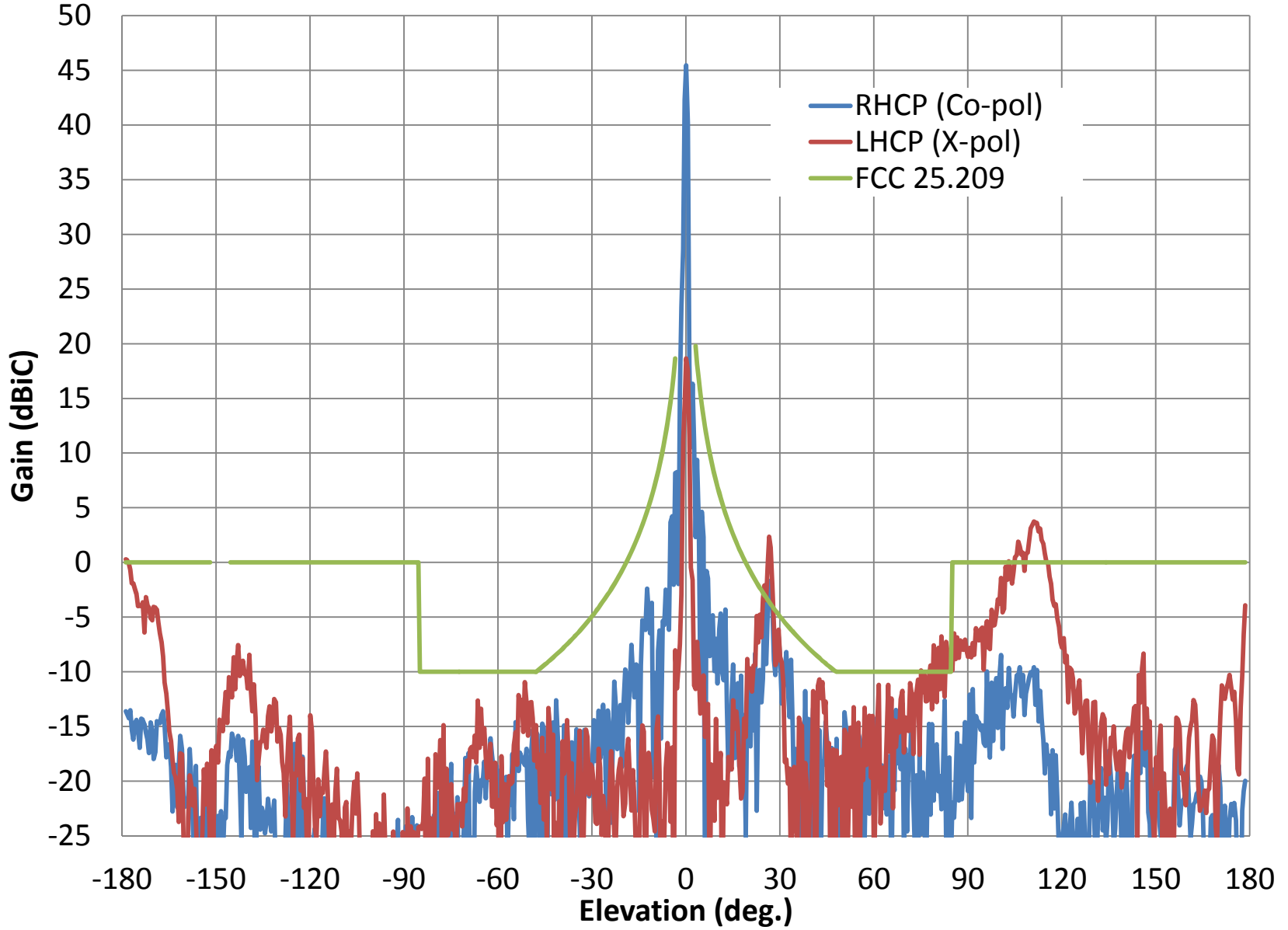
AVL- Rx RHCP Elevation Pattern at 19.7 GHz
