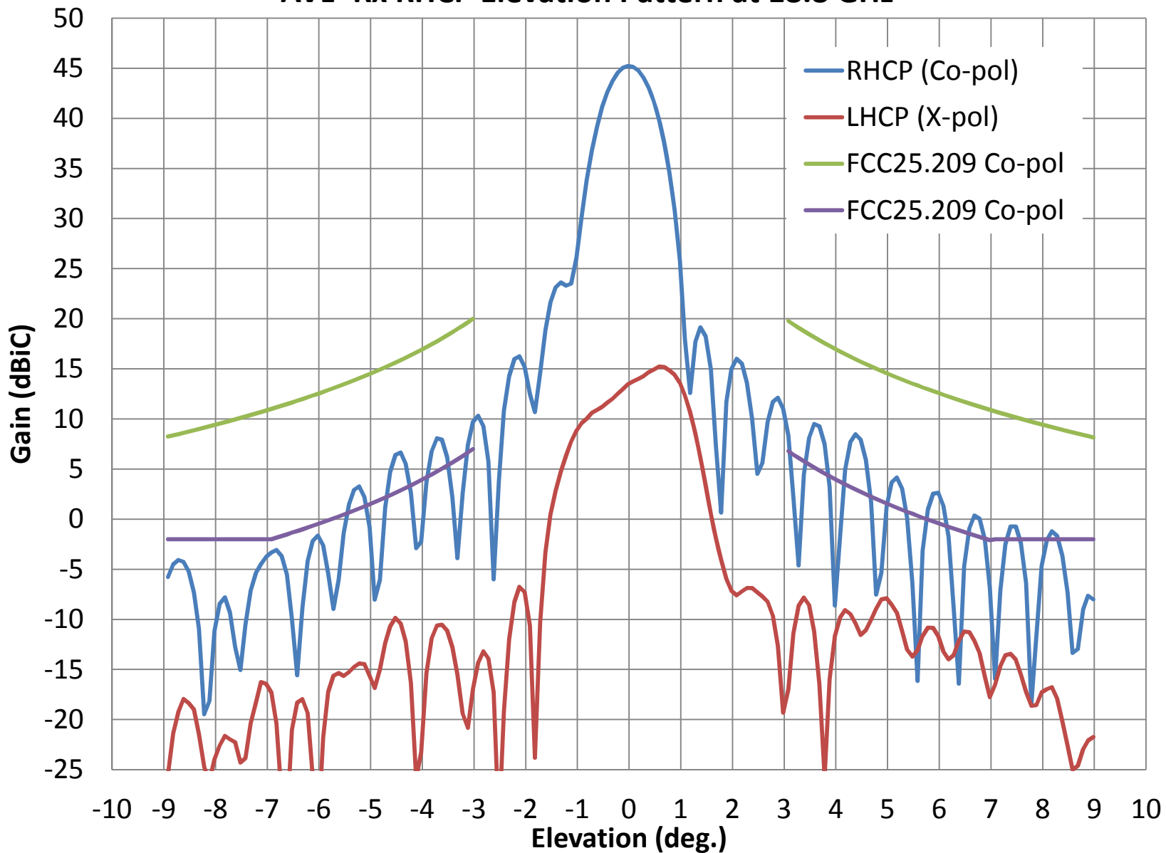
AVL- Rx RHCP Elevation Pattern at 18.8 GHz
