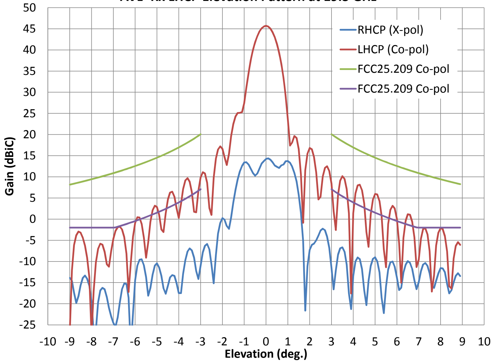
AVL- Rx LHCP Elevation Pattern at 19.3 GHz
