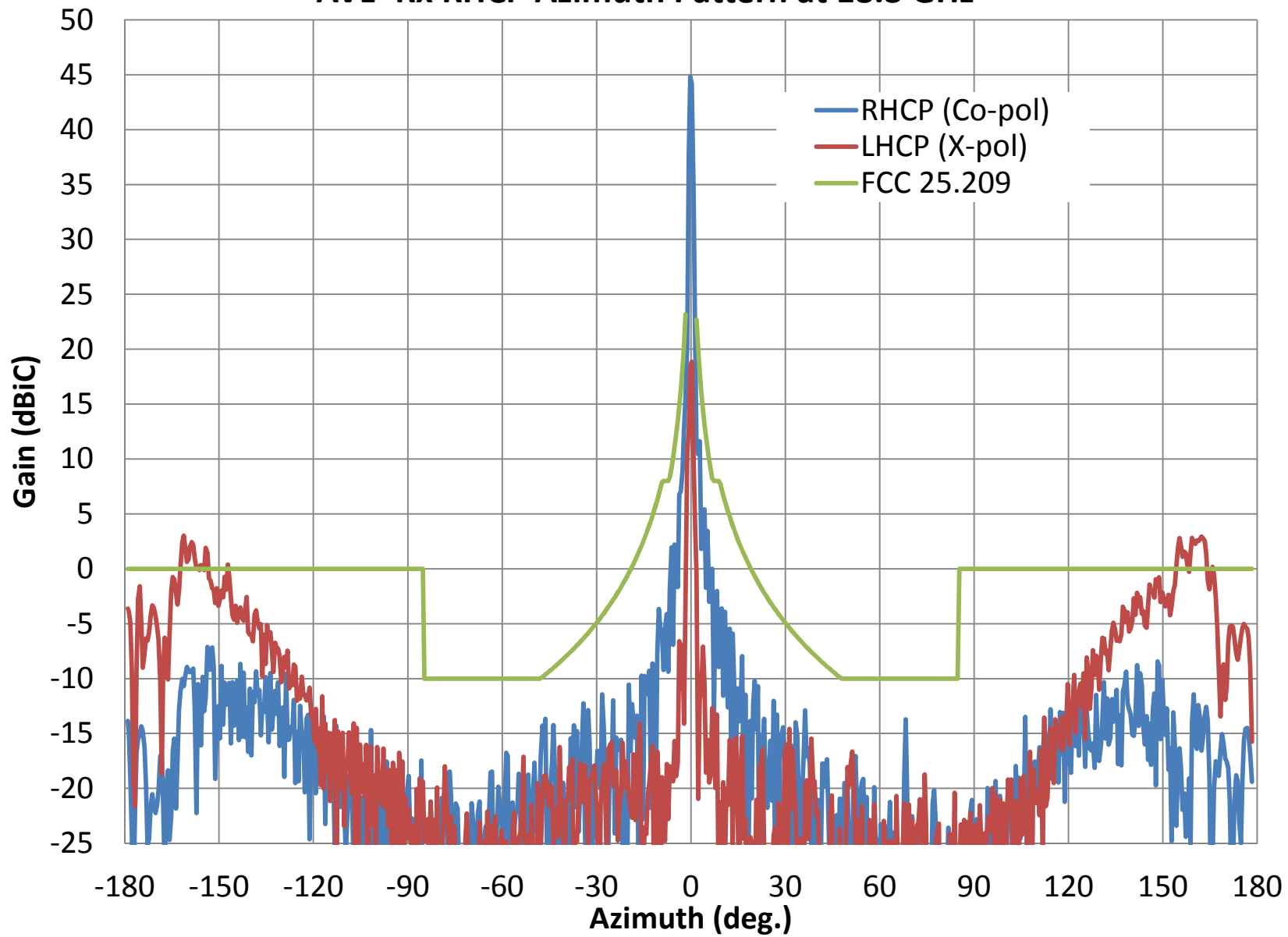
AVL- Rx RHCP Azimuth Pattern at 18.3 GHz
