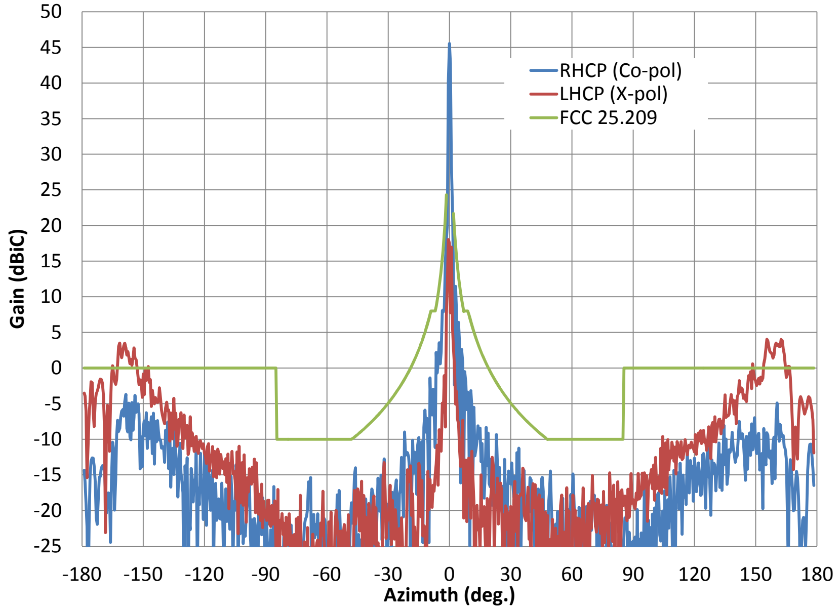
AVL- Rx RHCP Azimuth Pattern at 19.05 GHz
