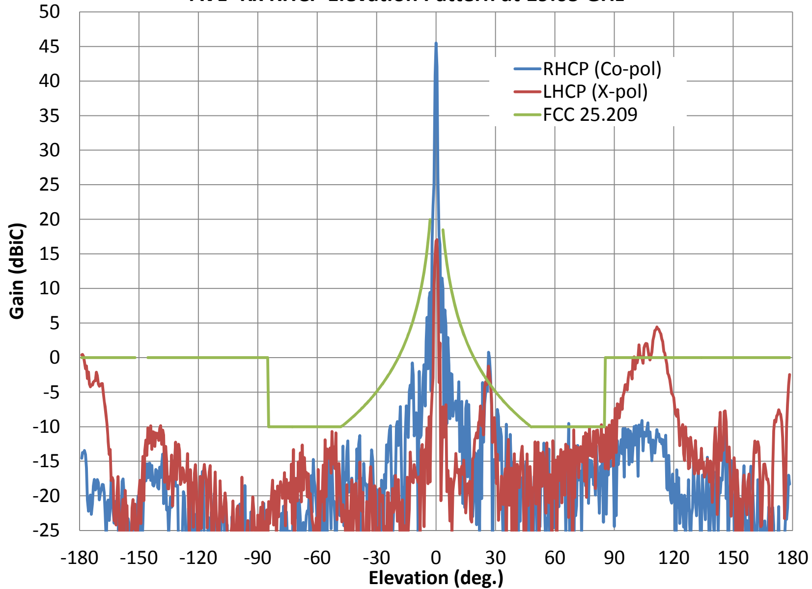
AVL- Rx RHCP Elevation Pattern at 19.05 GHz
