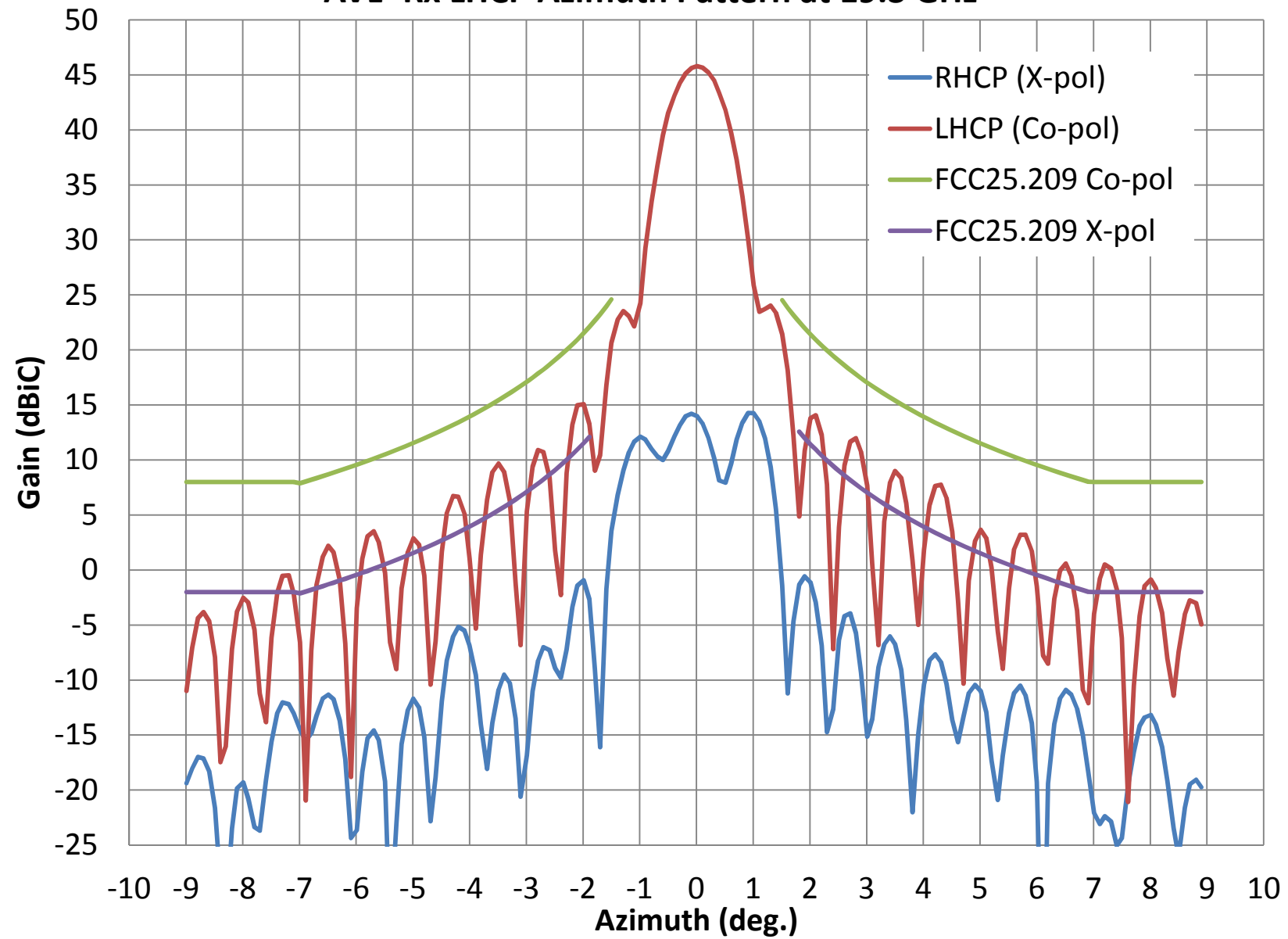
AVL- Rx LHCP Azimuth Pattern at 19.3 GHz
