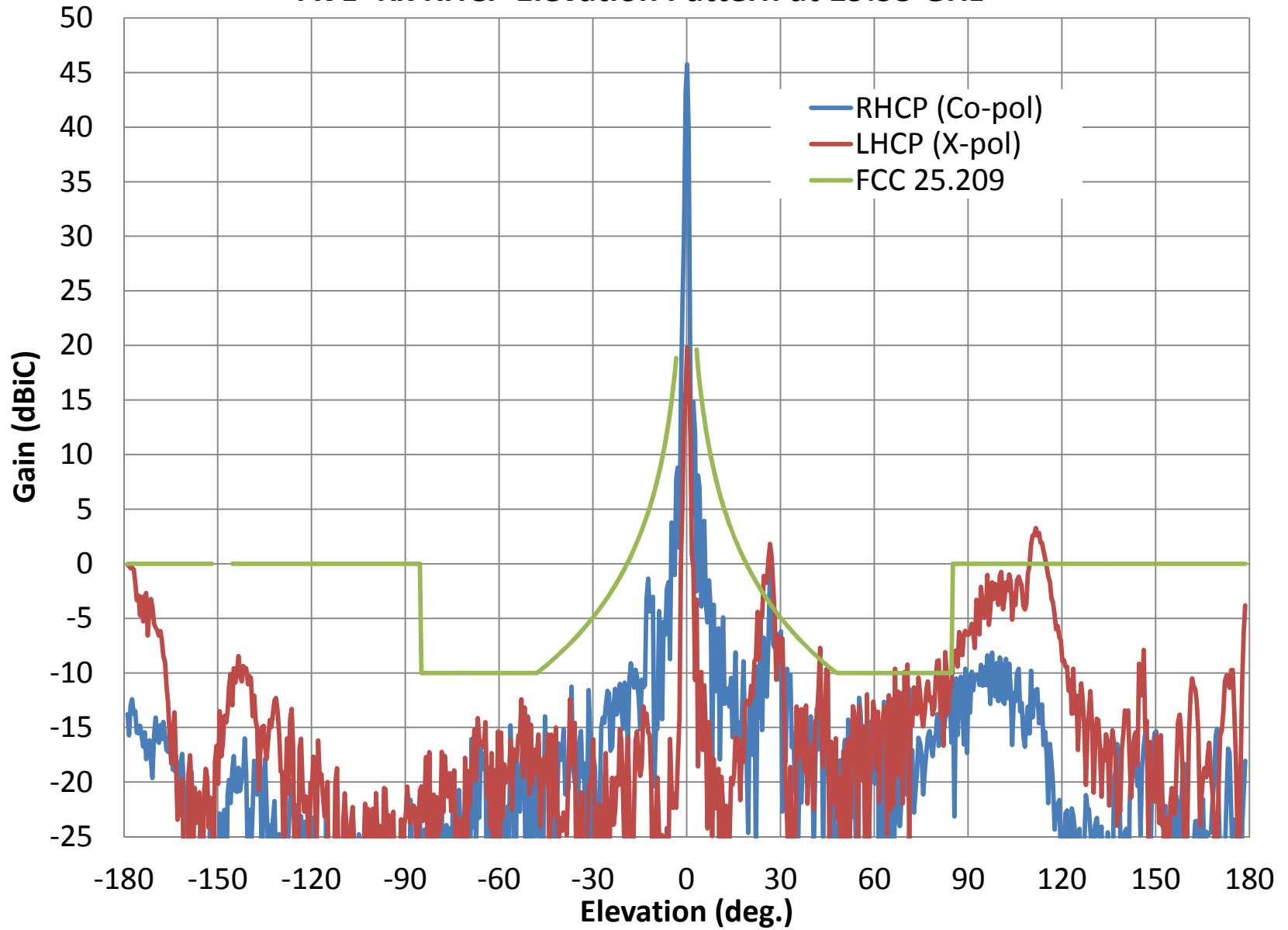
AVL- Rx RHCP Elevation Pattern at 19.95 GHz
