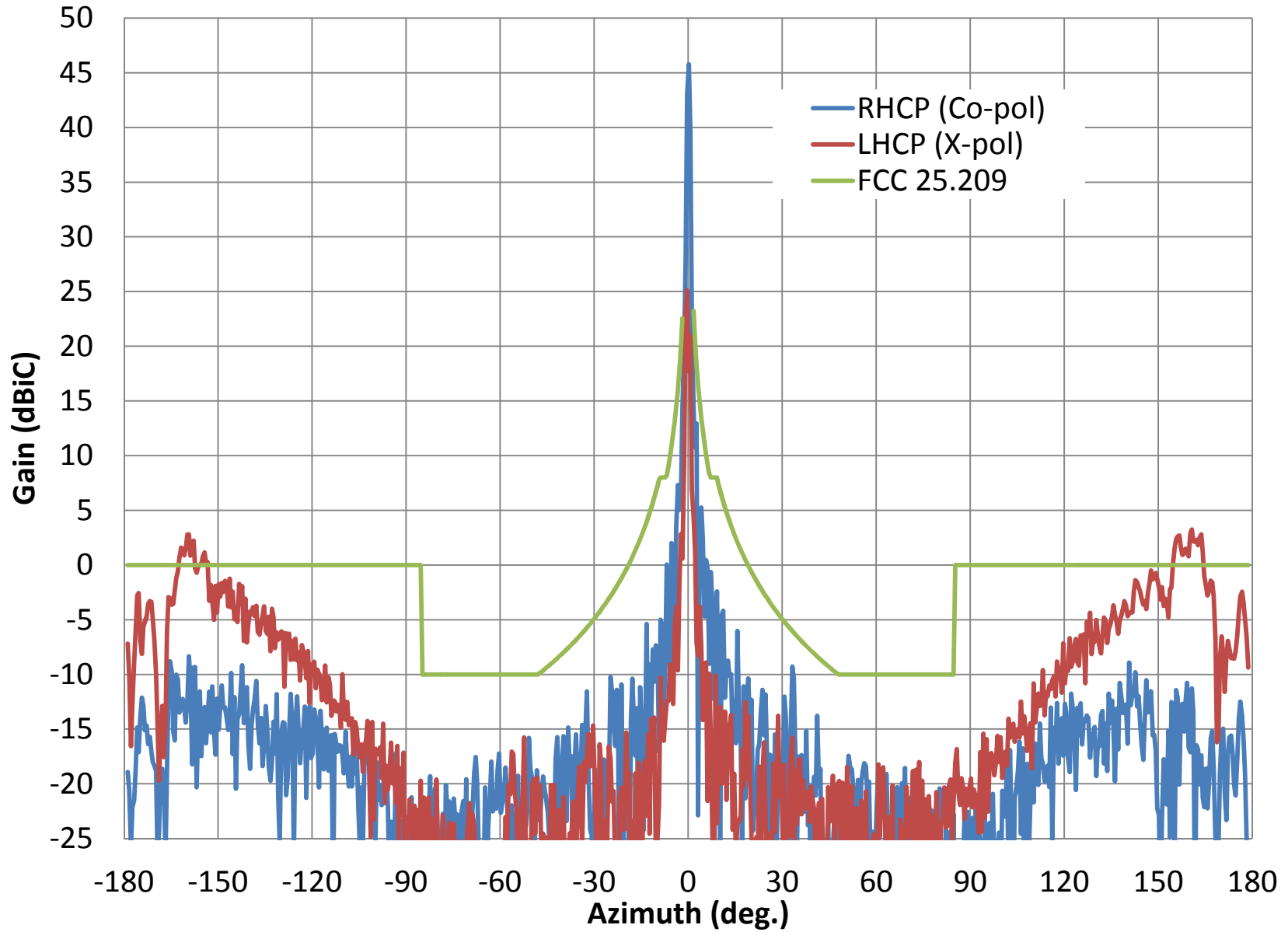
AVL- Rx RHCP Azimuth Pattern at 20.2 GHz
