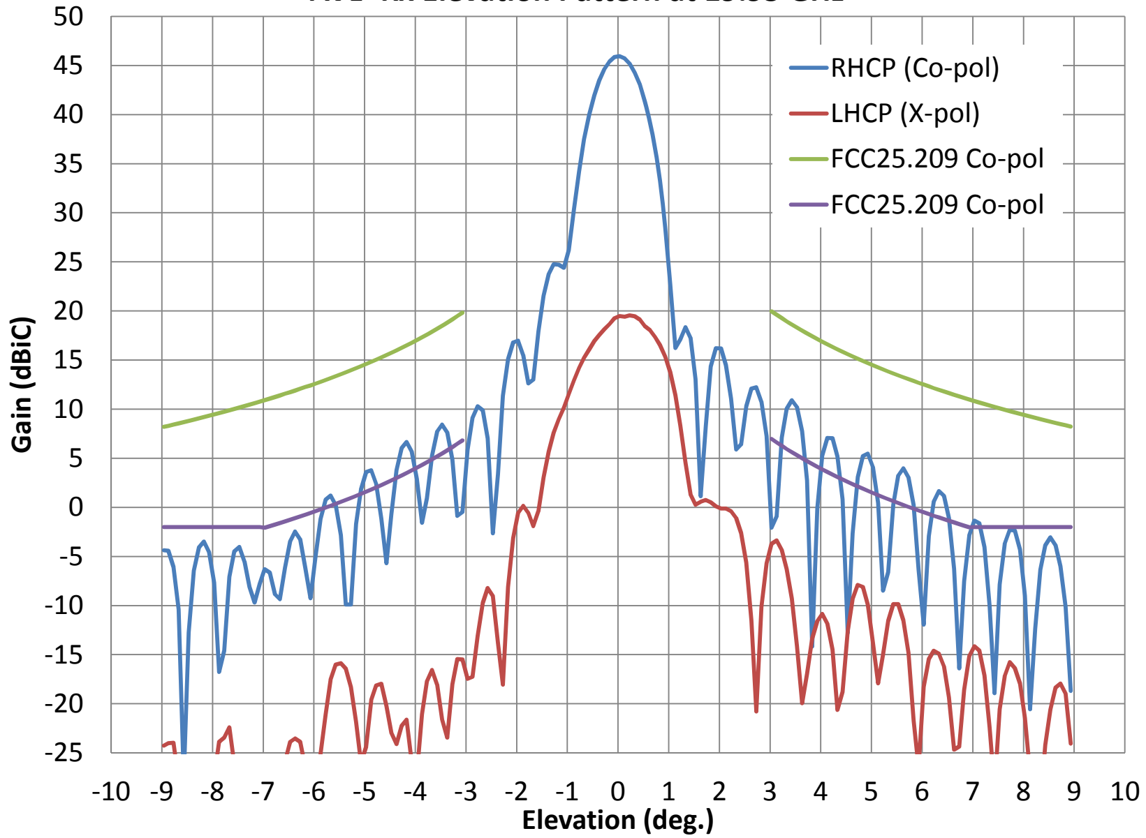
AVL- Rx Elevation Pattern at 19.95 GHz
