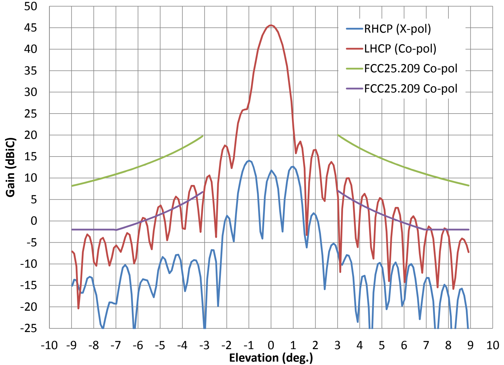
AVL- Rx LHCP Elevation Pattern at 19.7 GHz
