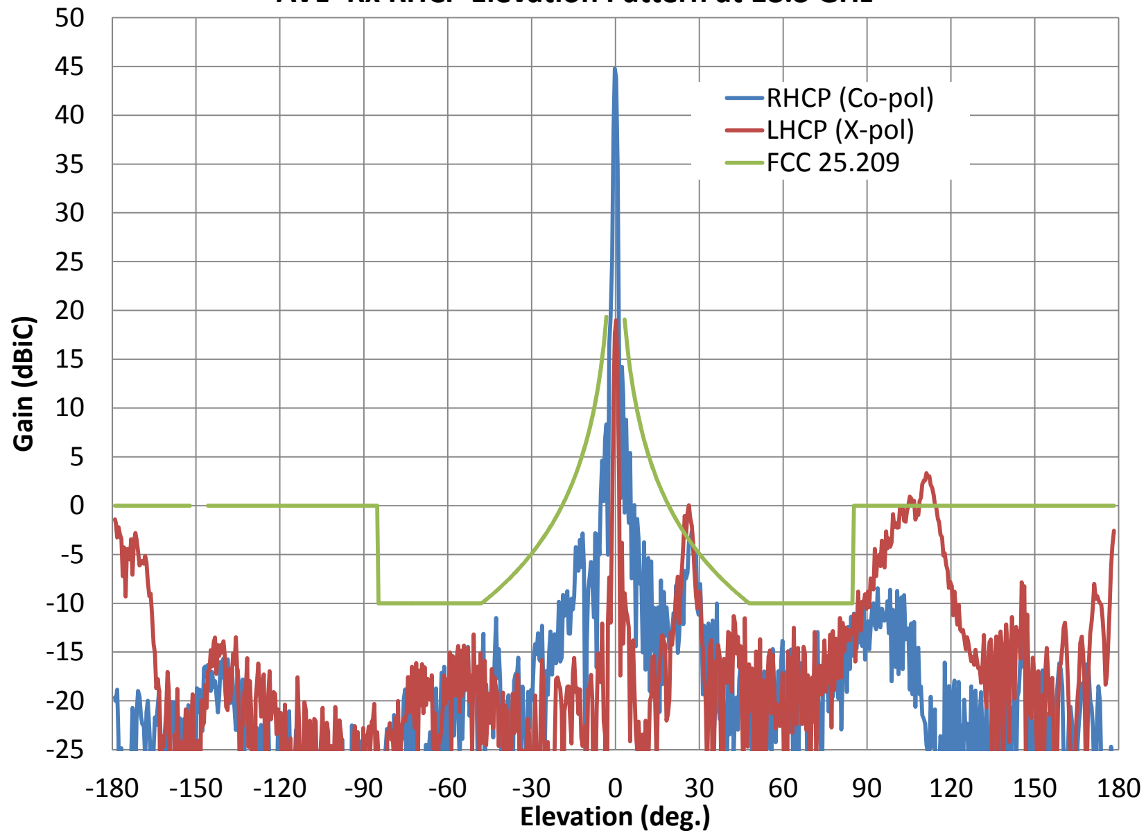
AVL- Rx RHCP Elevation Pattern at 18.3 GHz
