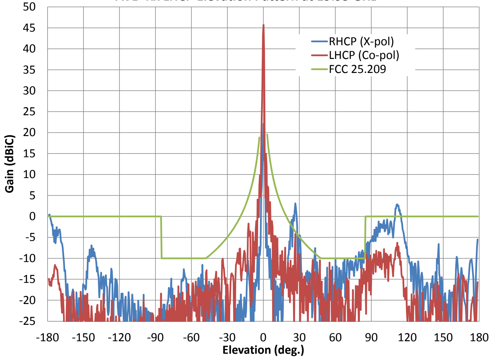
AVL- Rx LHCP Elevation Pattern at 19.95 GHz
