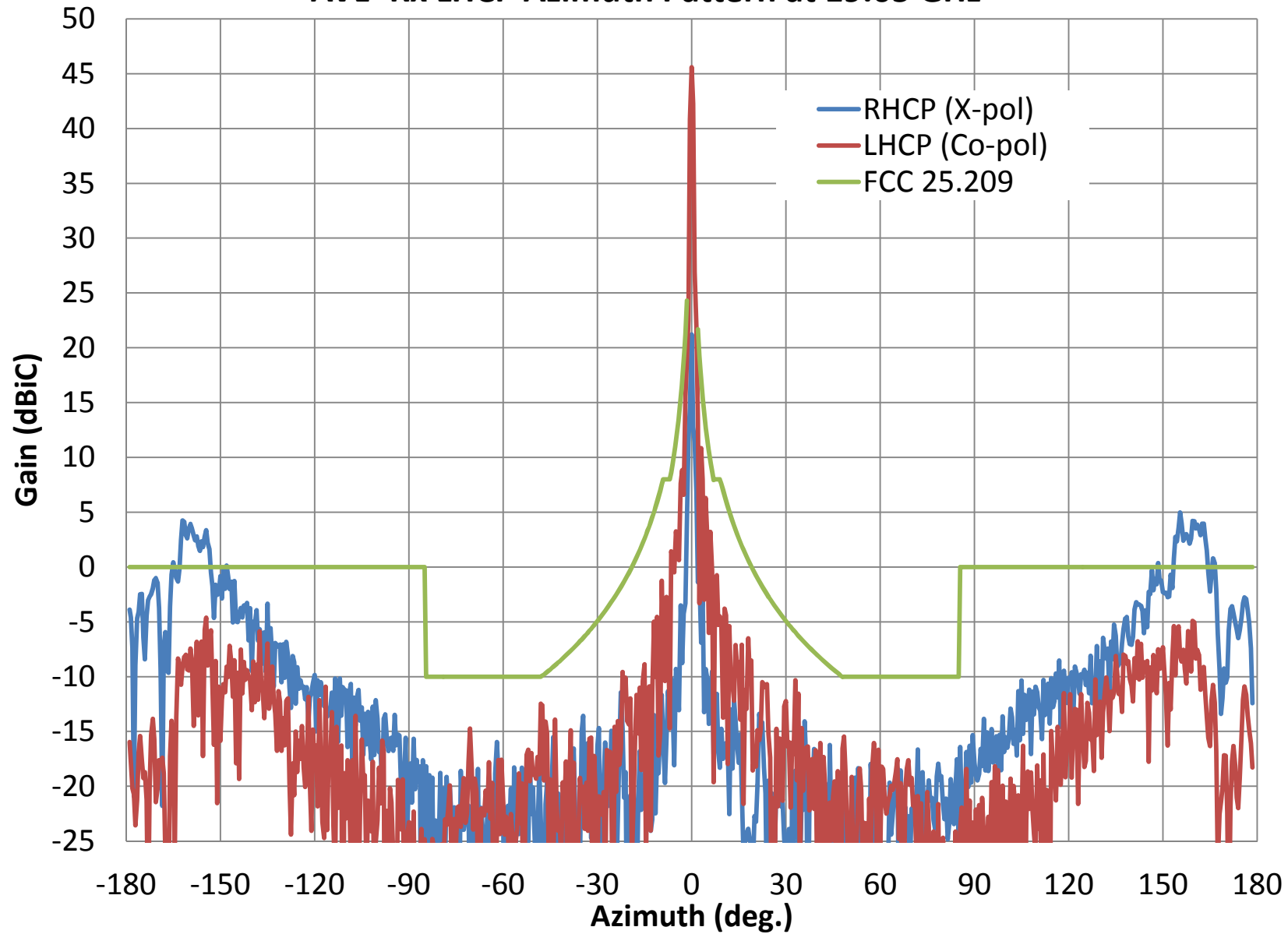
AVL- Rx LHCP Azimuth Pattern at 19.05 GHz
