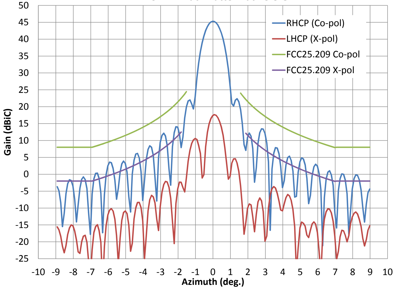
AVL- Rx RHCP Azimuth Pattern at 18.8 GHz
