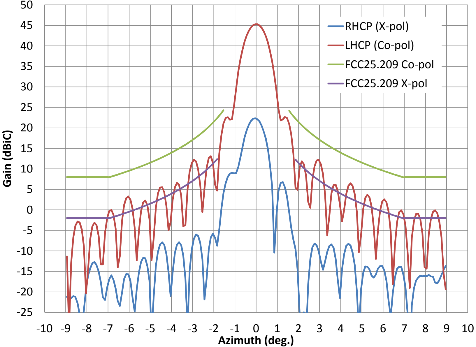
AVL- Rx LHCP Azimuth Pattern at 18.3 GHz
