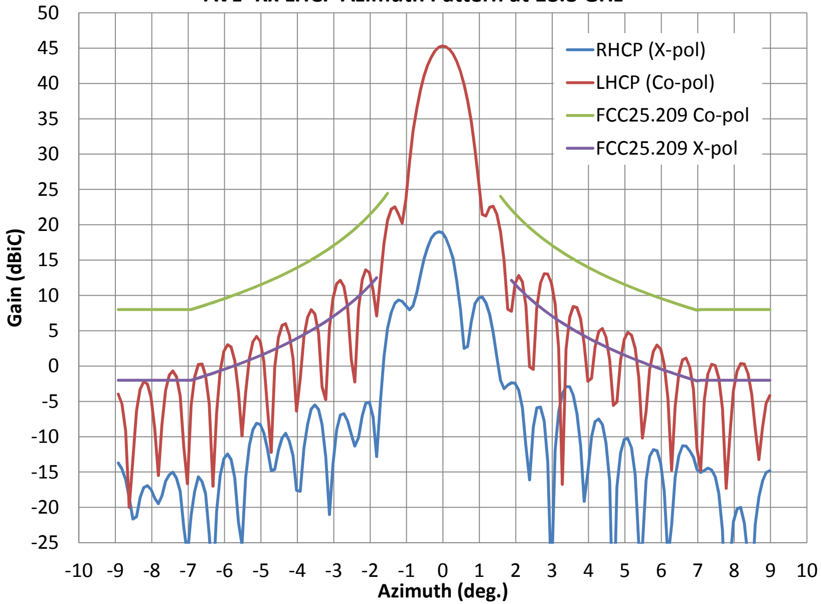
AVL- Rx LHCP Azimuth Pattern at 18.8 GHz
