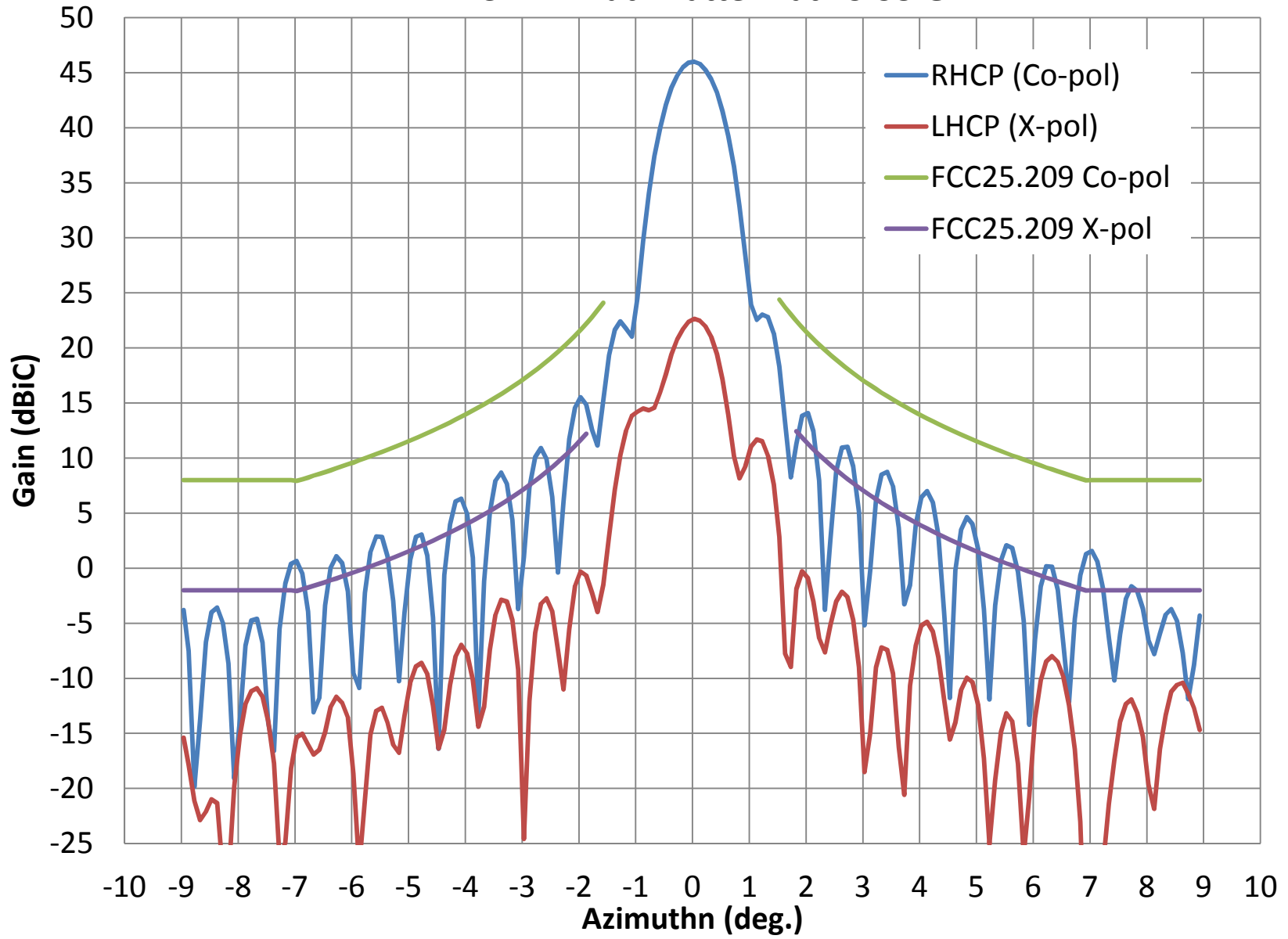
AVL- Rx RHCP Azimuth Pattern at 19.95 GHz
