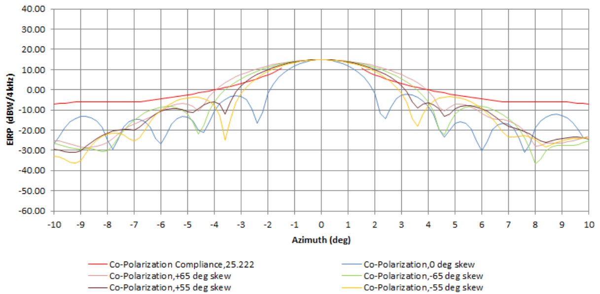
EIRP Density 14.25 GHz Horizontal Polarization, EIRP=38.8 dBW
