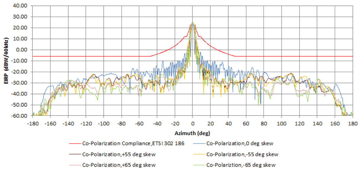
EIRP Density 14.25 GHz Horizontal Polarization, EIRP=38.8 dBW
