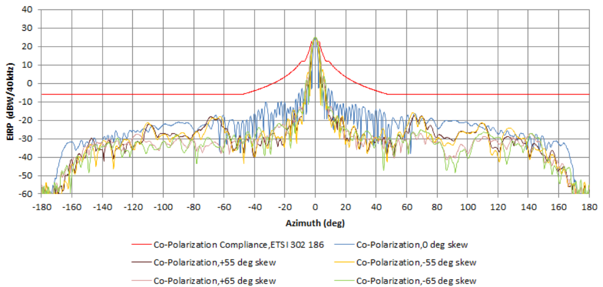
EIRP Density 14.47 GHz Horizontal Polarization, EIRP=38.8 dBW
