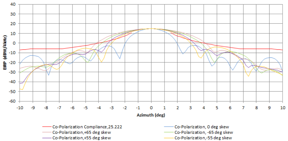
EIRP Density 14.05 GHz Vertical Polarization, EIRP=38.8 dBW
