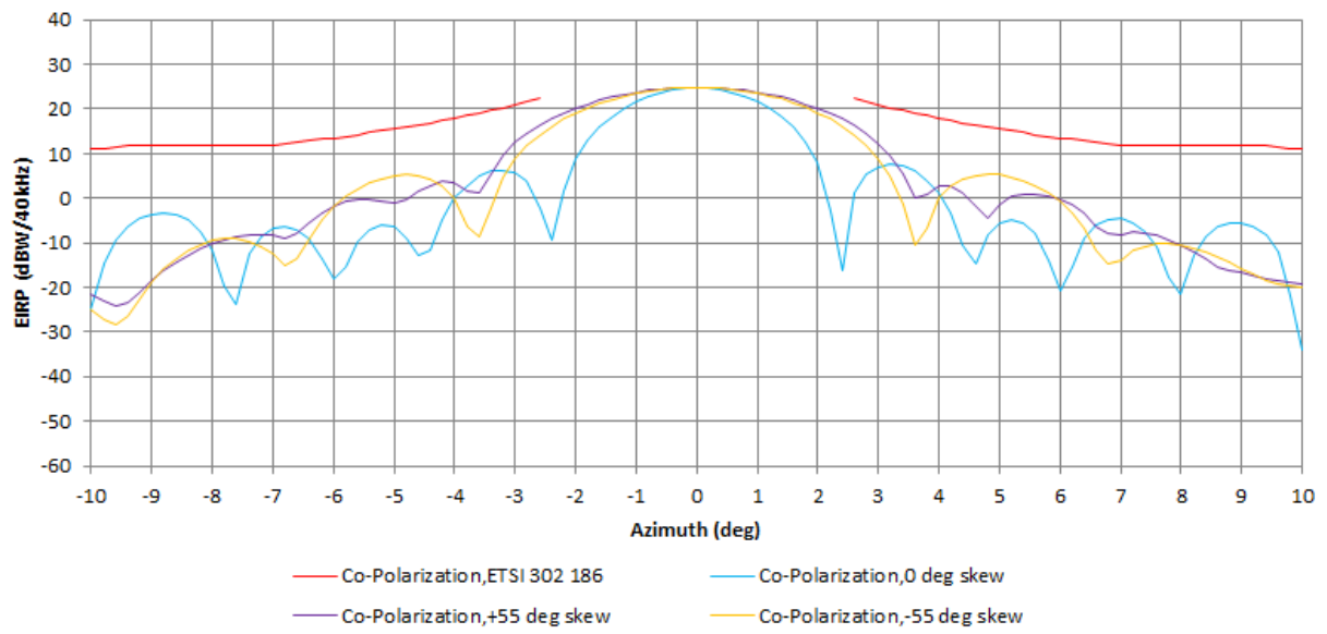
EIRP Density 14.25 GHz Vertical Polarization, EIRP=38.8 dBW
