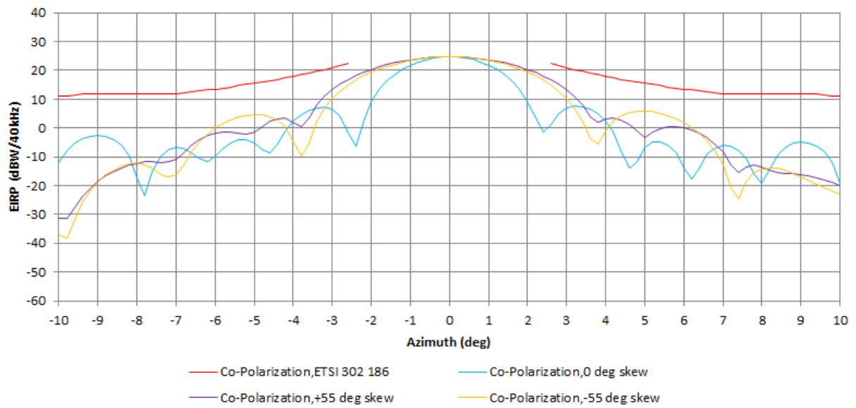
EIRP Density 14.05 GHz Vertical Polarization, EIRP=38.8 dBW
