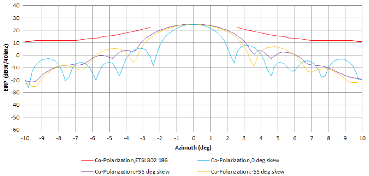
EIRP Density 14.47 GHz Vertical Polarization, EIRP=38.8 dBW
