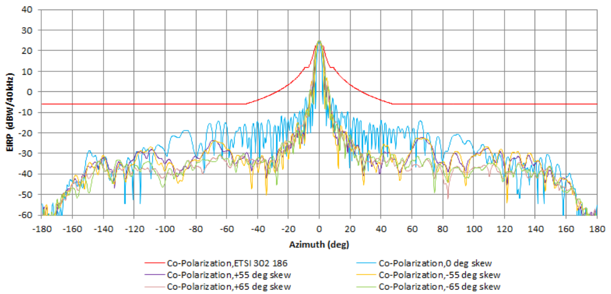
EIRP Density 14.47 GHz Vertical Polarization, EIRP=38.8 dBW
