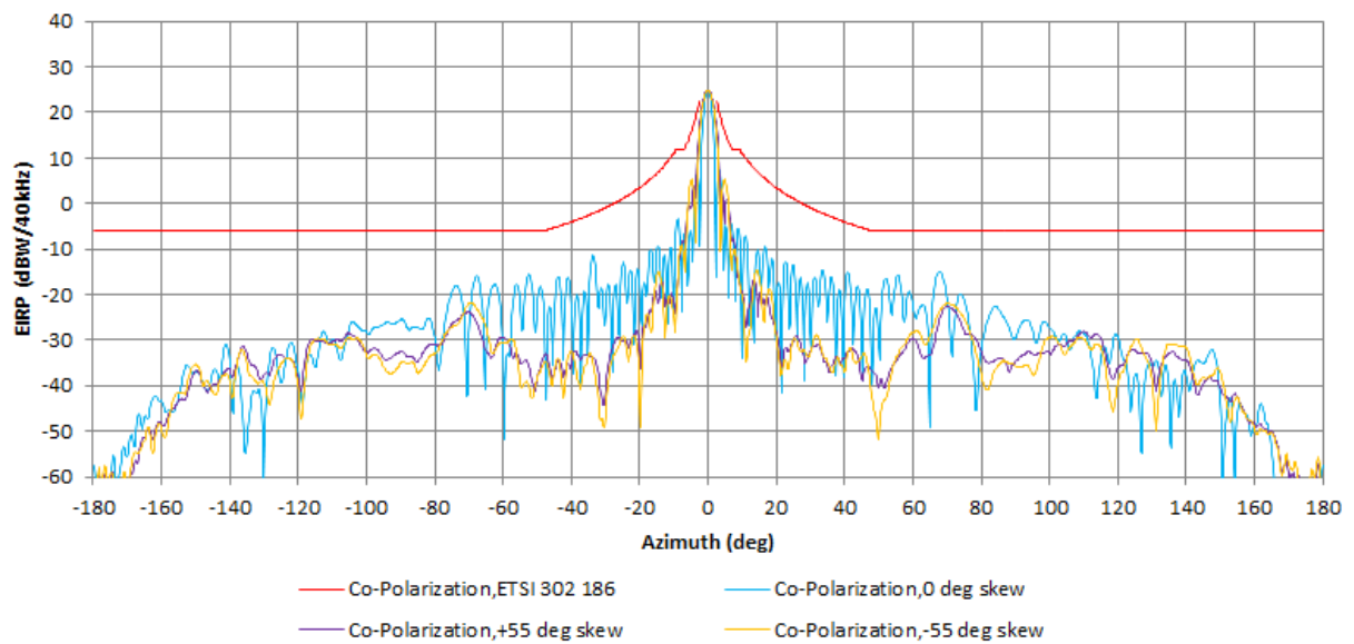
EIRP Density 14.25 GHz Vertical Polarization, EIRP=38.8 dBW
