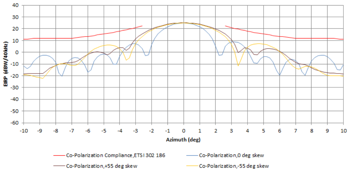
EIRP Density 14.47 GHz Horizontal Polarization, EIRP=38.8 dBW
