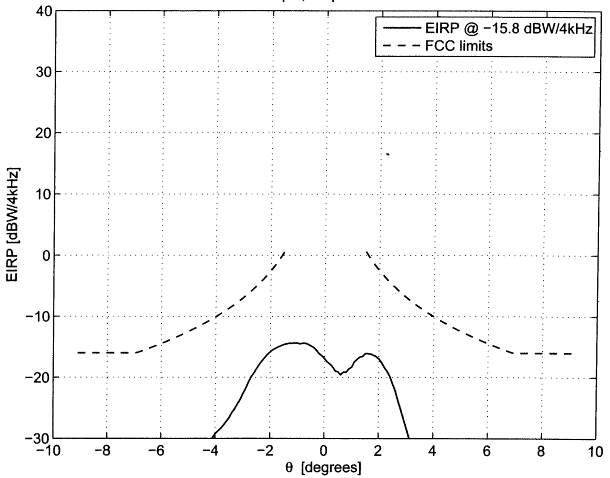
X-pol, freq=14 GHz
