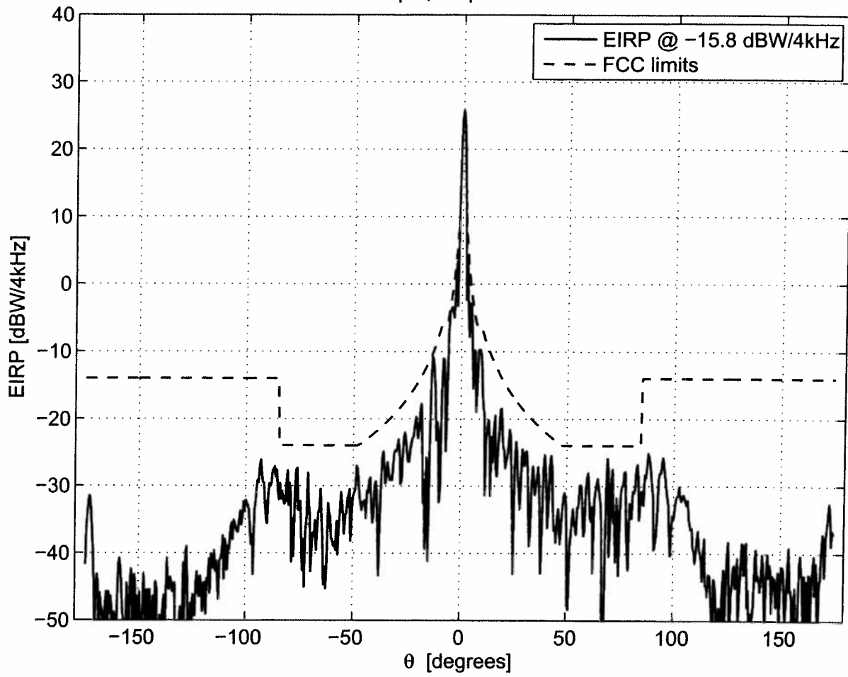
Co-pol, freq=14.5 GHz
