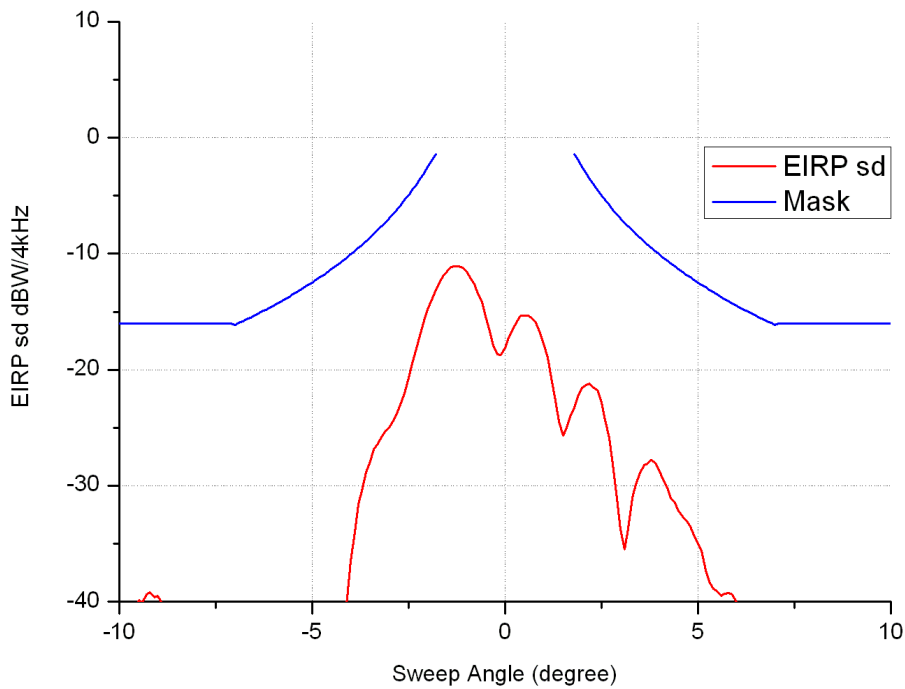
14.25 GHz @ -16.2 dBW/4kHz , 0.7dB Radome Loss
