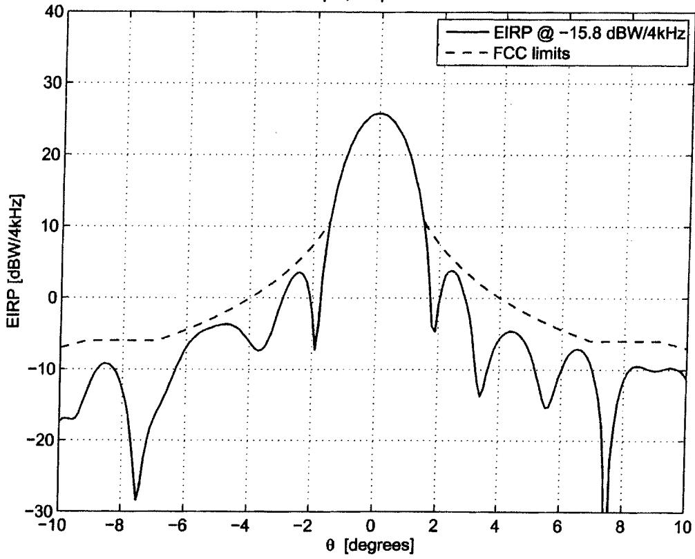
Co-pol, freq=14.25 GHz
