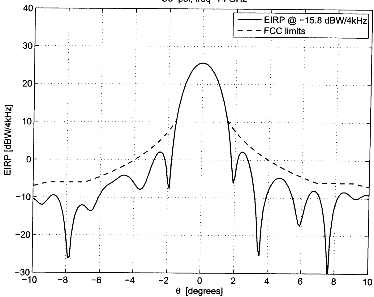
Co-pol, freq=14 GHz
