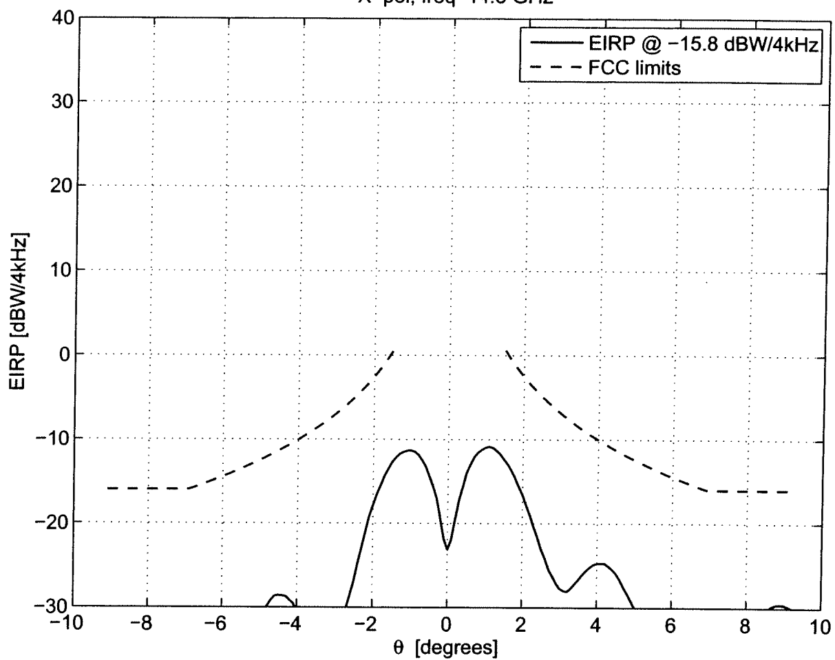
X-pol, freq=14.5 GHz
