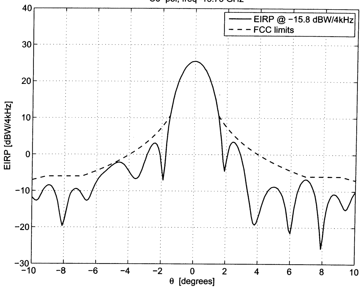
Co-pol, freq=13.75 GHz
