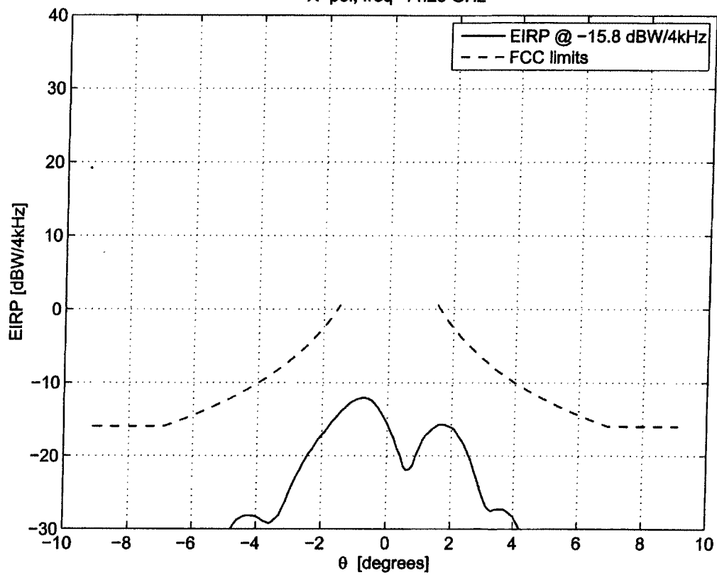
X-pol, freq=14.25 GHz
