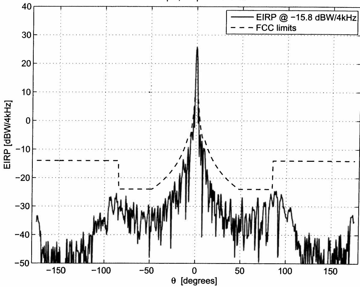
Co-pol, freq=14.25 GHz
