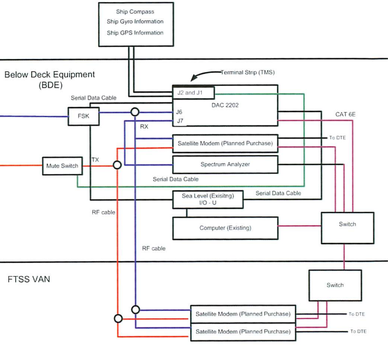
IEC Block Diagram Sea Tel 6009 ESV Terminal
