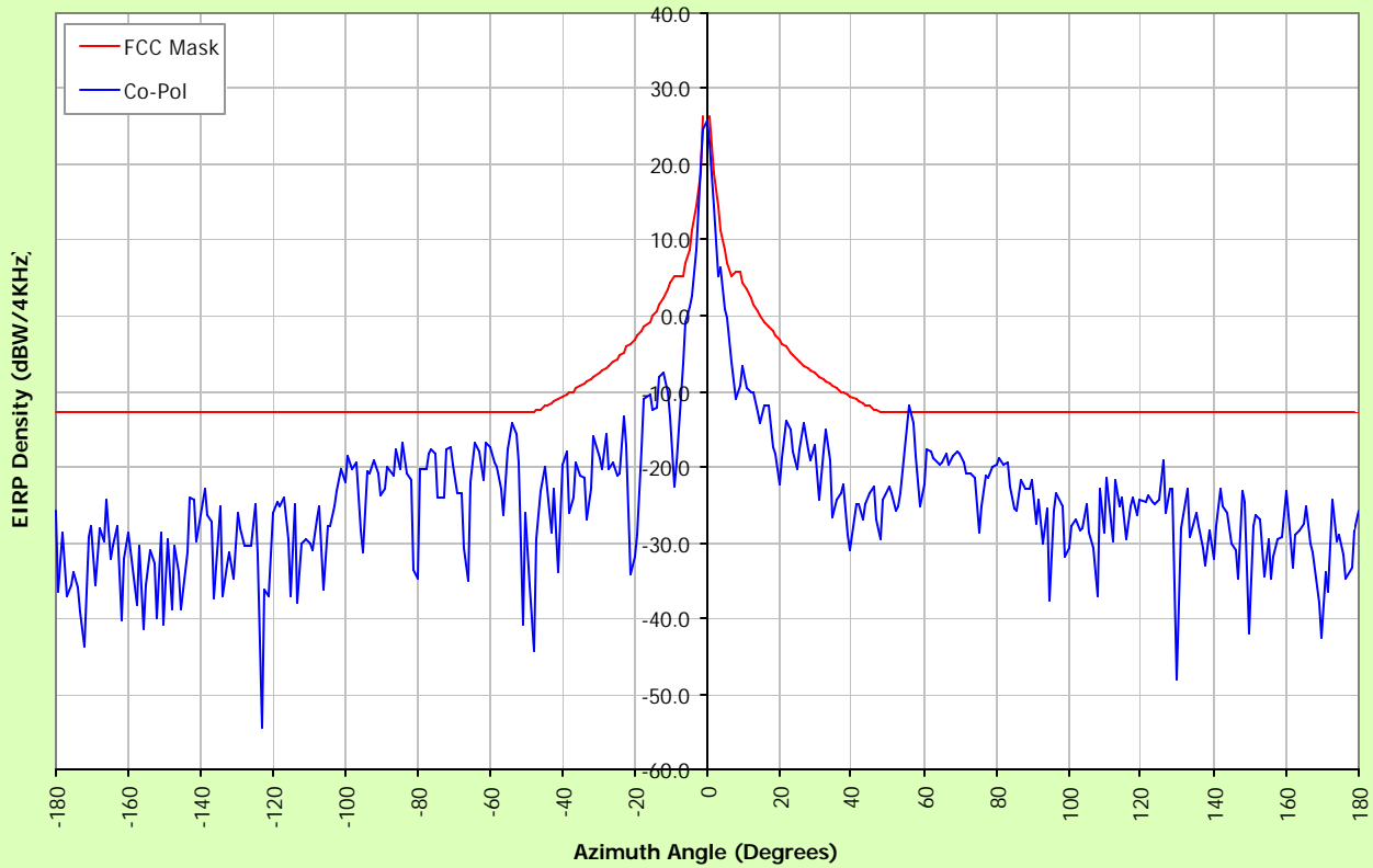
Co-Polarized E.I.R.P Density 128 Kbps IP Rate, Elevation=0°, Azimuth=-180° to 180°, F=6.175GHz
