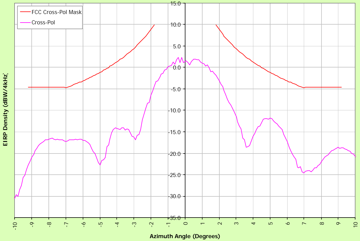
Cross Polarized E.I.R.P Density 512 Kbps IP Rate, Azimuth= -10° to 10°, Elevation = 0°, F=6.175GHz
