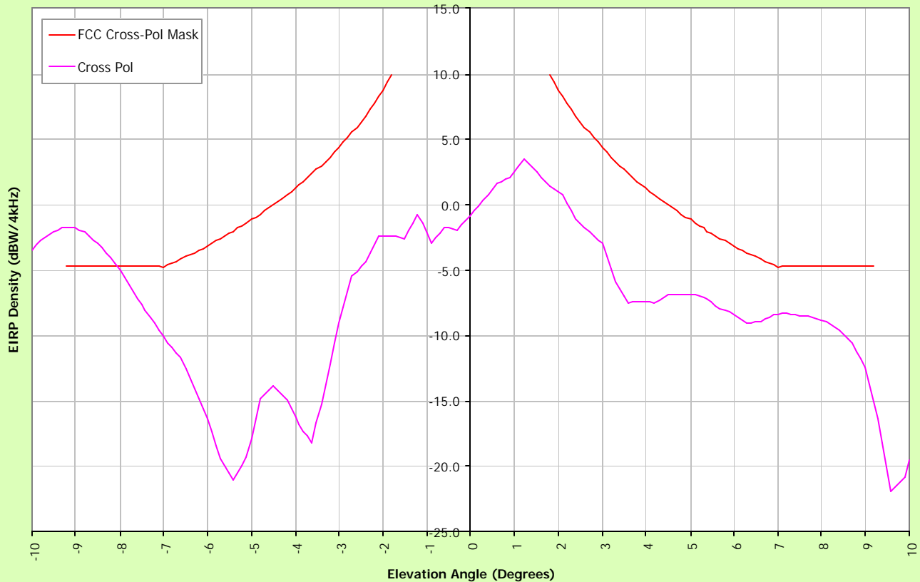
Cross Polarized E.I.R.P. Density 256 Kbps IP Rate, Azimuth = 0°, Elevation = -10° to 10°, F = 6.175GHz
