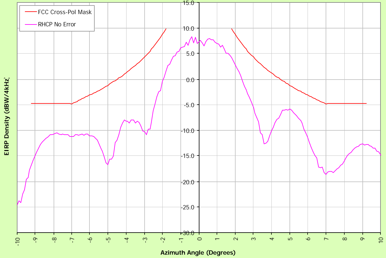
Cross Polarized E.I.R.P Density 128 Kbps IP Rate, Azimuth= -10° to 10°, Elevation = 0°, F=6.175GHz
