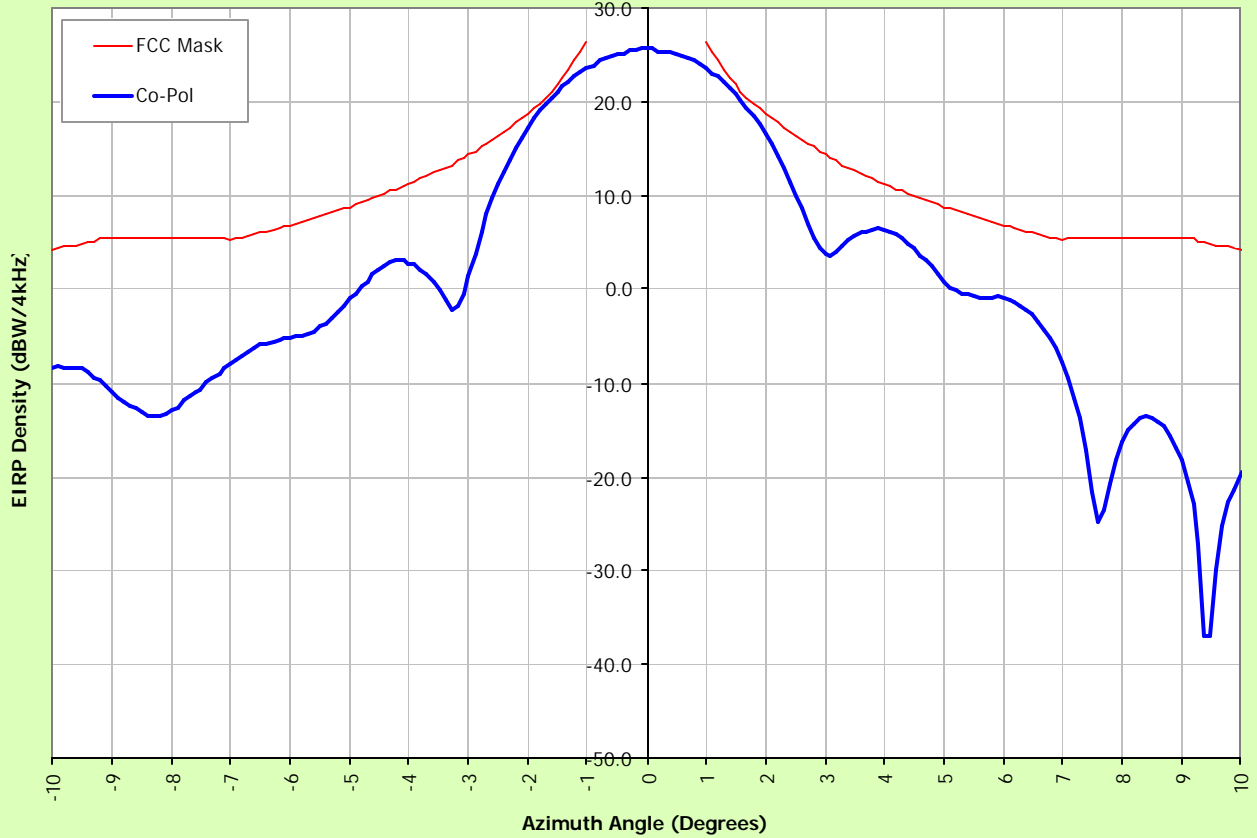
Co-Polarized E.I.R.P Density 128 Kbps IP Rate, Azimuth= -10° to 10°, F=6.175GHz
