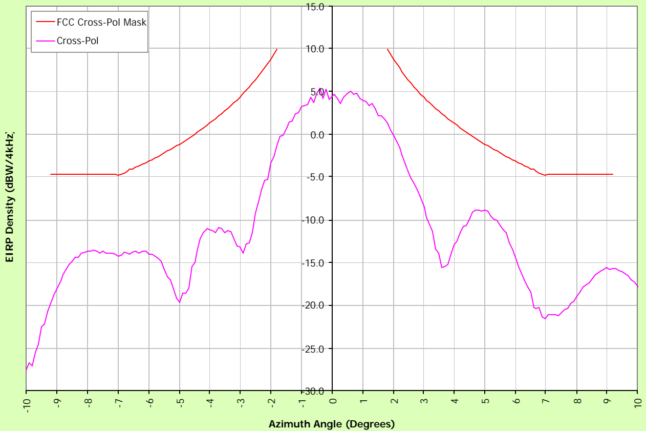
Cross Polarized E.I.R.P Density 256 Kbps IP Rate, Azimuth= -10° to 10°, Elevation = 0°, F=6.175GHz
