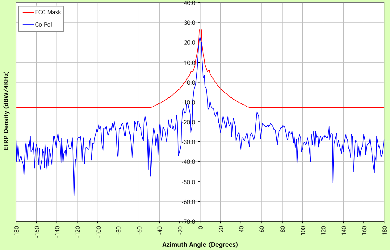
Co-Polarized E.I.R.P Density 256 Kbps IP Rate, Elevation=0°, Azimuth=-180° to 180°, F=6.175GHz
