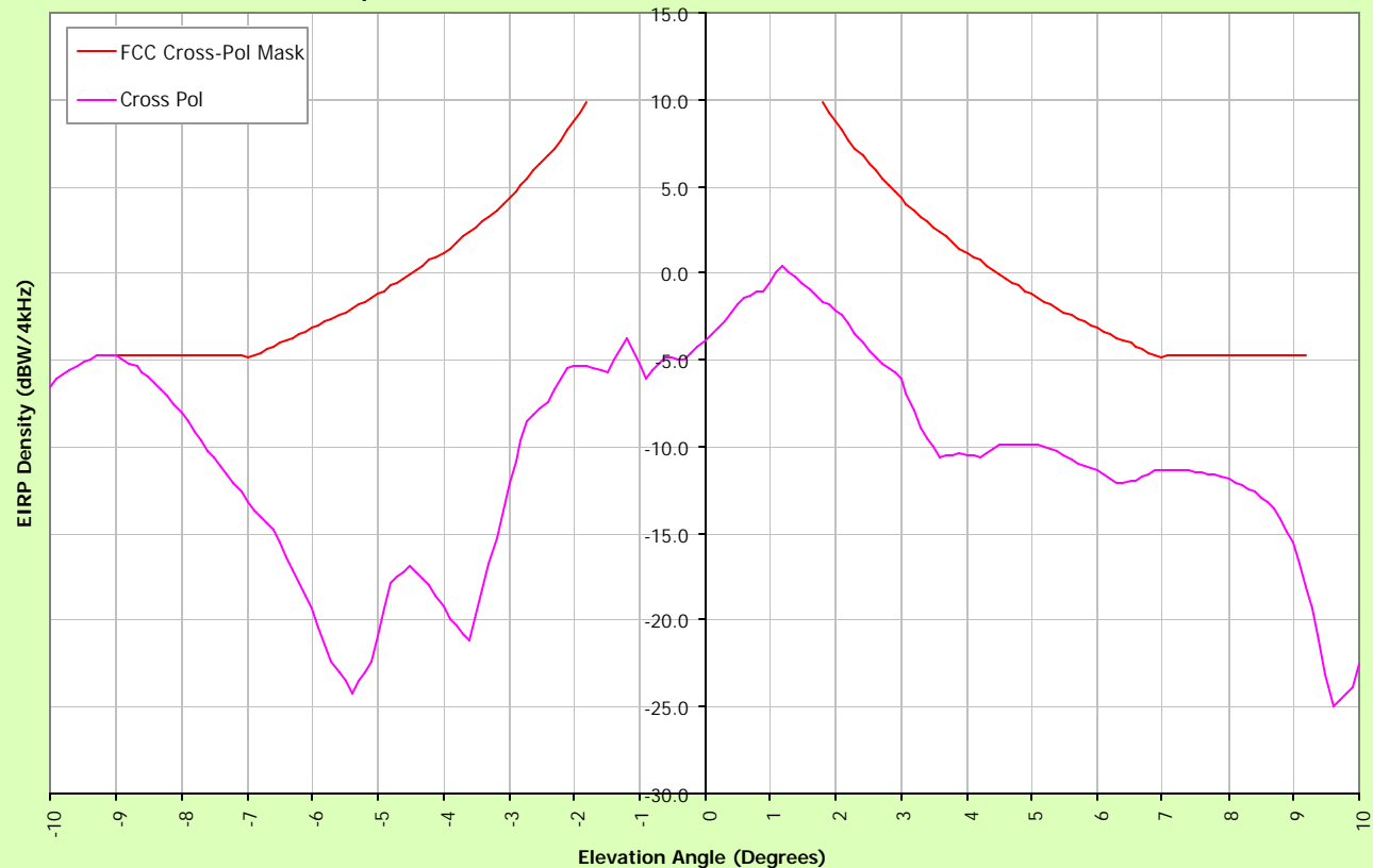
Cross Polarized E.I.R.P. Density 512 Kbps IP Rate, Azimuth = 0°, Elevation = -10° to 10°, F = 6.175GHz
