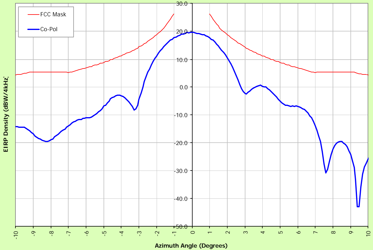
Co-Polarized E.I.R.P Density 512 Kbps IP Rate, Azimuth= -10° to 10°, F=6.175GHz
