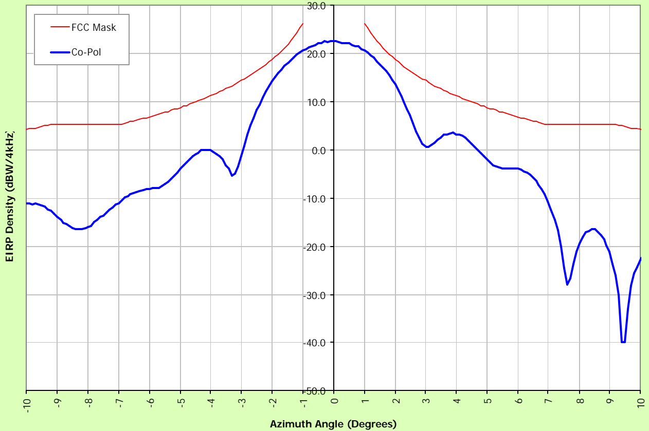
Co-Polarized E.I.R.P Density 256 Kbps IP Rate, Azimuth= -10° to 10°, F=6.175GHz
