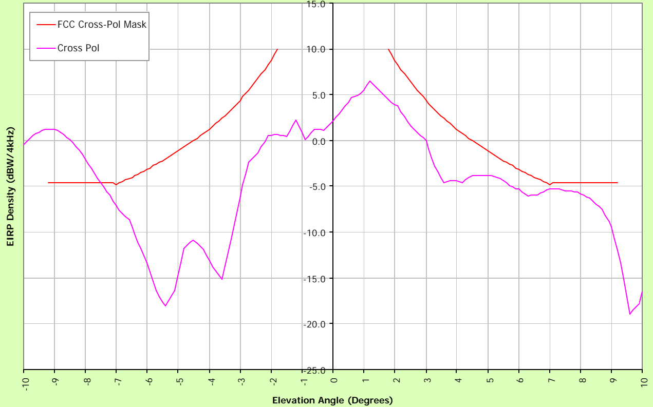
Cross Polarized E.I.R.P Density 128 Kbps IP Rate, Azimuth = 0°, Elevation = -10° to 10°, F = 6.175GHz
