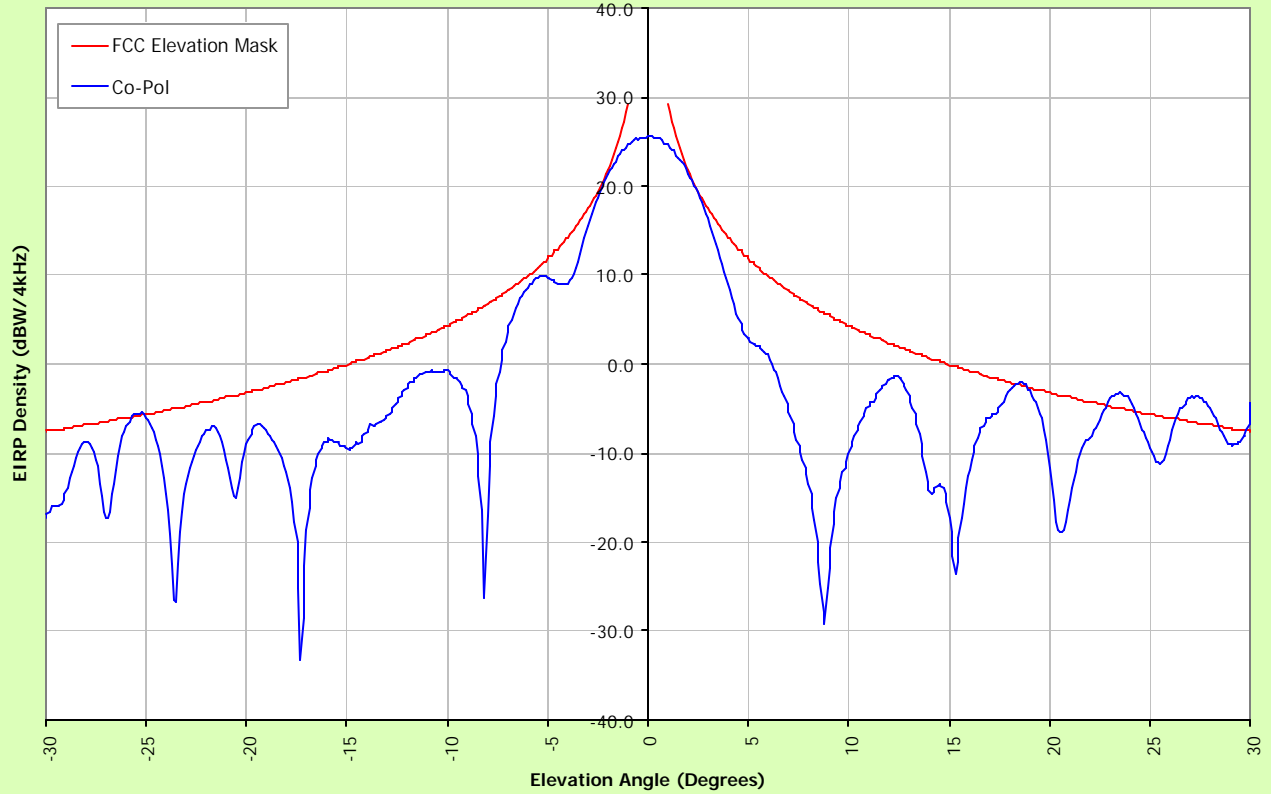
Co-Polarized E.I.R.P Density 128 Kbps IP Rate, Azimuth = 0°, Elevation = -30° to 30°, F = 6.175GHz
