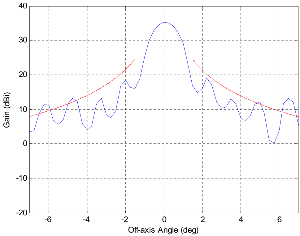
Figure 7. Tx Pattern @ 14.05GHz, Polarity: H, Plane: Co, Elevation: 5°, Azimuth Cut
