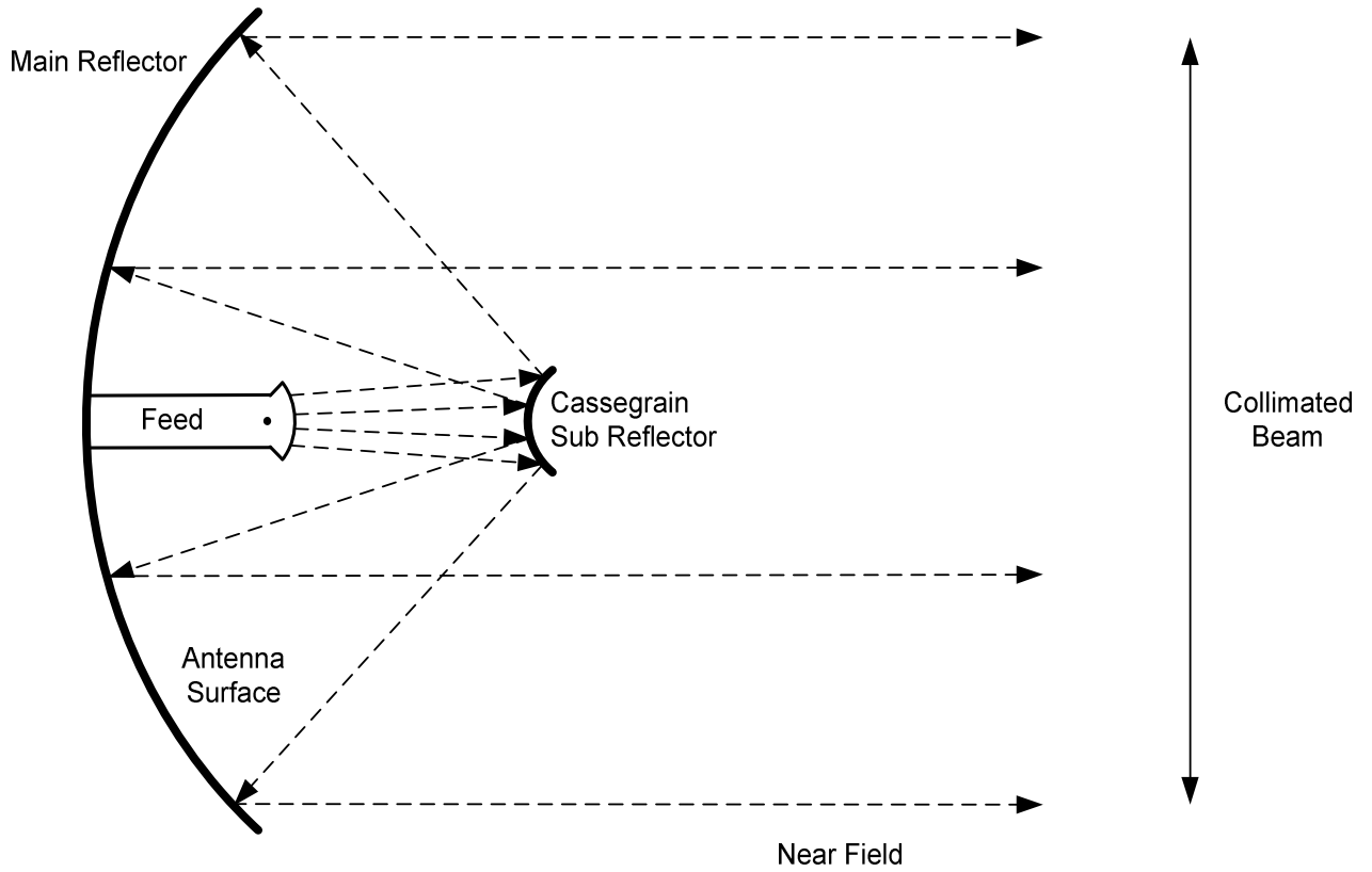
Figure 1. 9.0 meter Dual Optics Satellite Antenna
