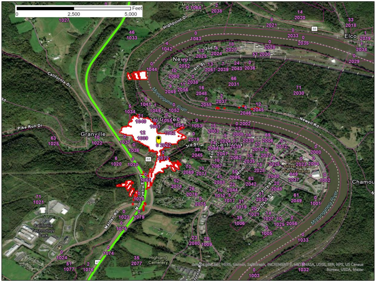
Figure 1 – California, PA SAN -77.6 dB(mW/(m2 * MHz)) pfd contour
