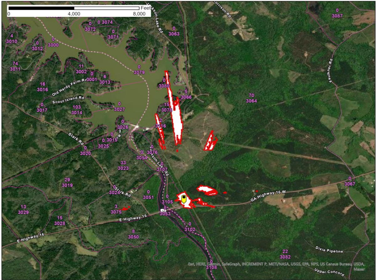
Figure 1 – Monticello, GA SAN -77.6 dB(mW/(m2 * MHz)) pfd contour
