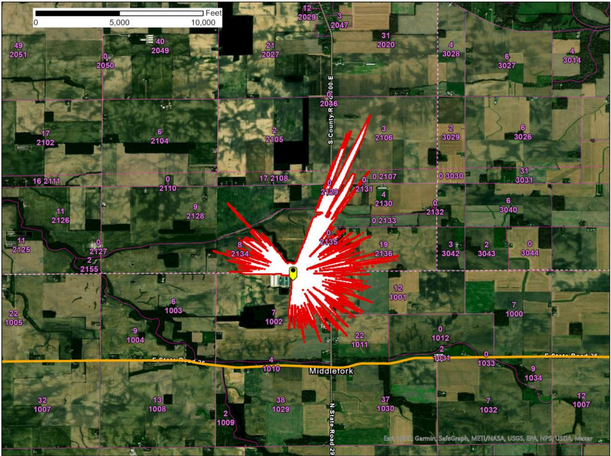
Figure 1 – Frankfort, IN SAN -77.6 dB(mW/(m 2 * MHz)) pfd contour
