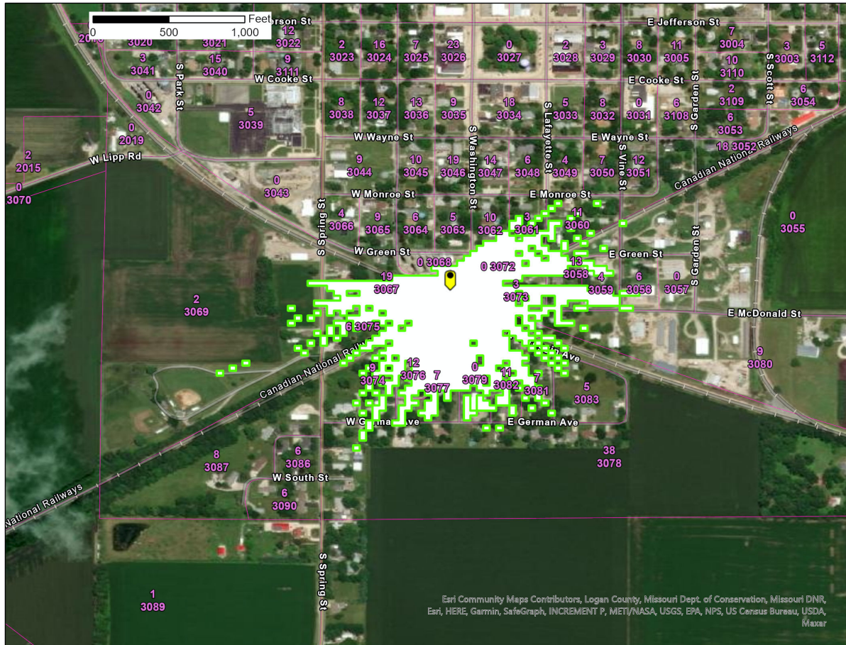
Figure 1 – Pulaski, IL SAN -77.6 \text{ dB(mW/(m}^2 * \text{MHz))} pfd contour
