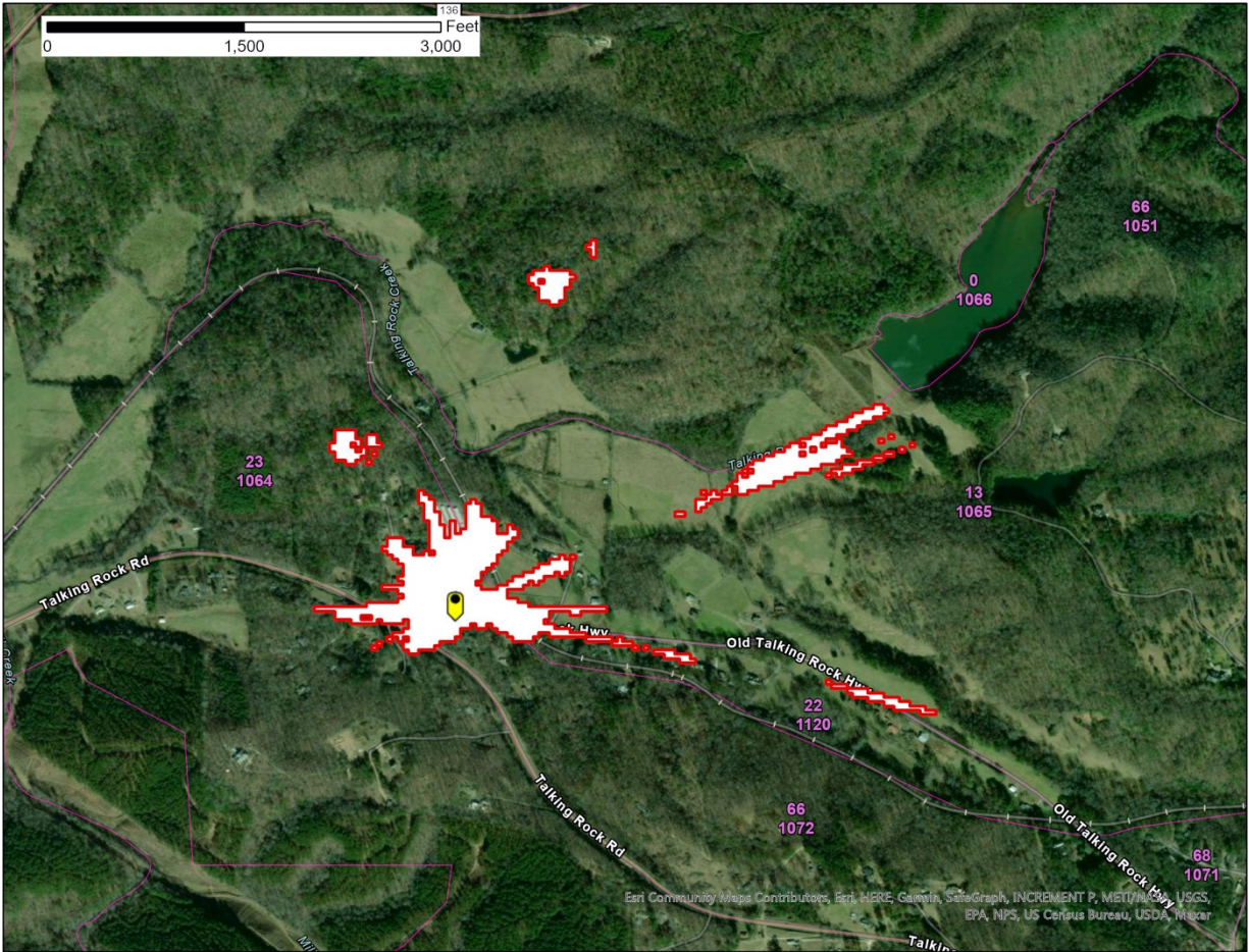
Figure 1 – Talking Rock, GA SAN -77.6 dB(mW/(m2 * MHz)) pfd contour
