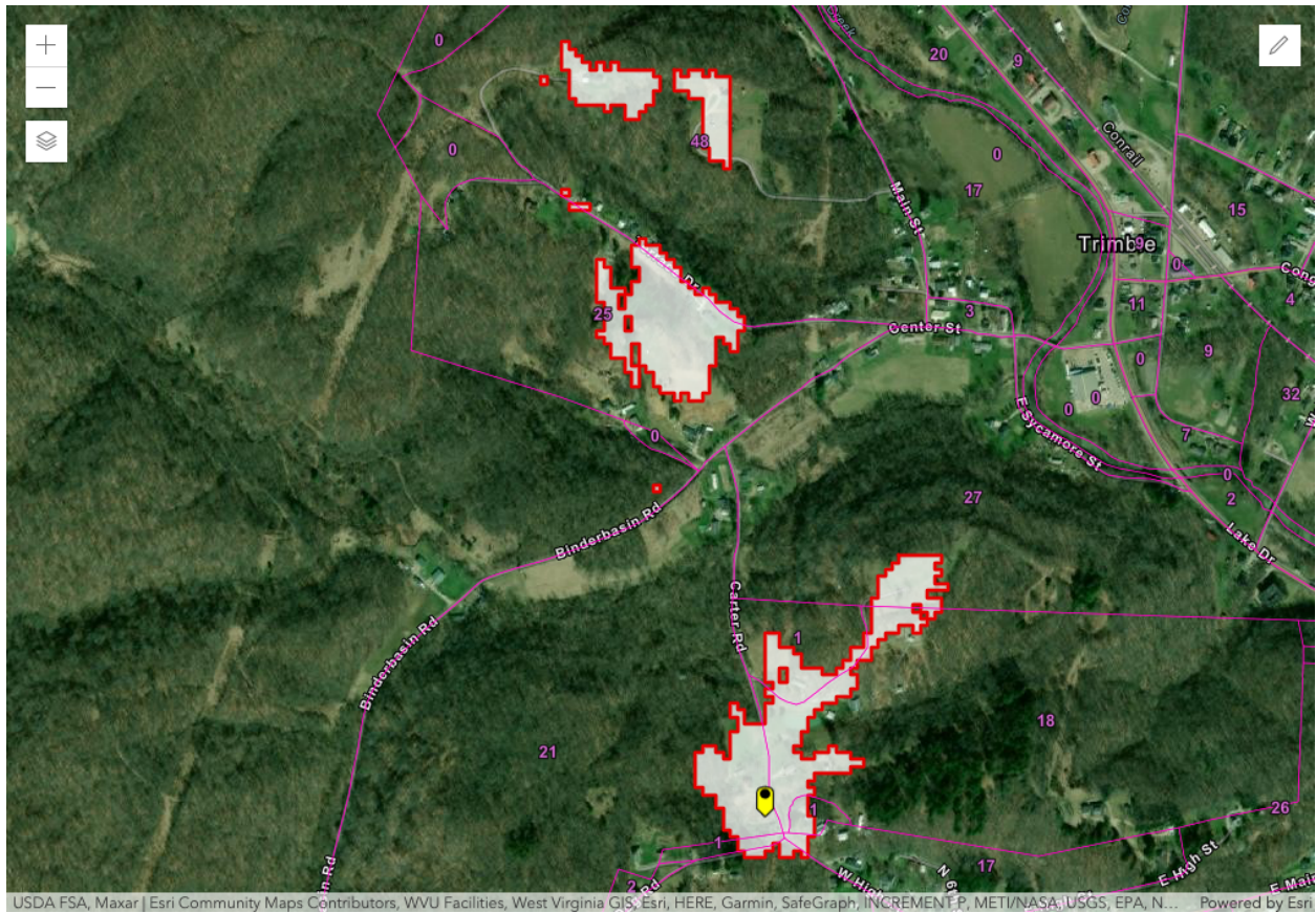
Figure 1 – Jacksonville, OH SAN -77.6 dB(mW/(m 2 * MHz)) pfd contour
