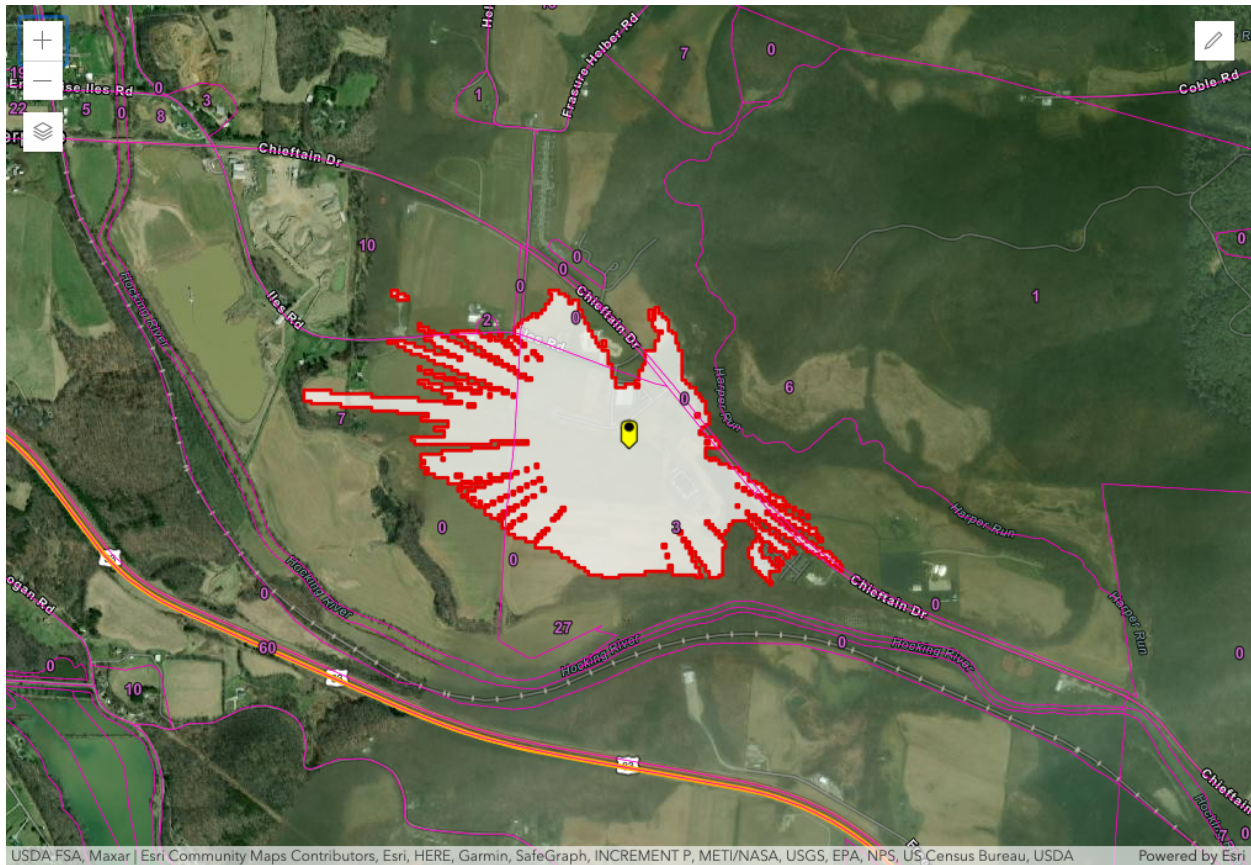
Figure 1 – Logan, OH SAN -77.6 dB(mW/(m 2 * MHz)) pfd contour
