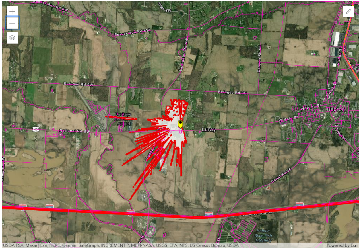
Figure 1 – Hebron, OH SAN -77.6 dB(mW/(m 2 * MHz)) pfd contour
