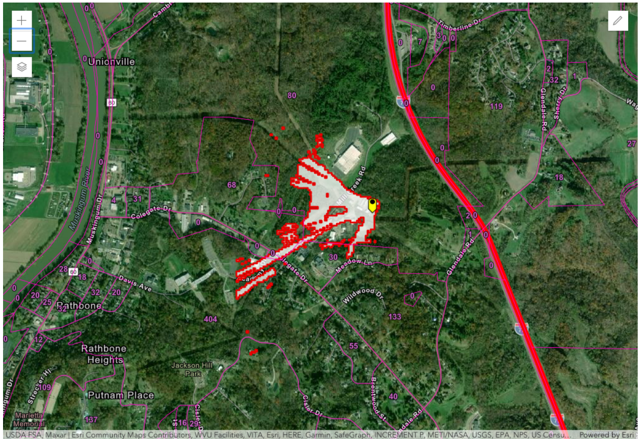
Figure 1 – Marietta, OH SAN -77.6 dB(mW/(m 2 * MHz)) pfd contour
