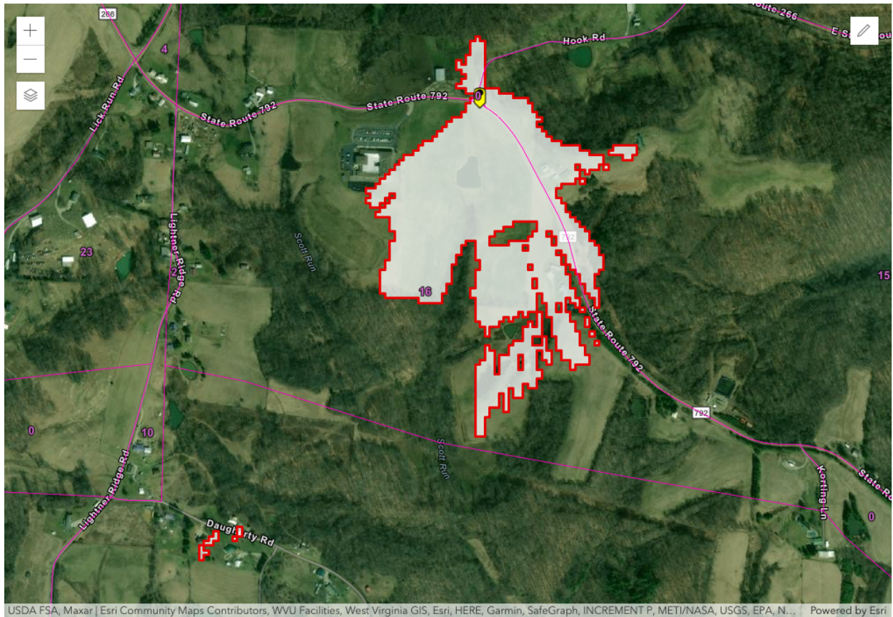
Figure 1 – Stockport, OH SAN -77.6 dB(mW/(m 2 * MHz)) pfd contour
